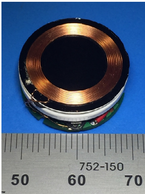
PCBA Stackup Bottom View
