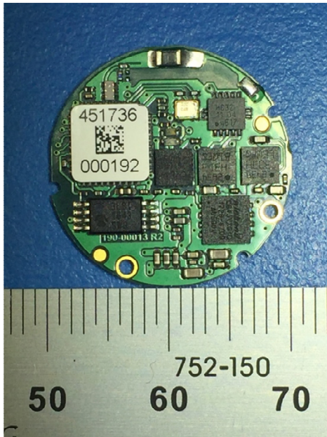
PCBA Top View
