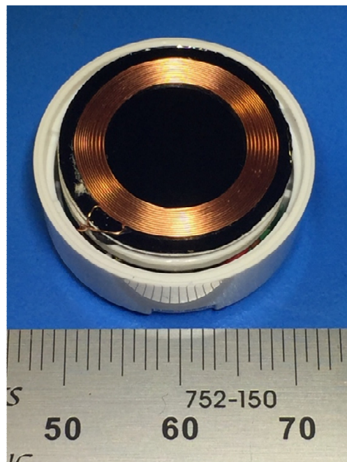
PCBA Stackup in Top Enclosure
