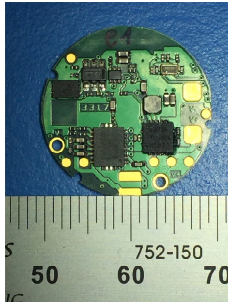
PCBA Bottom View
