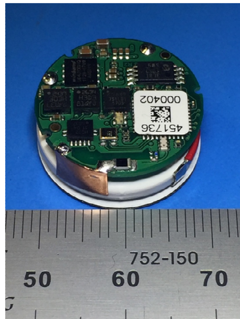
PCBA Stackup Antenna view
