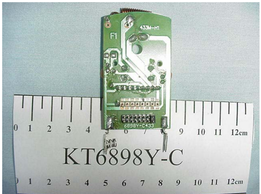
FIGURE 2 WIRELESS DOOR CHIME (M/N: KT6898Y-C) MAIN BOARD (SOLDERED SIDE)
