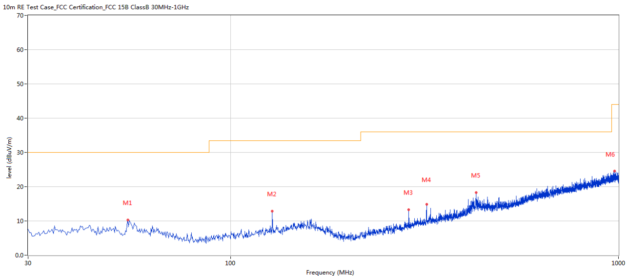
30 MHz to 1 GHz, ANT H
