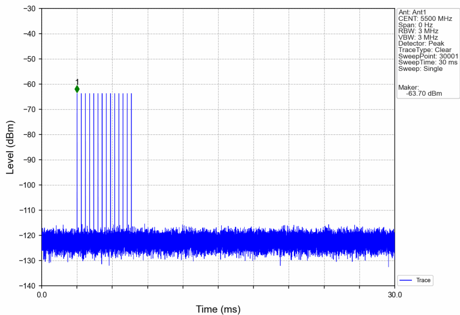
Signal Calibration 802.11a 2C 5500MHz RadarType5 Trial0
