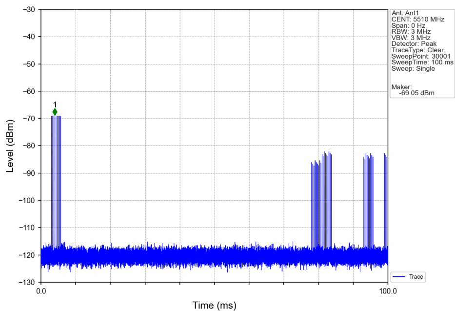
Signal Calibration 802.11n(HT40) 2C 5510MHz RadarType6 Trial0
