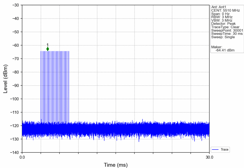
Signal Calibration 802.11n(HT40) 2C 5510MHz RadarType2 Trial0
