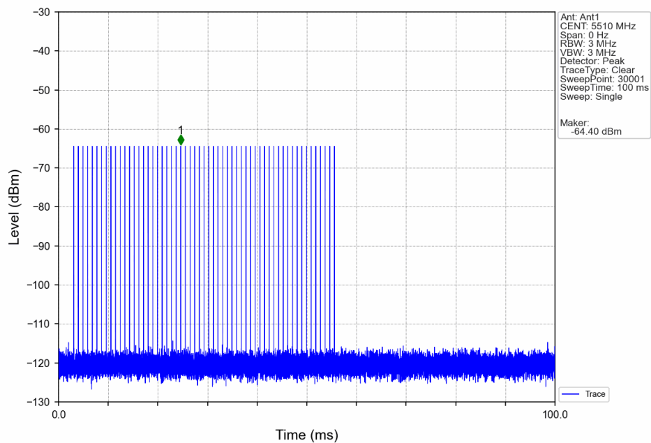
Signal Calibration 802.11n(HT40) 2C 5510MHz RadarType2 Trial0
