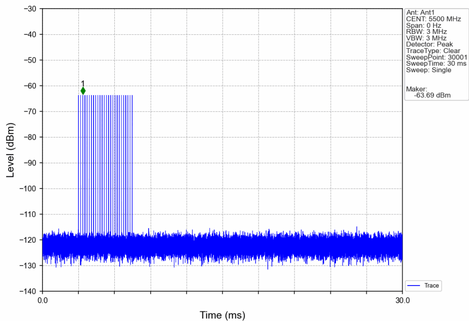
Signal Calibration 802.11a 2C 5500MHz RadarType3 Trial0
