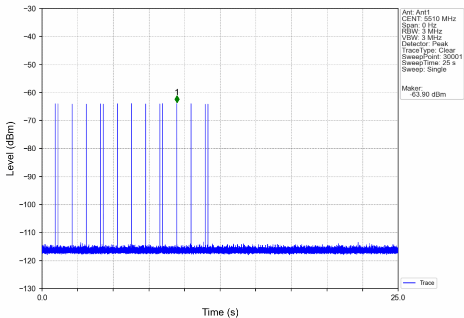
Signal Calibration 802.11n(HT40) 2C 5510MHz RadarType6 Trial0
