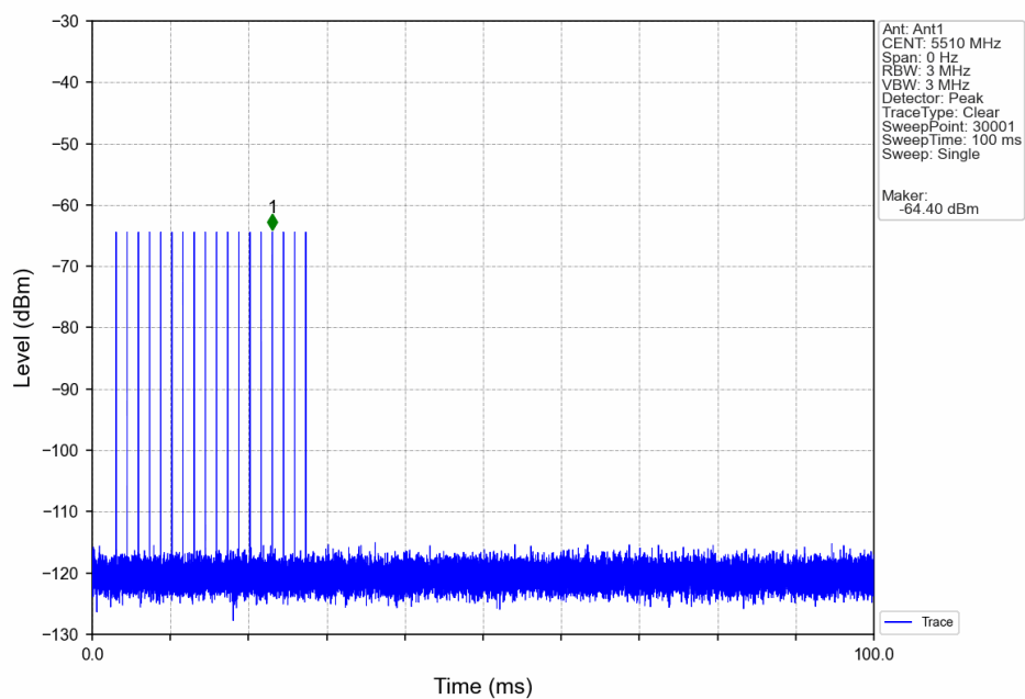
Signal Calibration 802.11n(HT40) 2C 5510MHz RadarType0 Trial0
