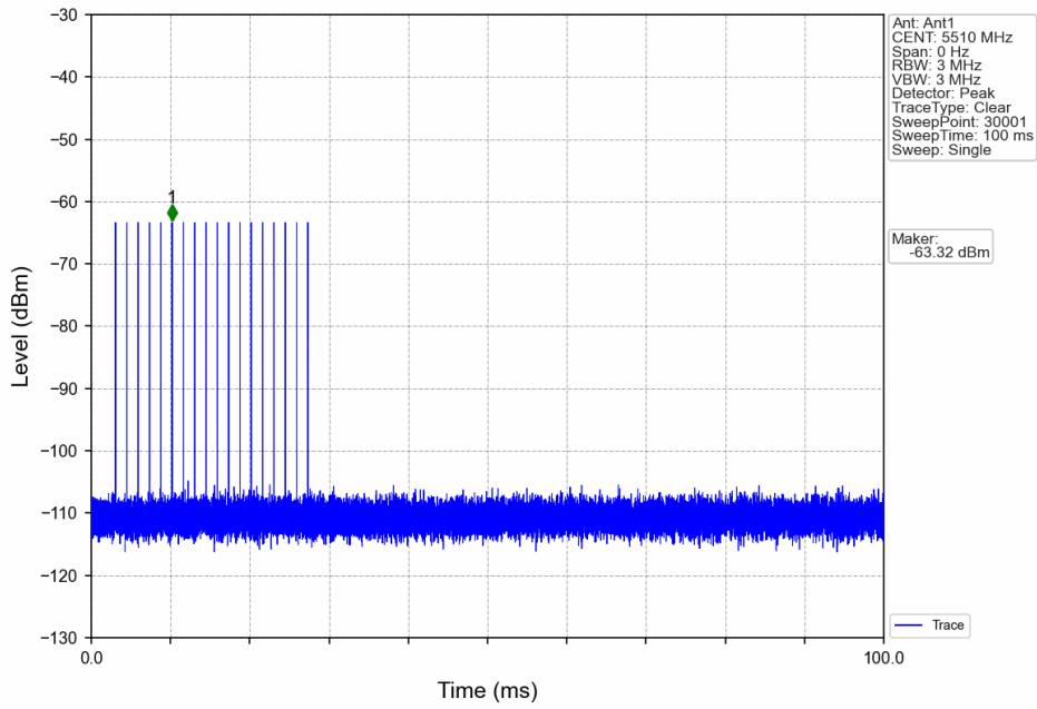
Signal Calibration_802.11n(HT40)_2C_5510MHz_RadarType0
