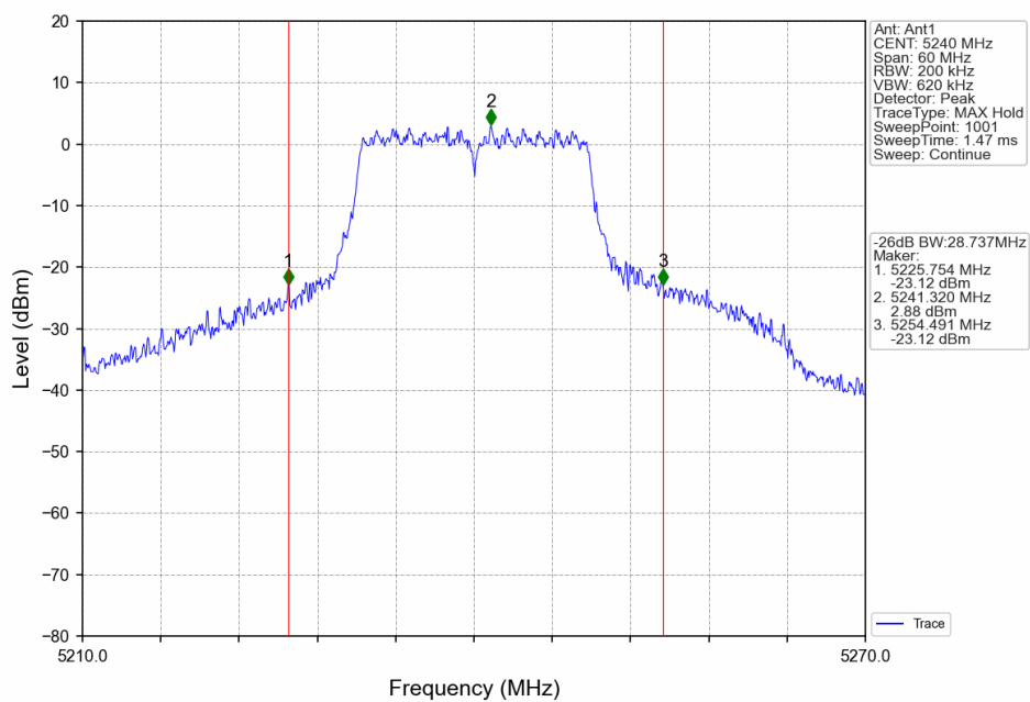
802.11n(HT20)_HCH_5240MHz_Ant1_NTN
