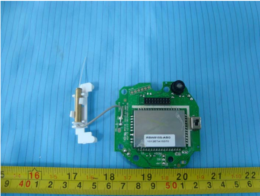
EUT – Main Board with Antenna View
