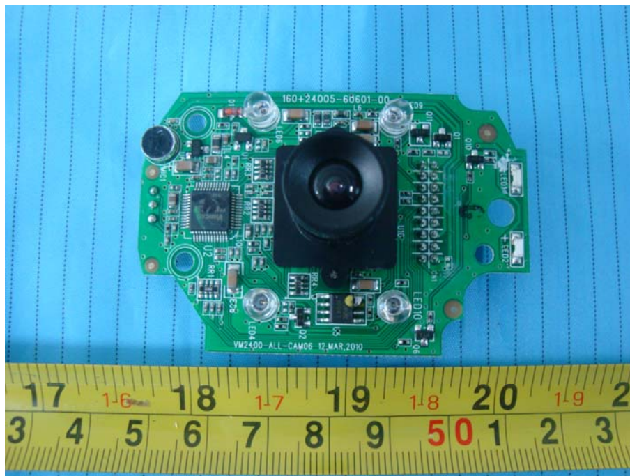
EUT – Main Board with Camera Lens View
