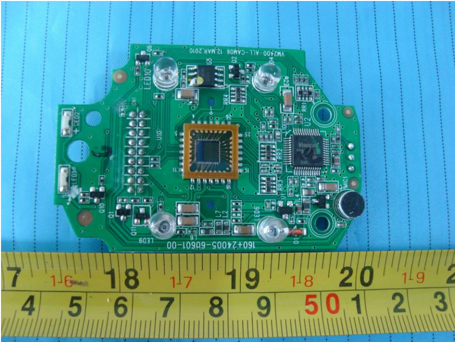
EUT – Main Board without Camera Lens View
