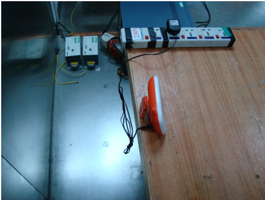
AC Line Conducted Emissions - Side View (Adapter Mode)
