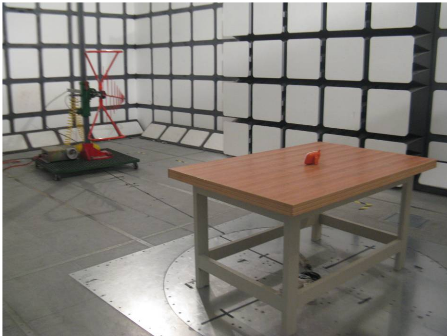
Below 1 GHz: Radiated Emissions - Rear View (Battery Mode)
