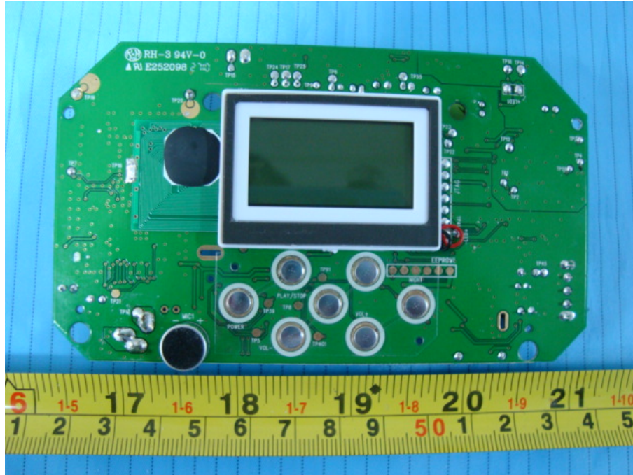
EUT – Main Board with LCD Screen Bottom View 1
