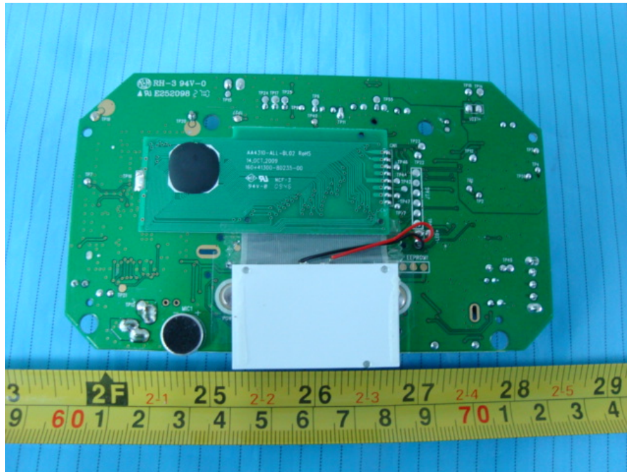
EUT – Main Board with LCD Screen Bottom View 2
