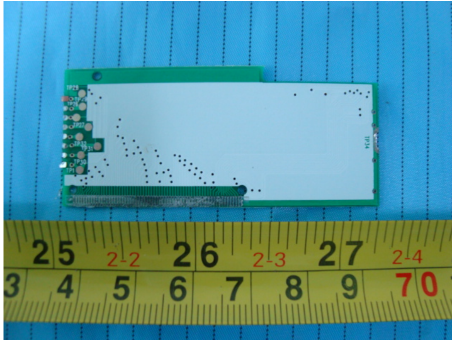
EUT – Other Board Bottom View
