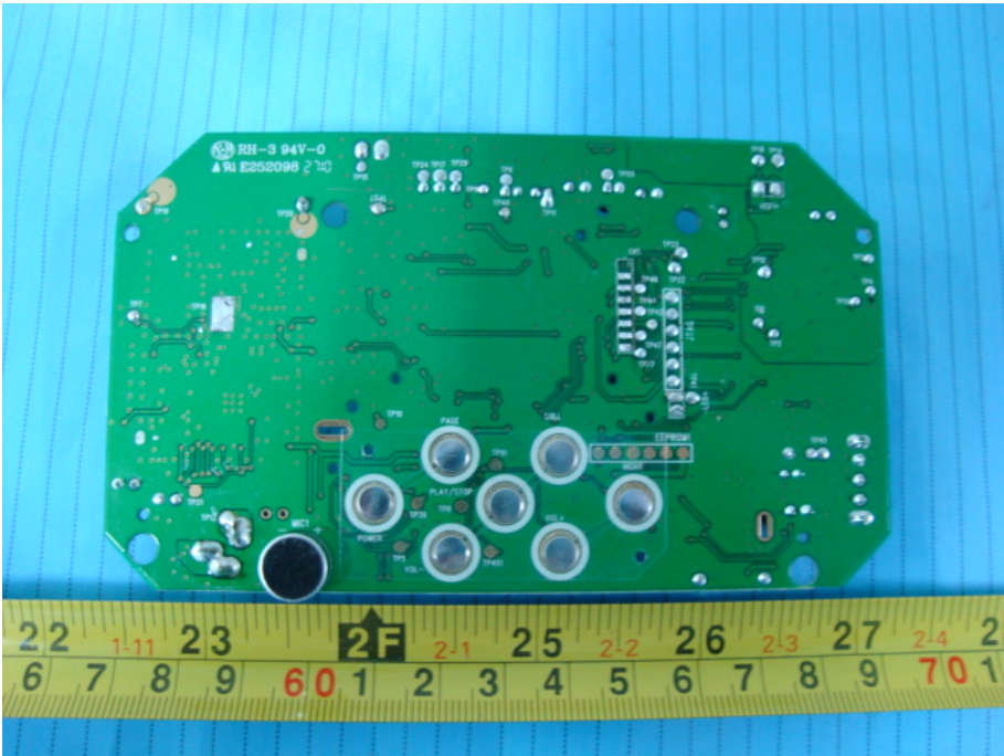
EUT – Main Board Shielded off BottomView
