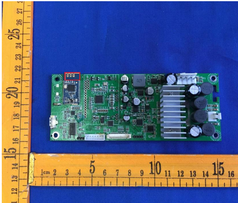
Antenna View
