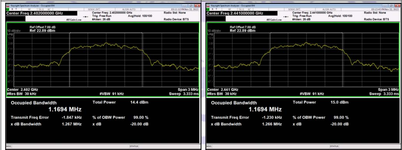
8DPSK_3-DH1_Channel 0
