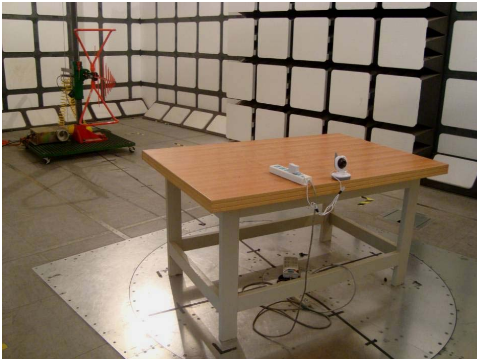
Below 1 GHz: Radiated Emissions - Rear View (Adapter Mode)
