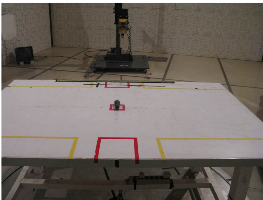
Radiated emission
