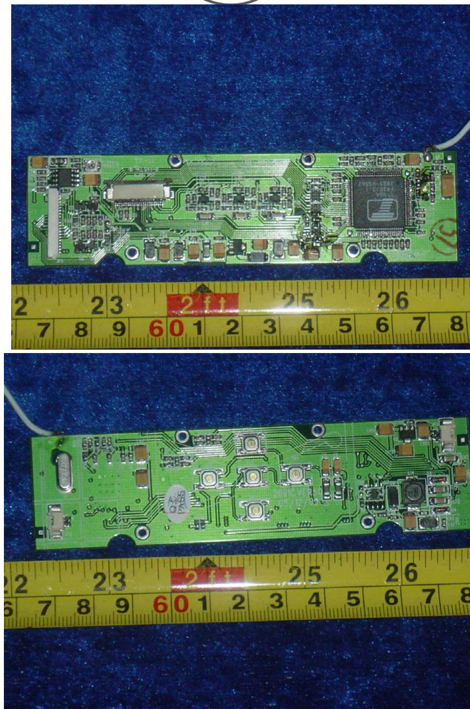
Interior View
