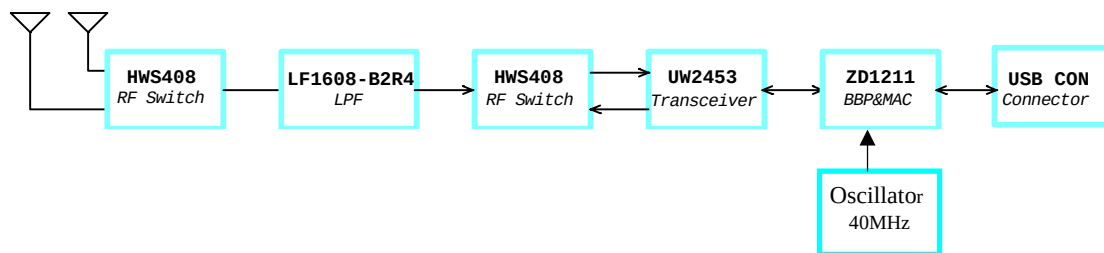
The WiFi Module Diagram
