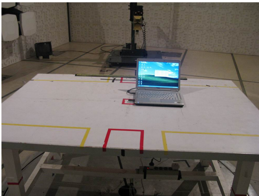
Radiated emission
