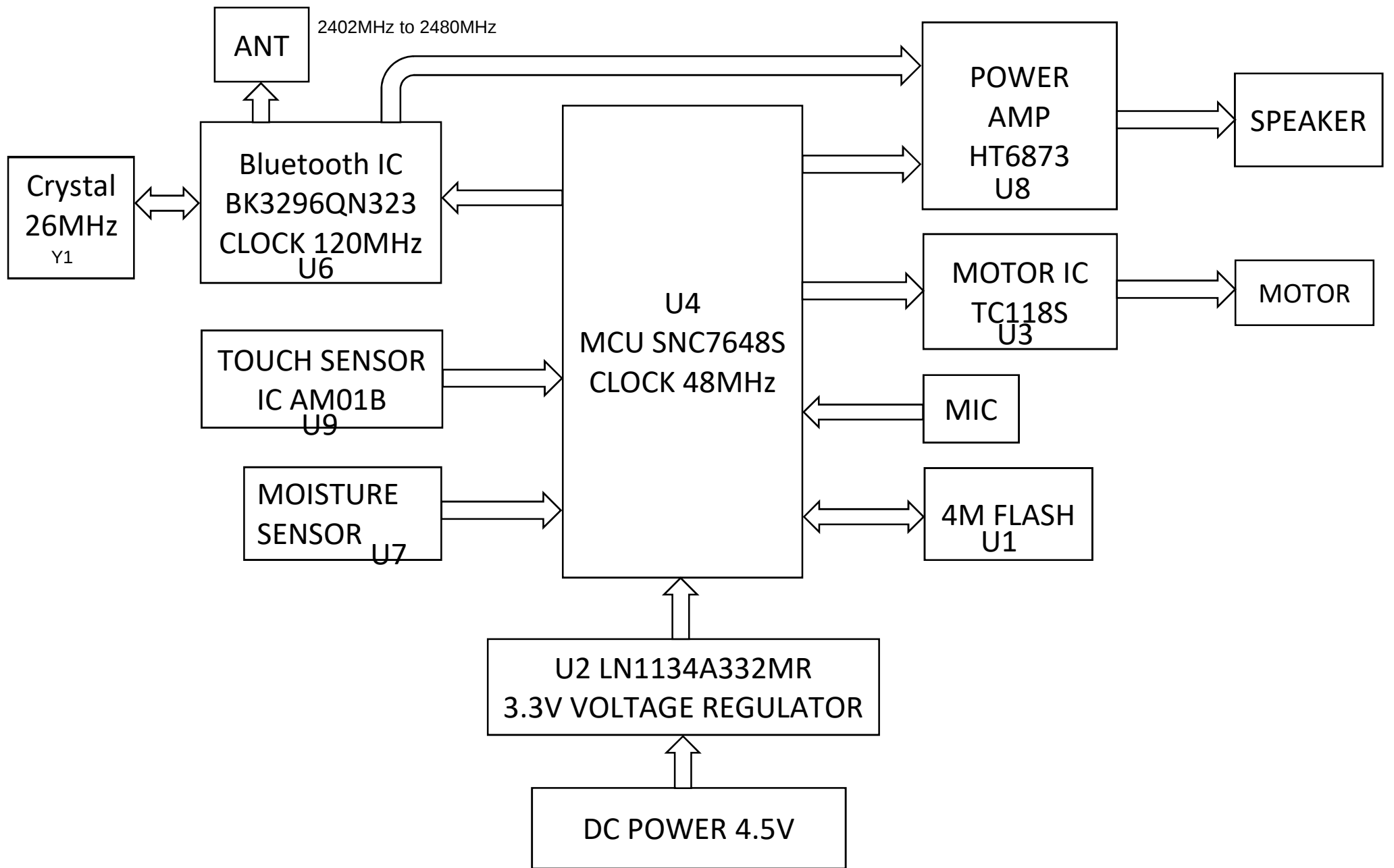
Block Diagram
