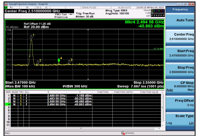
Right bandedge
