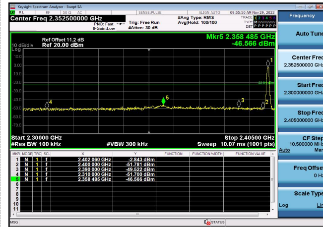
Left bandedge
