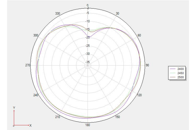
The Theta 90 2D chart
