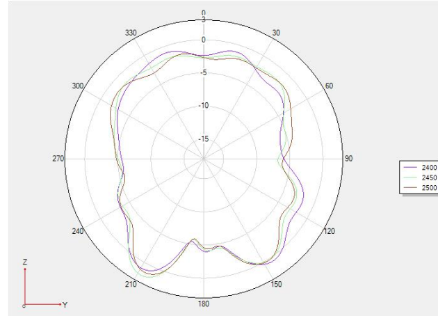
Phi 90 2D chart
