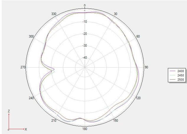
Phi 0 2D graph
