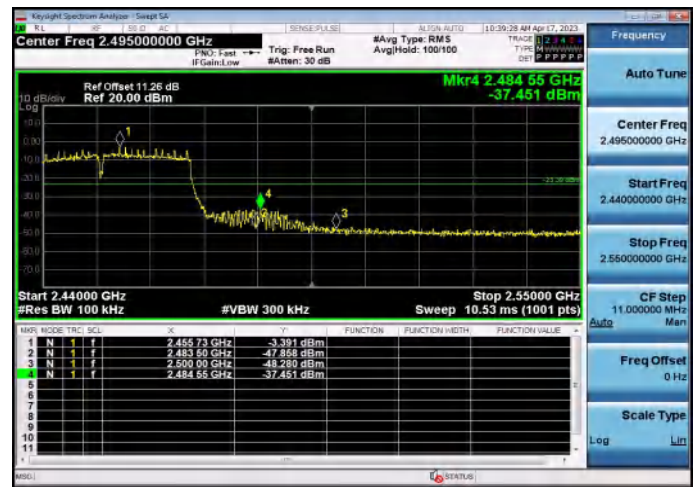
Right bandedge
