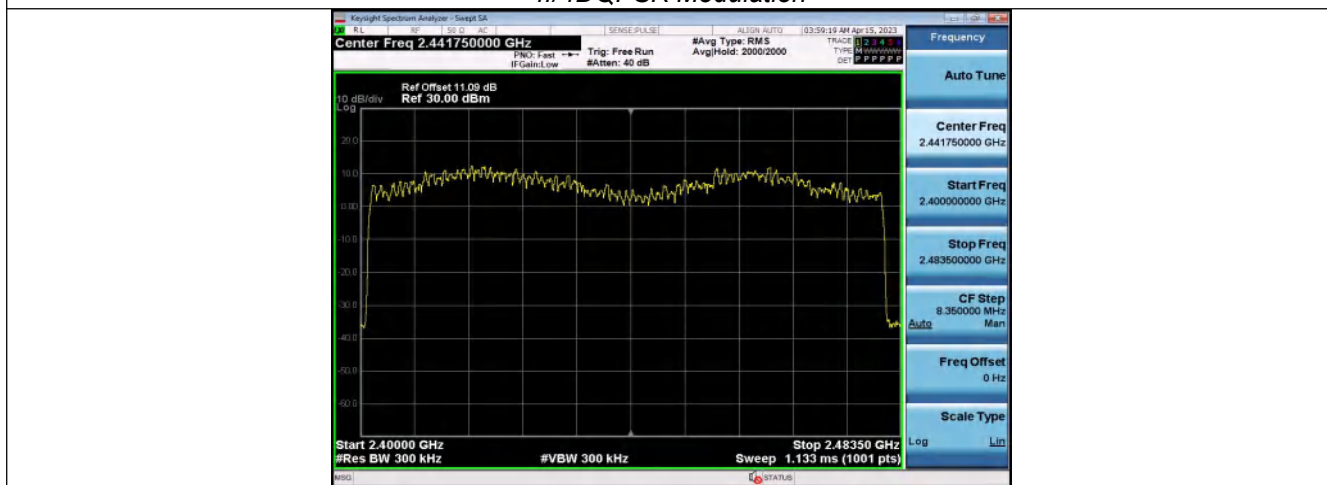
8DPSK Modulation
