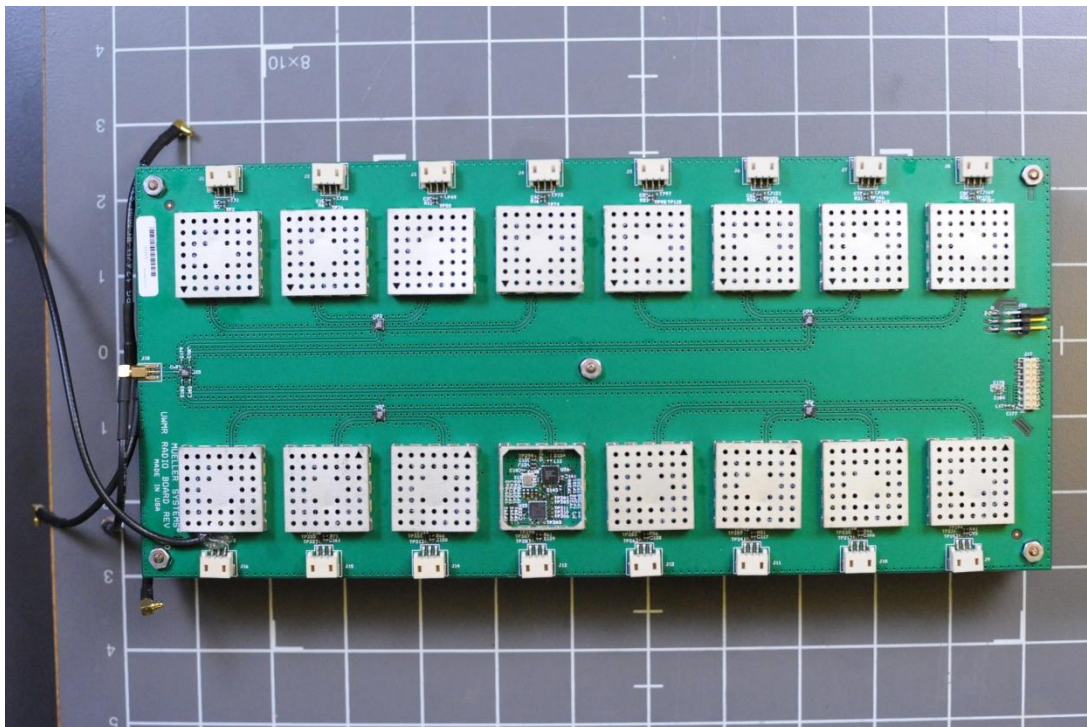
4 Internal Photo, Radio Board, Top
