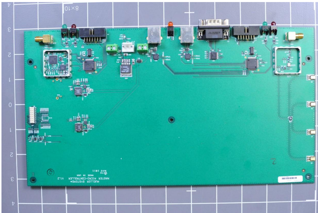
2 Internal Photo, MCU Board Top
