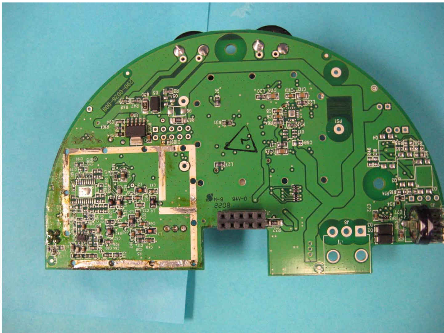
SM6-UGM-L Internal photo of the bottom of the module
