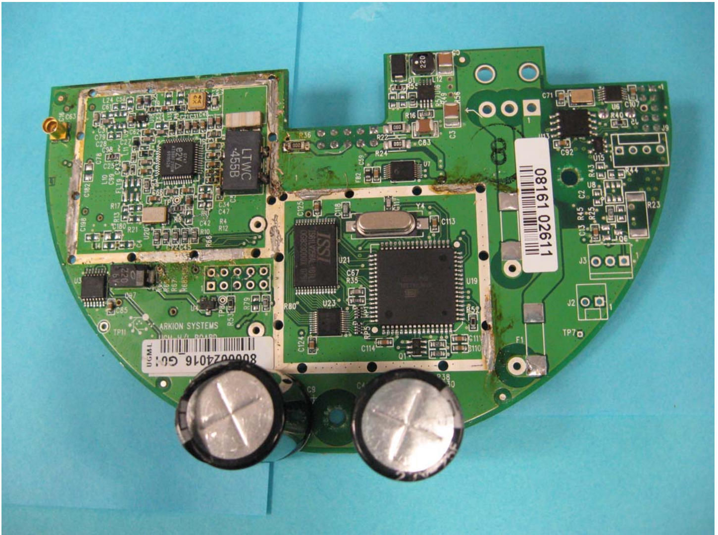
SM6-UGM-L Internal photo of the top of the module
