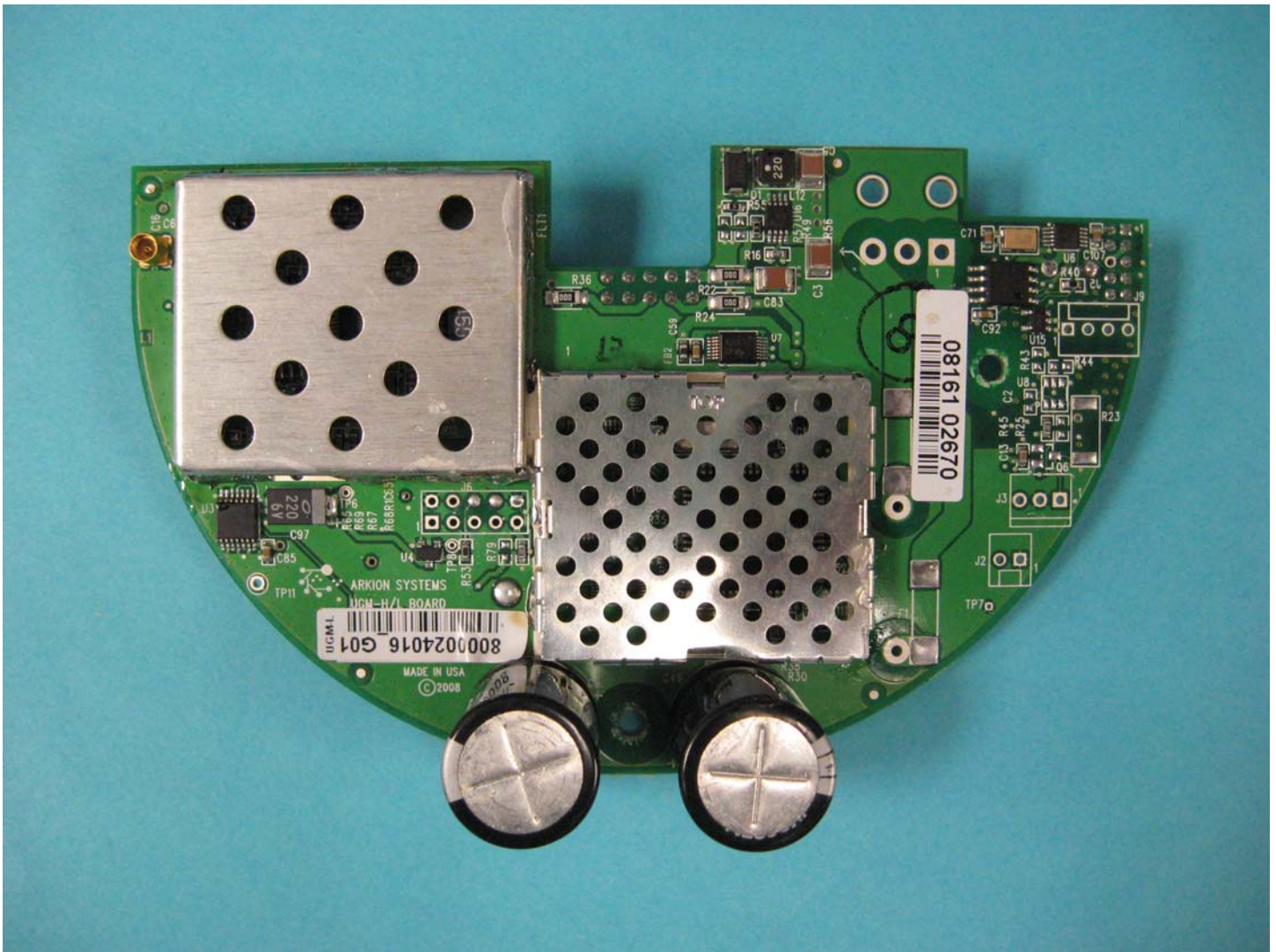
SM6-UGM-L external photos, top of the module
