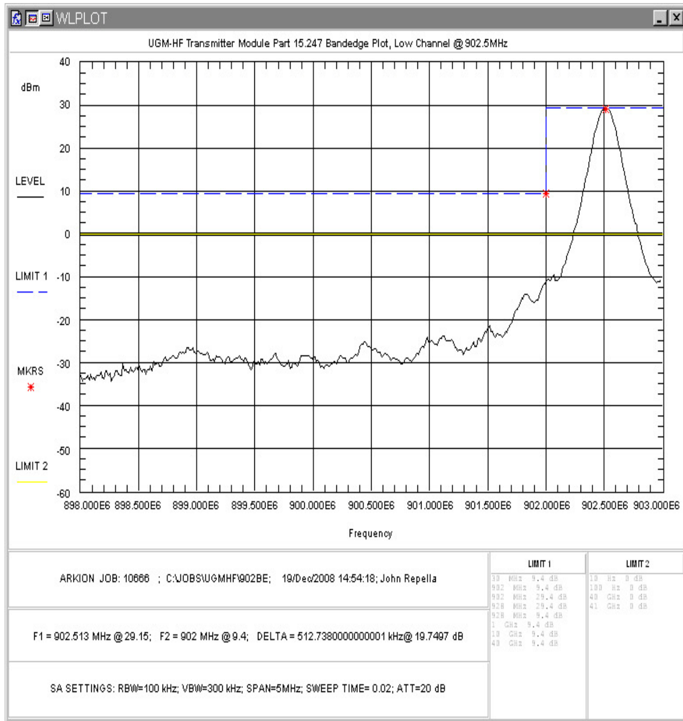
Figure 5-11. Lower Band Edge Plot, Low Channel
