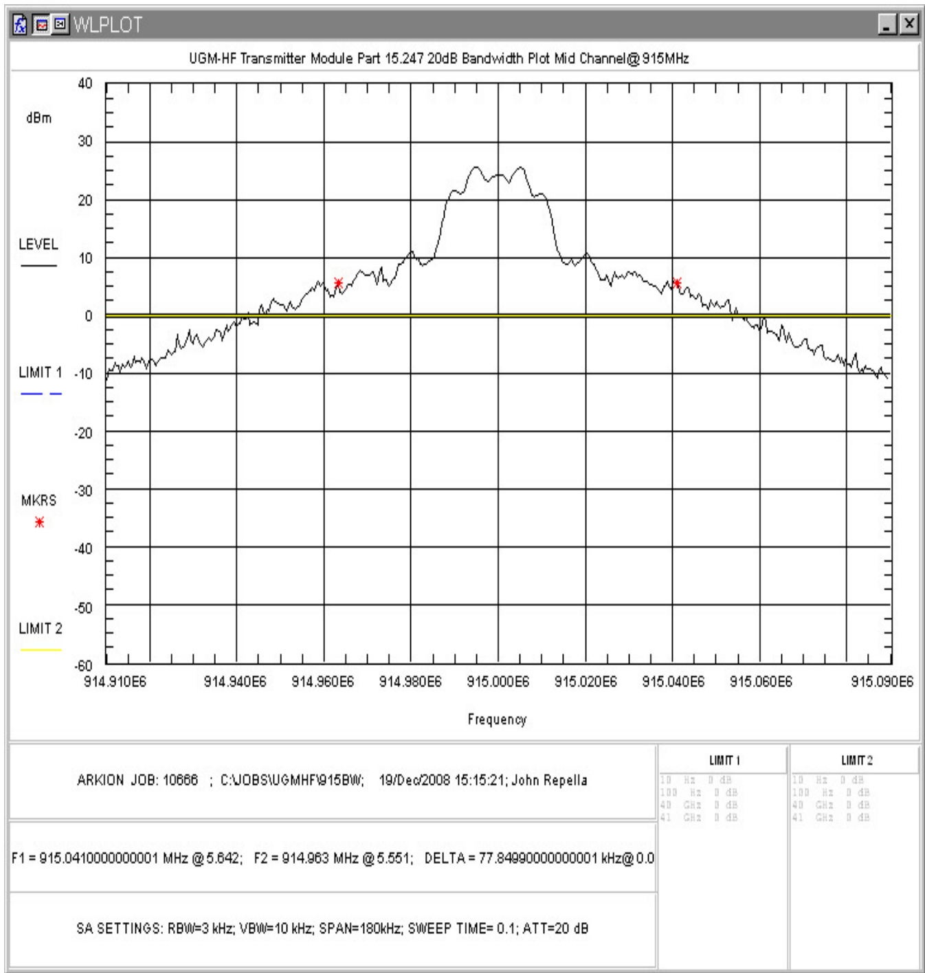
Figure 5-7. Occupied Bandwidth, Mid Channel
