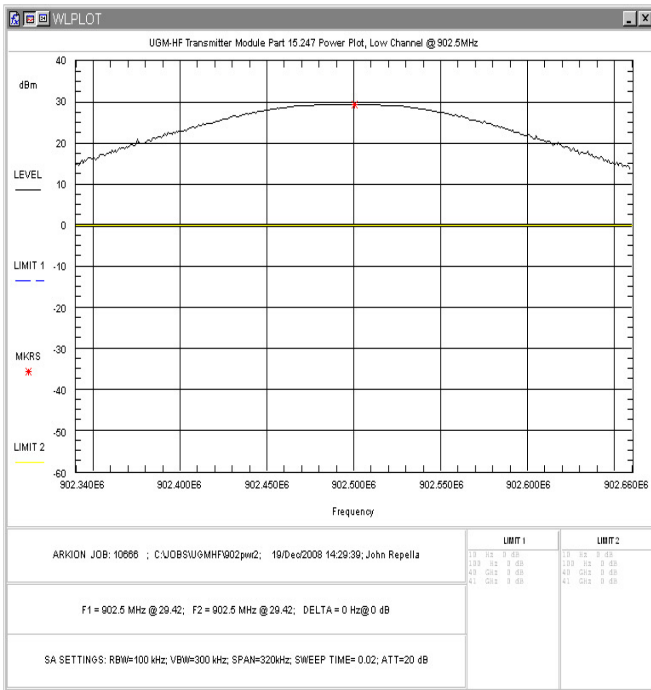
Figure 5-3. RF Peak Power, Low Channel
