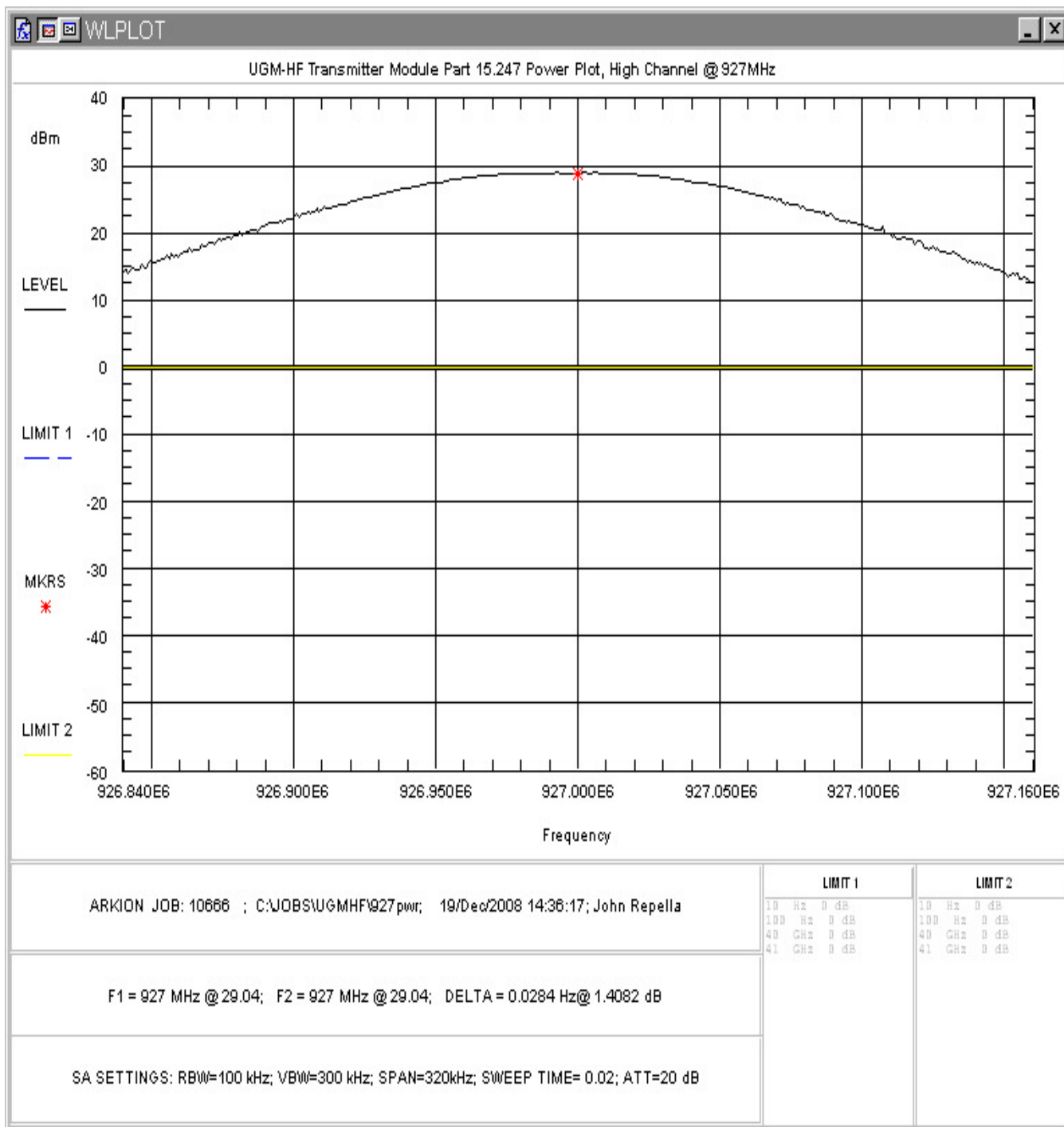
Figure 5-5. RF Peak Power, High Channel
