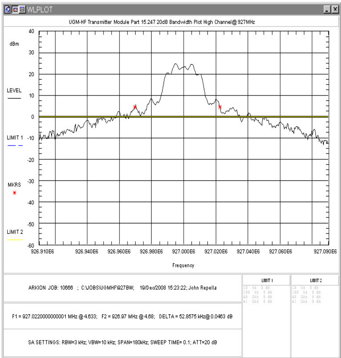
Figure 5-8. Occupied Bandwidth, High Channel
