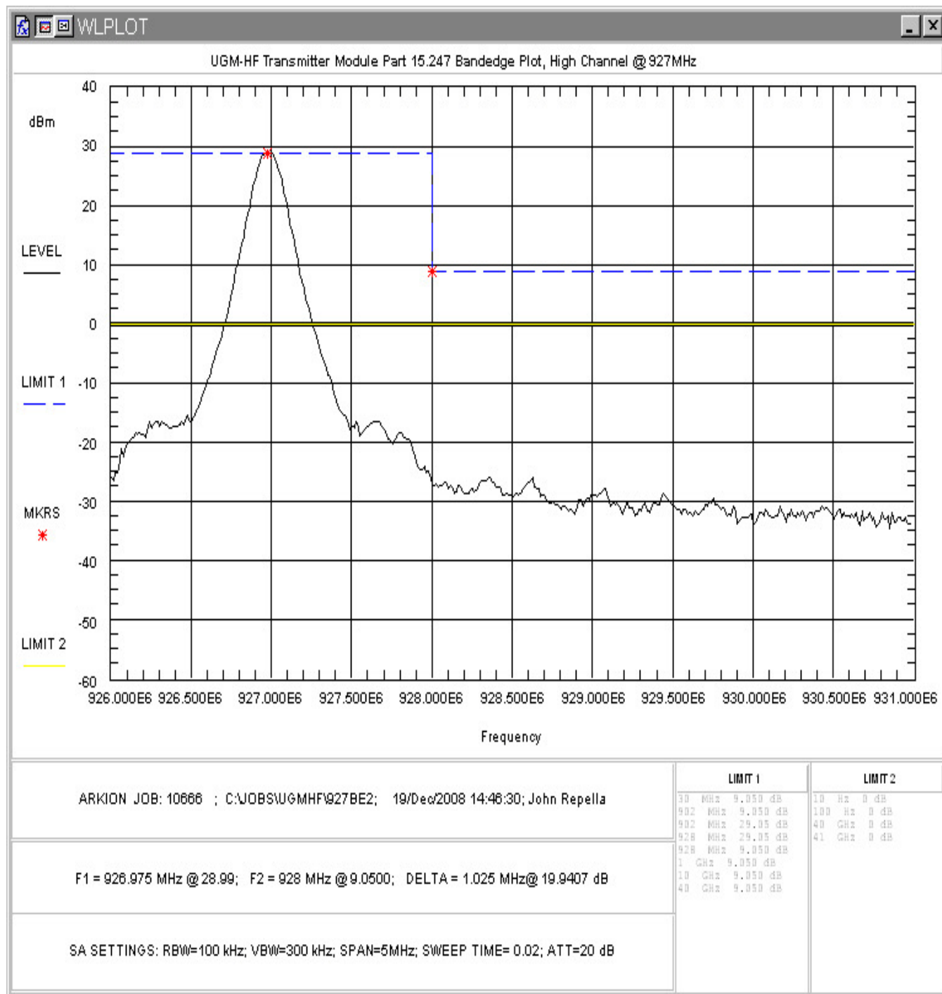
Figure 5-12. Upper Band Edge Plot, High Channel
