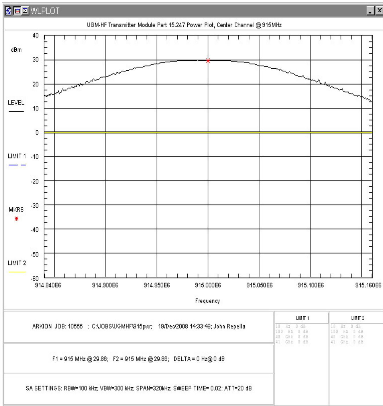
Figure 5-4. RF Peak Power, Mid Channel
