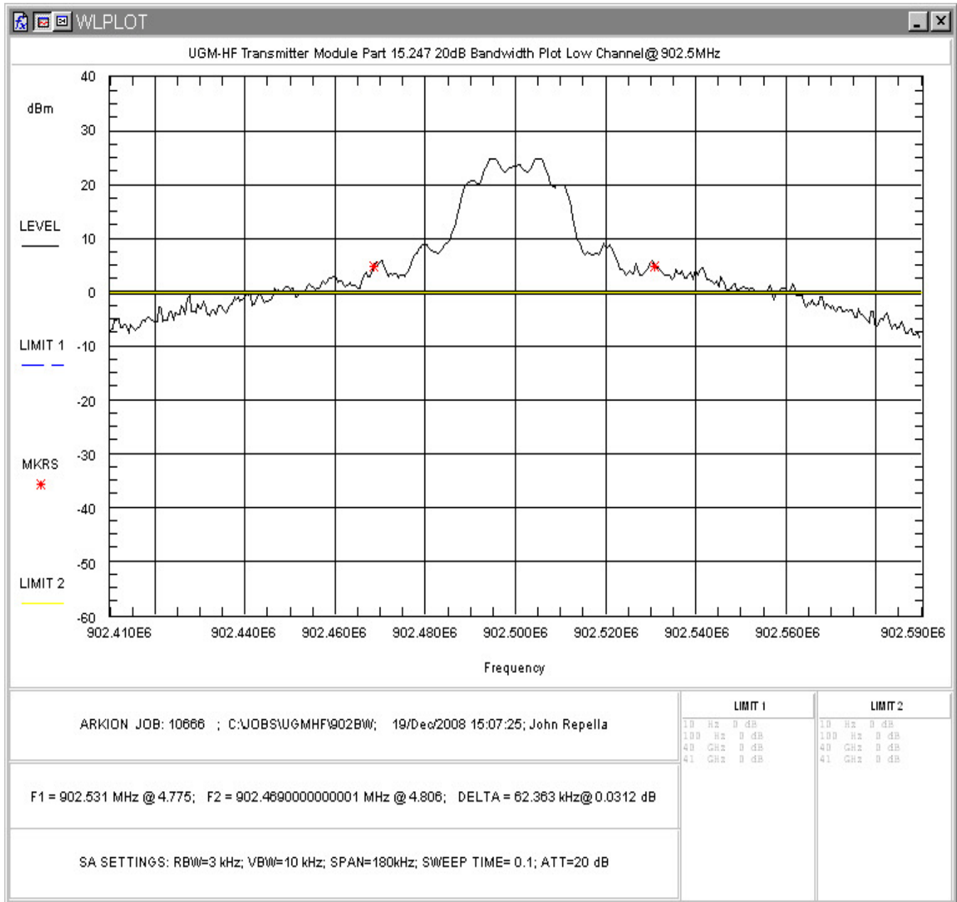
Figure 5-6. Occupied Bandwidth, Low Channel
