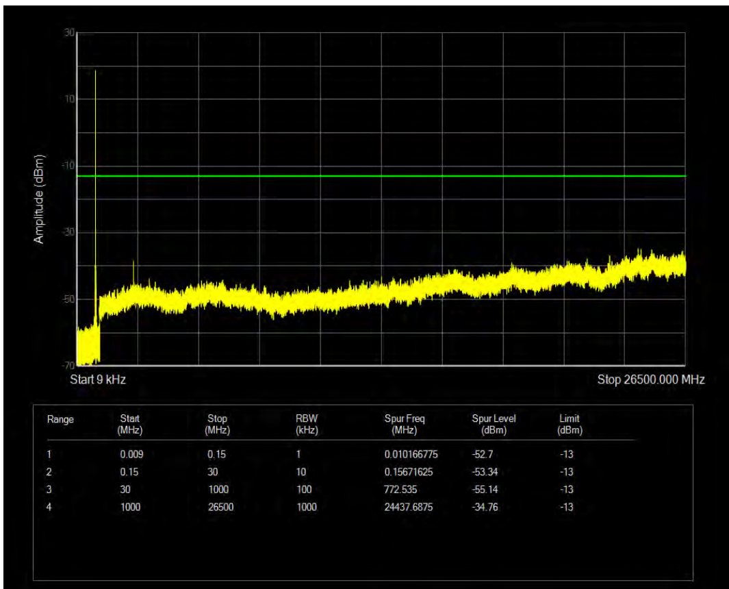
Band5 16QAM BW=10MHz Channel=20450 RB Size=6 Position=#0 NB Index=0
