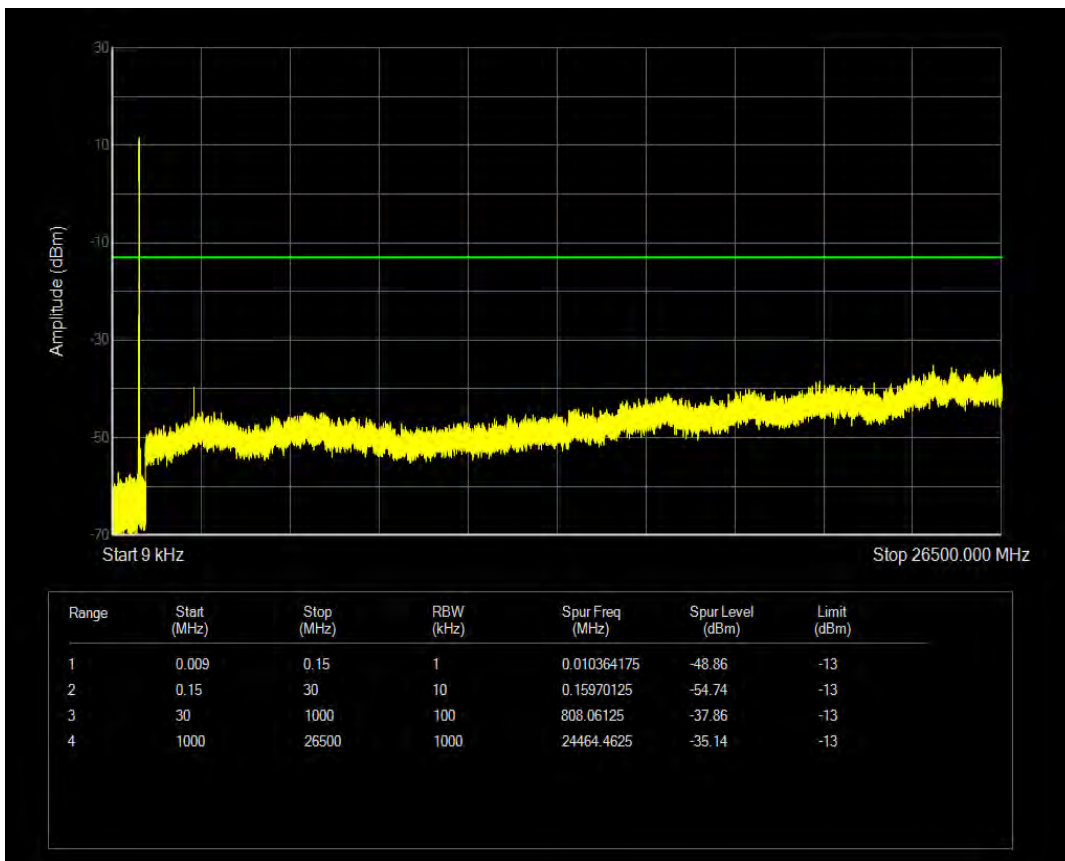
Band26(814-824) 16QAM BW=1.4MHz Channel=26783 RB Size=1 Position=#0 NB Index=0
