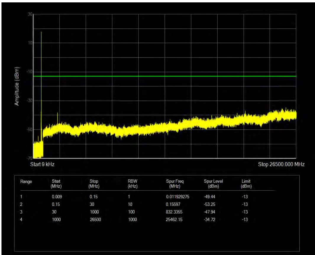
Band26(814-824) 16QAM BW=1.4MHz Channel=26783 RB Size=6 Position=#0 NB Index=0
