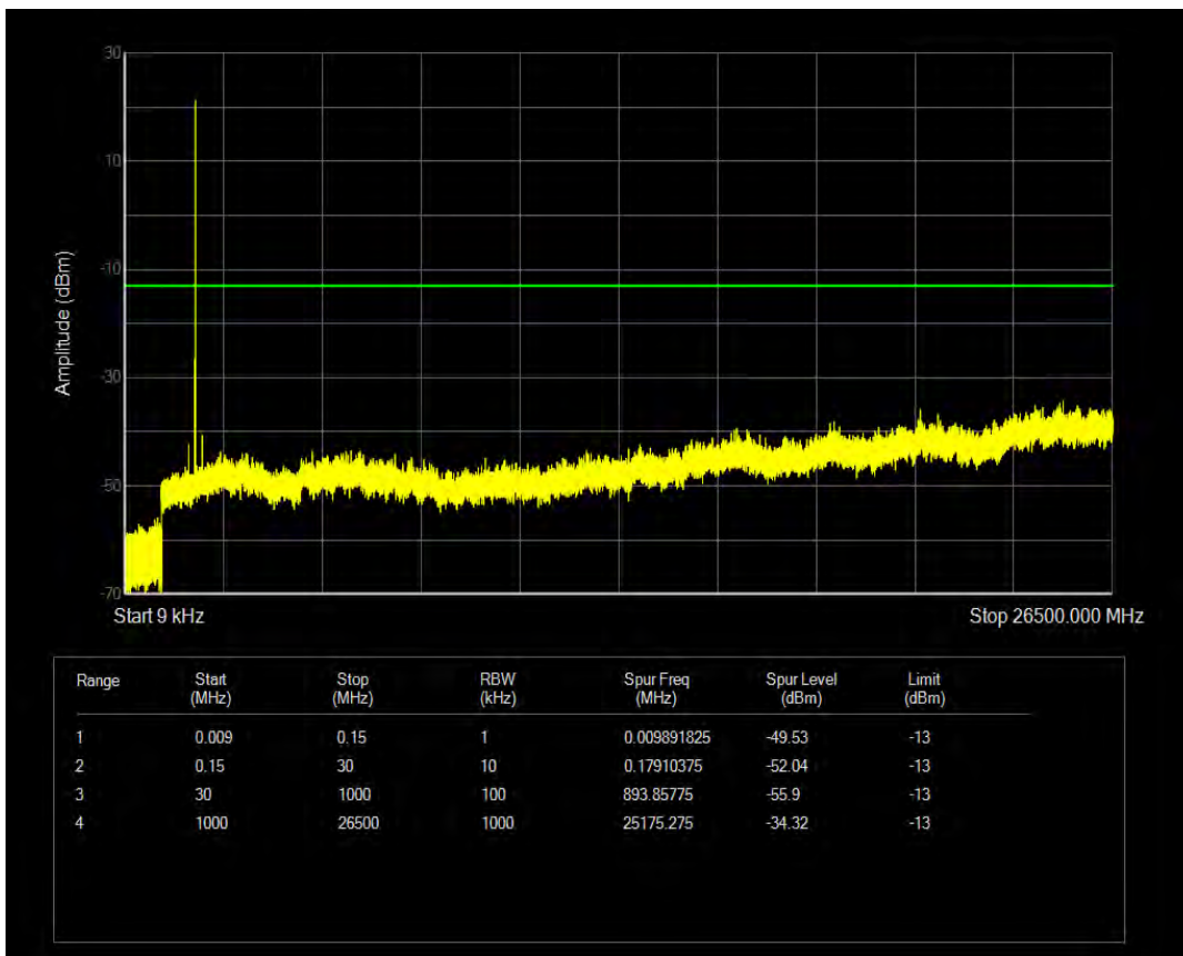
Band2 16QAM BW=1.4MHz Channel=19193 RB Size=6 Position=#0 NB Index=0
