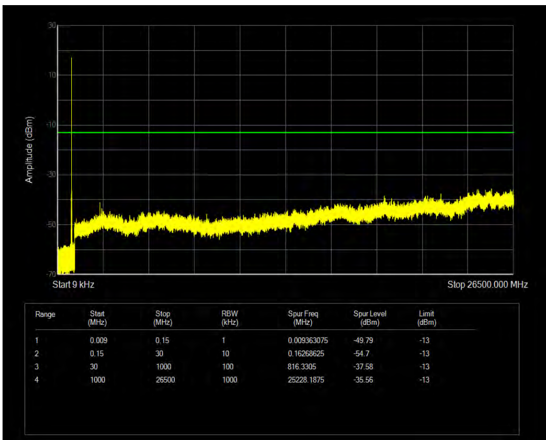
Band26(824-849) 16QAM BW=1.4MHz Channel=26797 RB Size=6 Position=#0 NB Index=0
