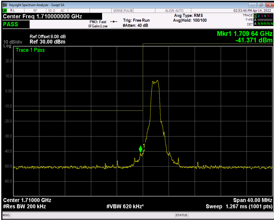
Band66 16QAM BW=20MHz Channel=132572 RB Size=1 Position=#Max NB Index=15
