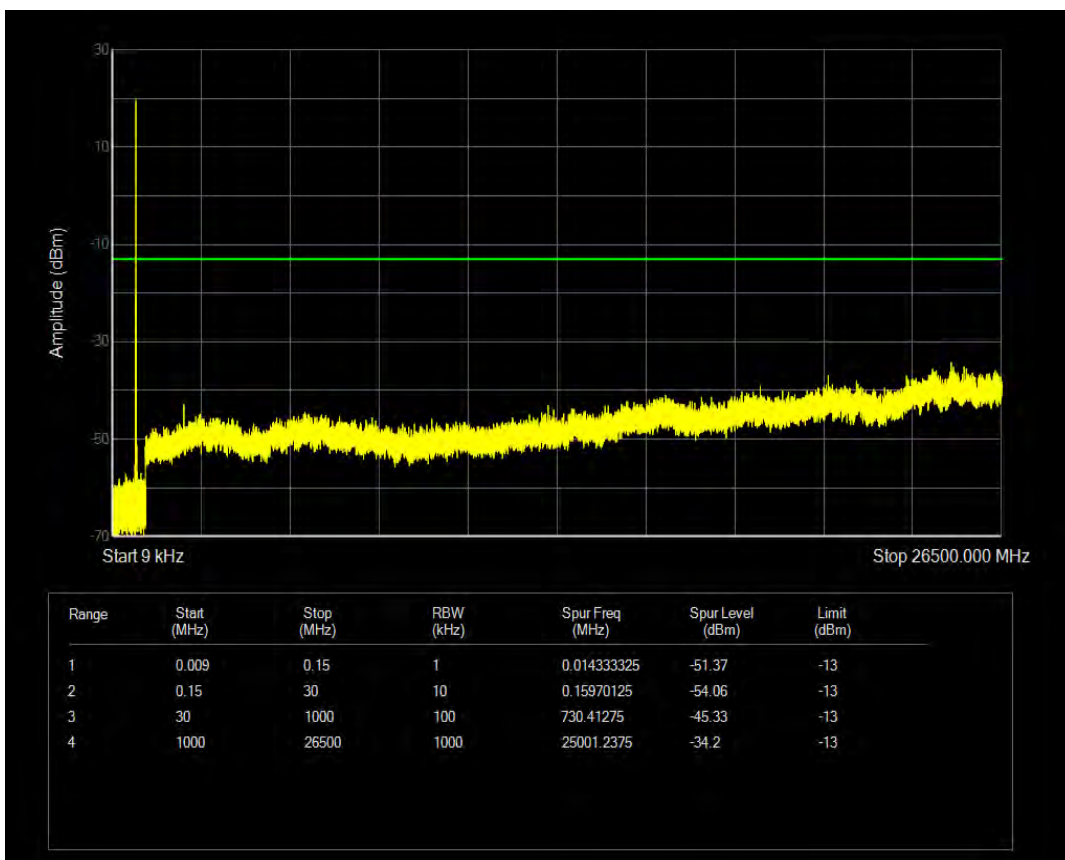
Band12 16QAM BW=1.4MHz Channel=23173 RB Size=6 Position=#0 NB Index=0
