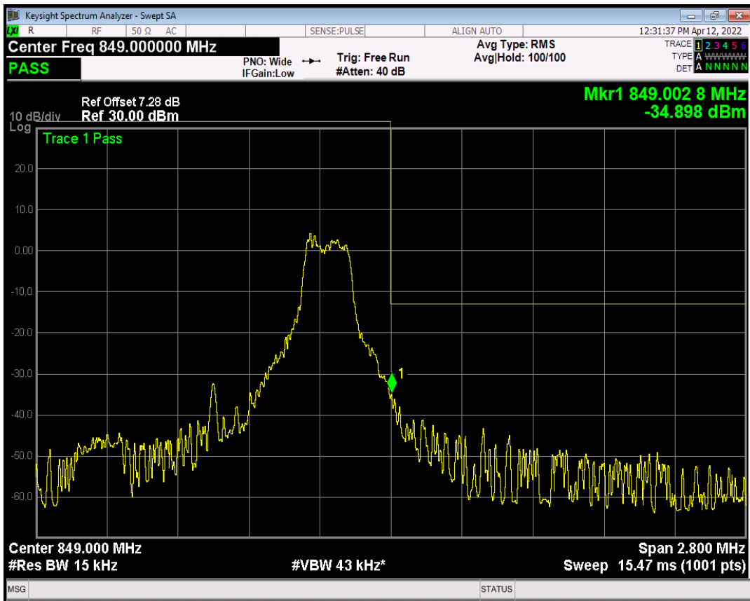
Band5 QPSK BW=1.4MHz Channel=20643 RB Size=6 Position=#Max NB Index=0
