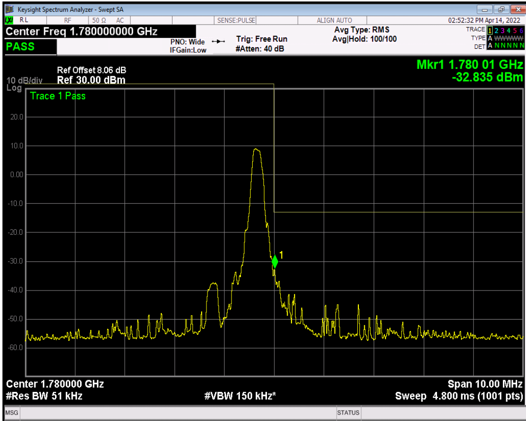
Band66 16QAM BW=5MHz Channel=132647 RB Size=6 Position=#Max NB Index=3
