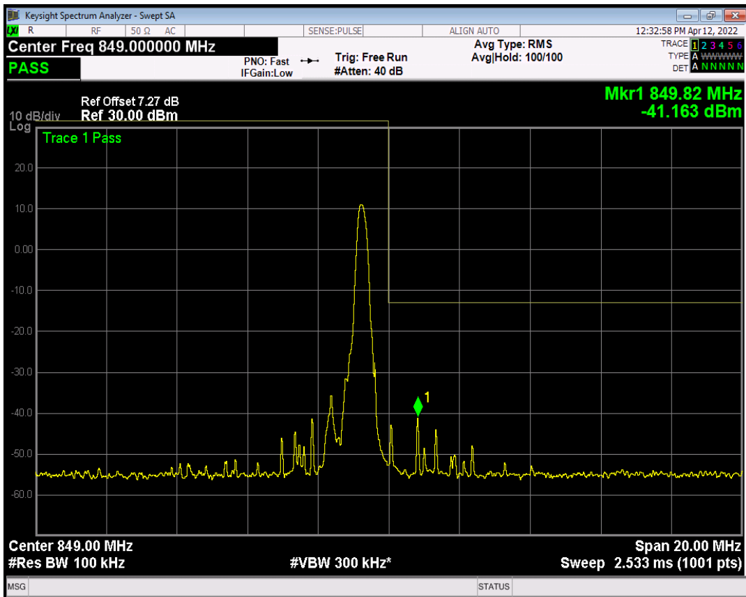
Band5 QPSK BW=10MHz Channel=20600 RB Size=4 Position=#Max NB Index=7
