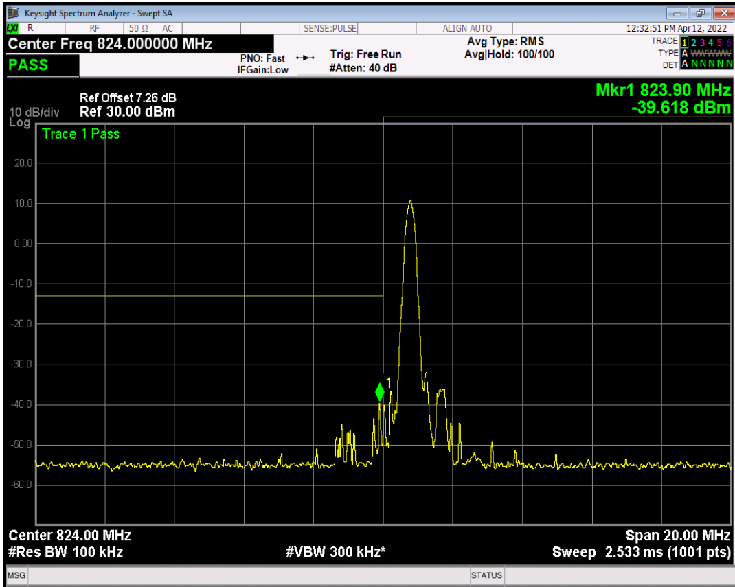
Band5 16QAM BW=10MHz Channel=20450 RB Size=4 Position=#0 NB Index=0
