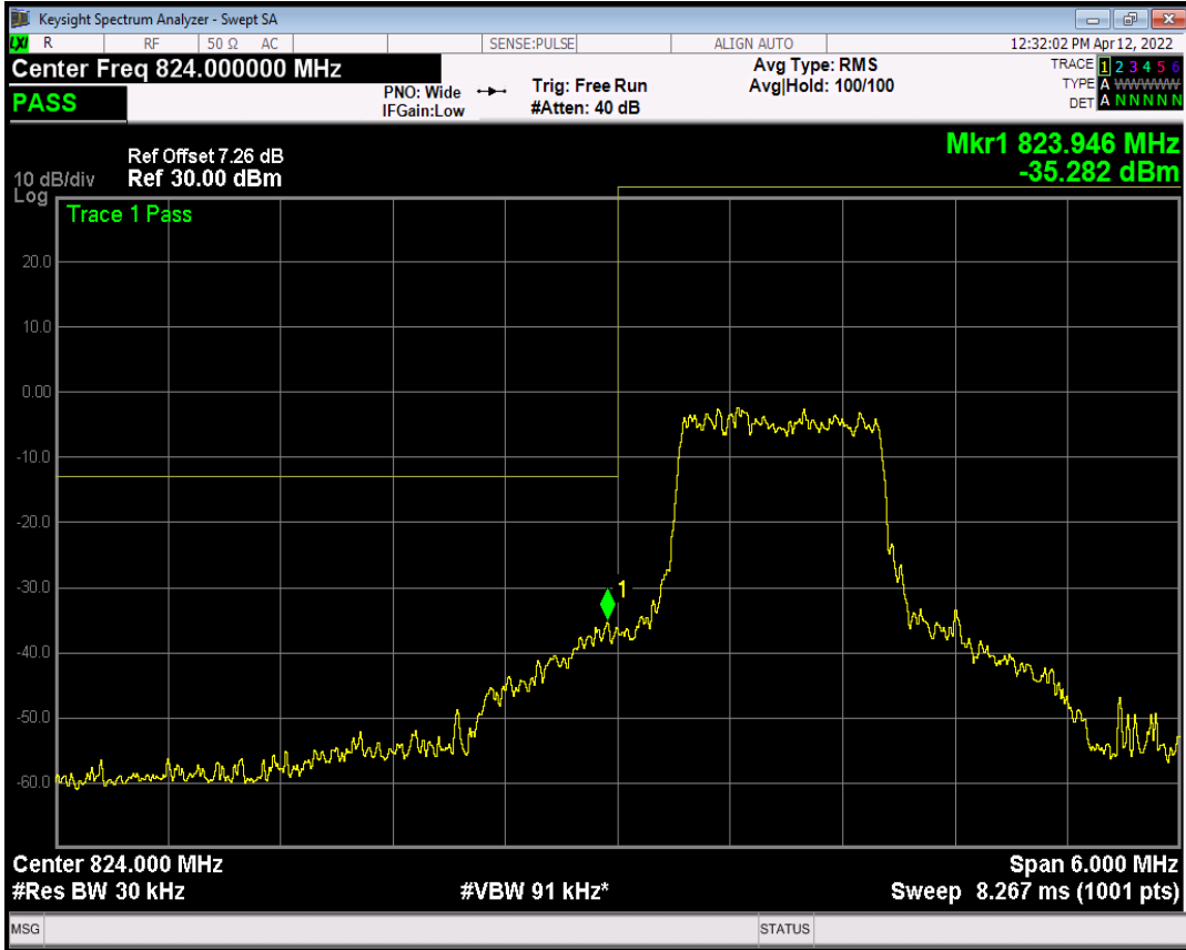
Band5 16QAM BW=3MHz Channel=20635 RB Size=1 Position=#Max NB Index=1
