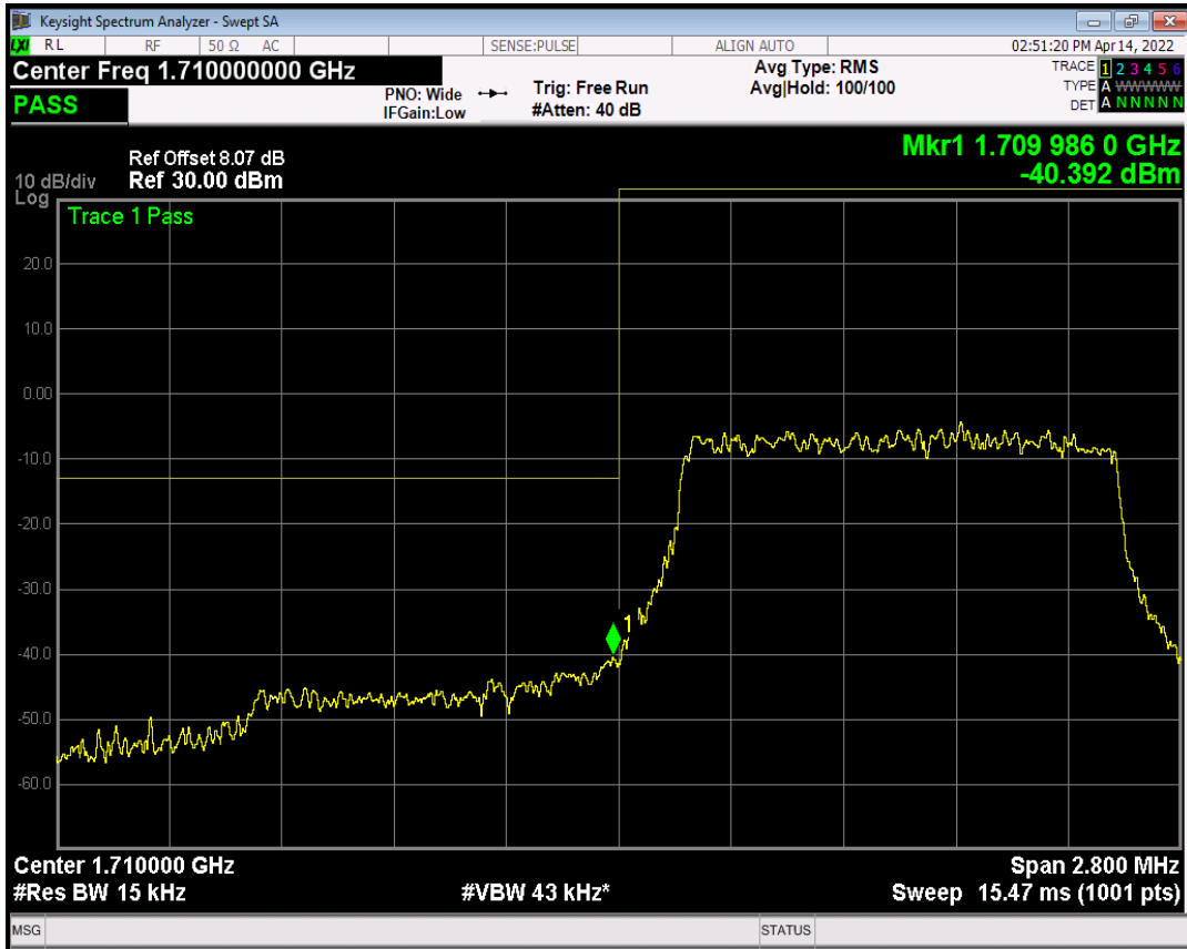
Band66 16QAM BW=1.4MHz Channel=132665 RB Size=1 Position=#Max NB Index=0
