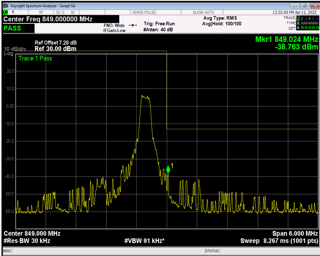
Band5 QPSK BW=3MHz Channel=20635 RB Size=6 Position=#Max NB Index=1
