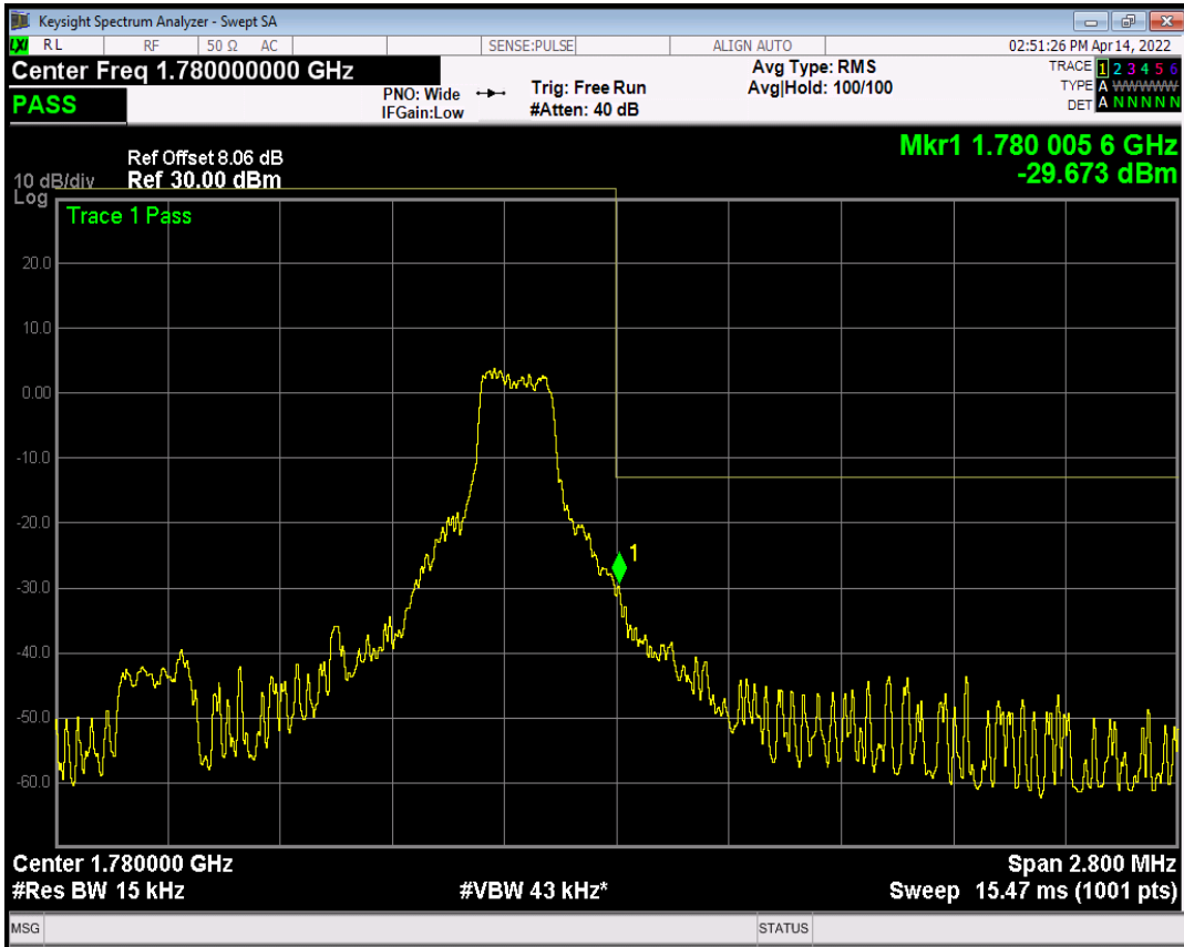
Band66 QPSK BW=1.4MHz Channel=132665 RB Size=6 Position=#Max NB Index=0
