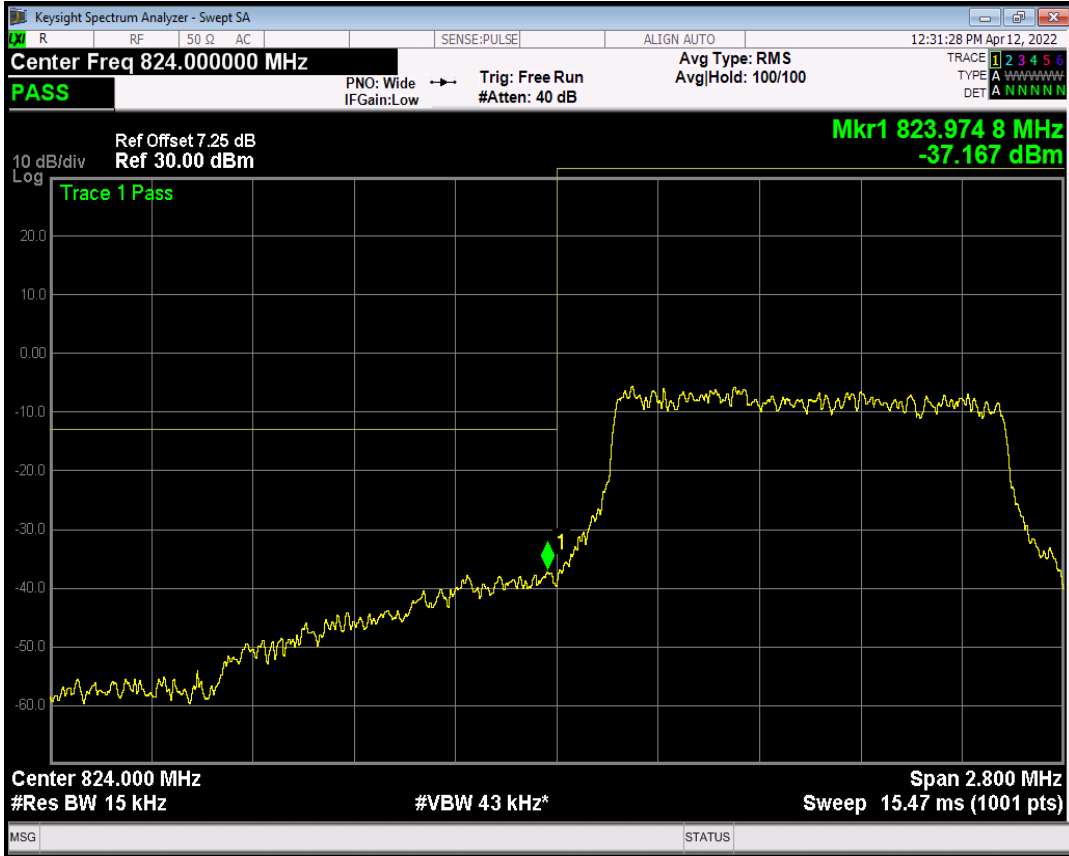
Band5 16QAM BW=1.4MHz Channel=20643 RB Size=1 Position=#Max NB Index=0
