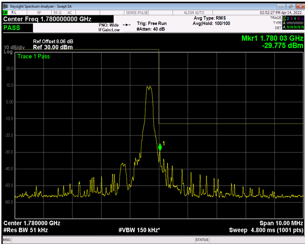
Band66 QPSK BW=5MHz Channel=132647 RB Size=6 Position=#Max NB Index=3
