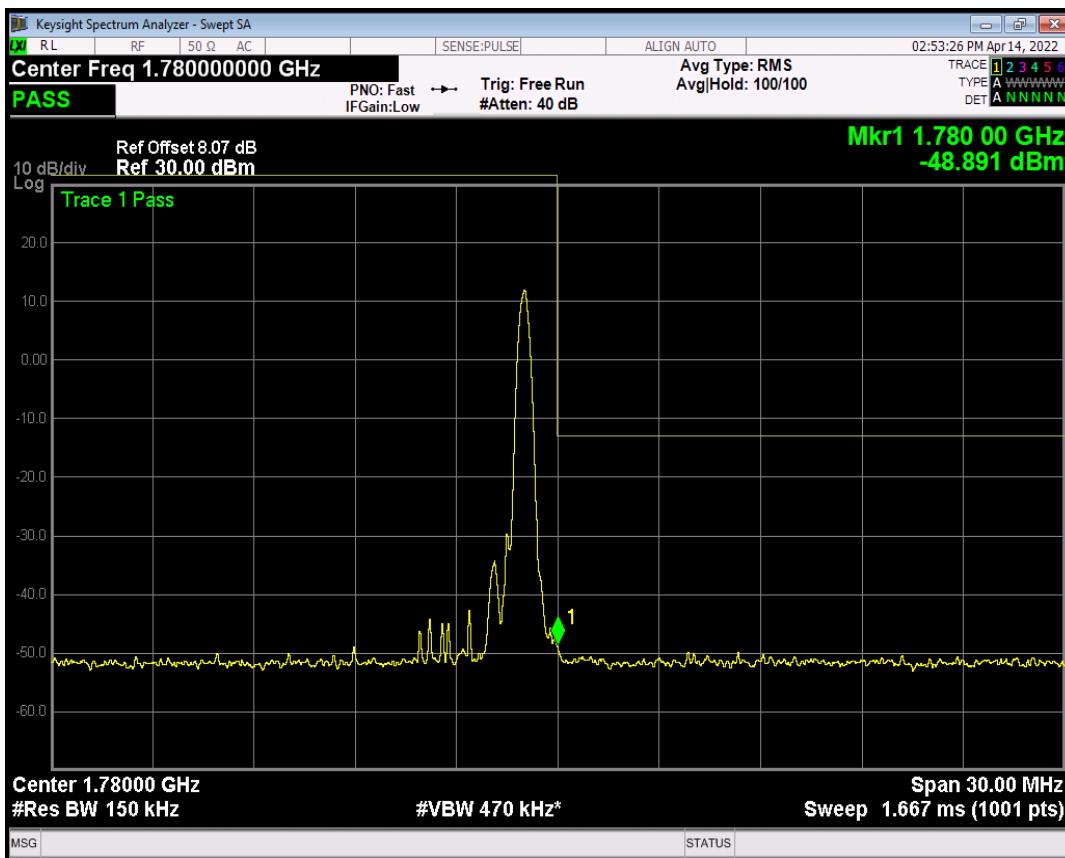
Band66 16QAM BW=15MHz Channel=132597 RB Size=6 Position=#Max NB Index=1
