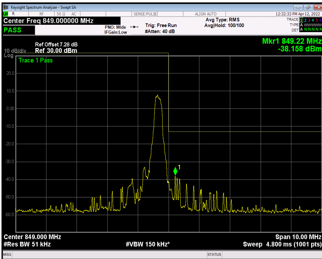
Band5 QPSK BW=5MHz Channel=20625 RB Size=6 Position=#Max NB Index=3
