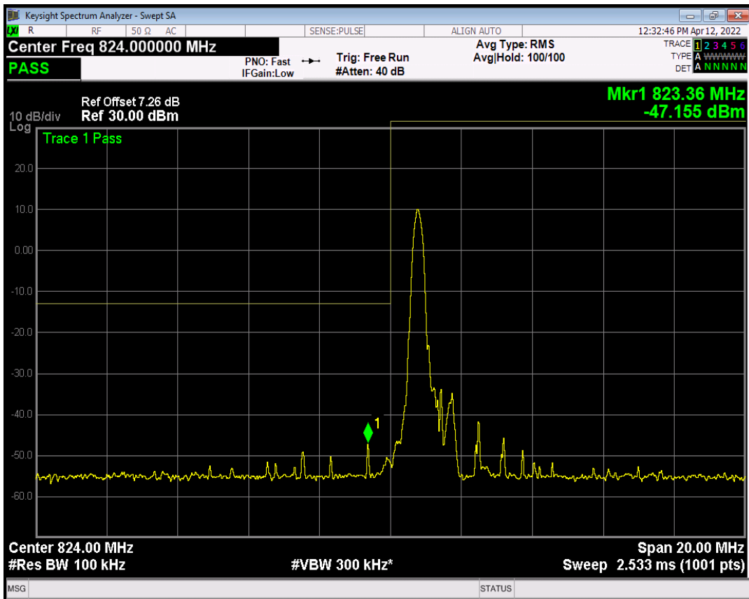
Band5 QPSK BW=10MHz Channel=20450 RB Size=4 Position=#0 NB Index=0
