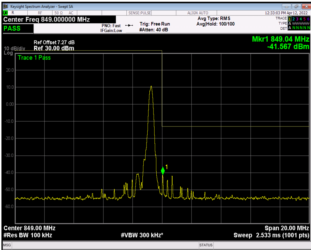
Band5 16QAM BW=10MHz Channel=20600 RB Size=4 Position=#Max NB Index=7
