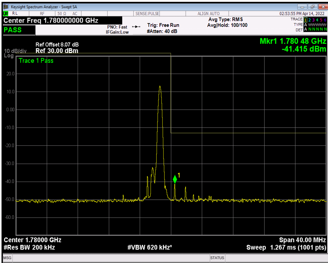
Band66 16QAM BW=20MHz Channel=132572 RB Size=6 Position=#Max NB Index=15
