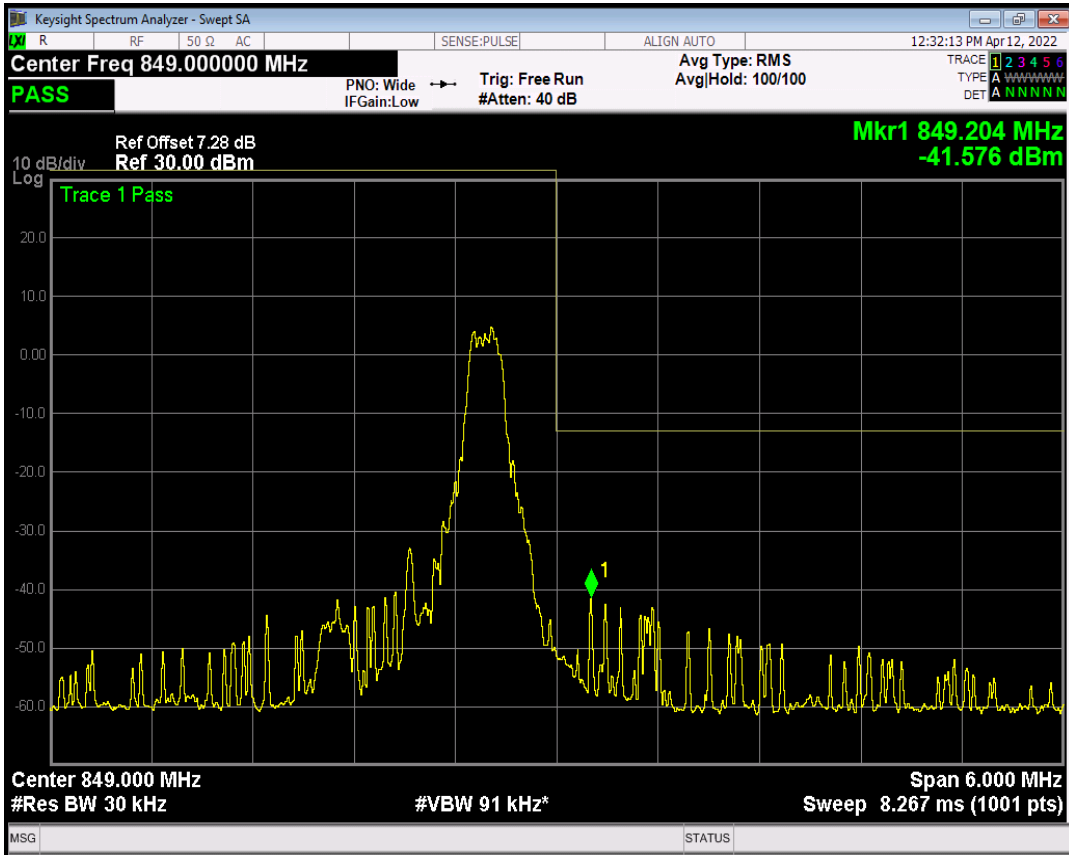
Band5 16QAM BW=3MHz Channel=20635 RB Size=6 Position=#Max NB Index=1
