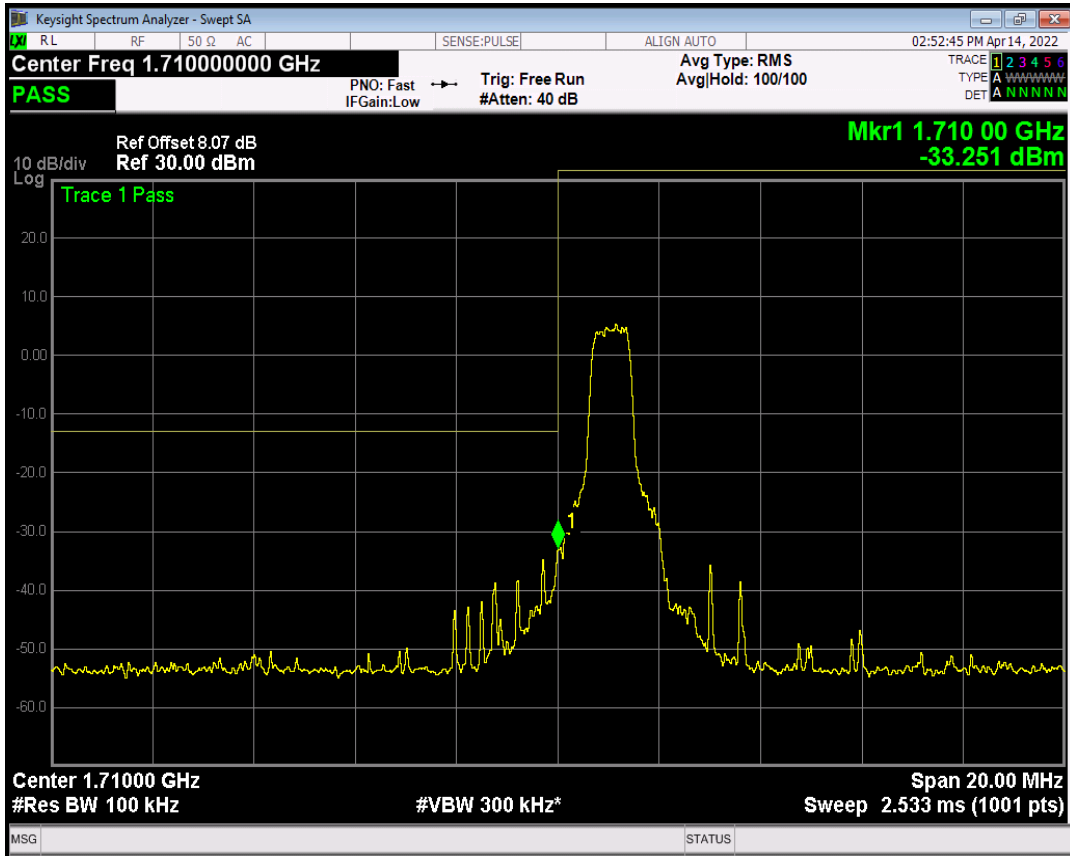
Band66 QPSK BW=10MHz Channel=132622 RB Size=1 Position=#Max NB Index=7
