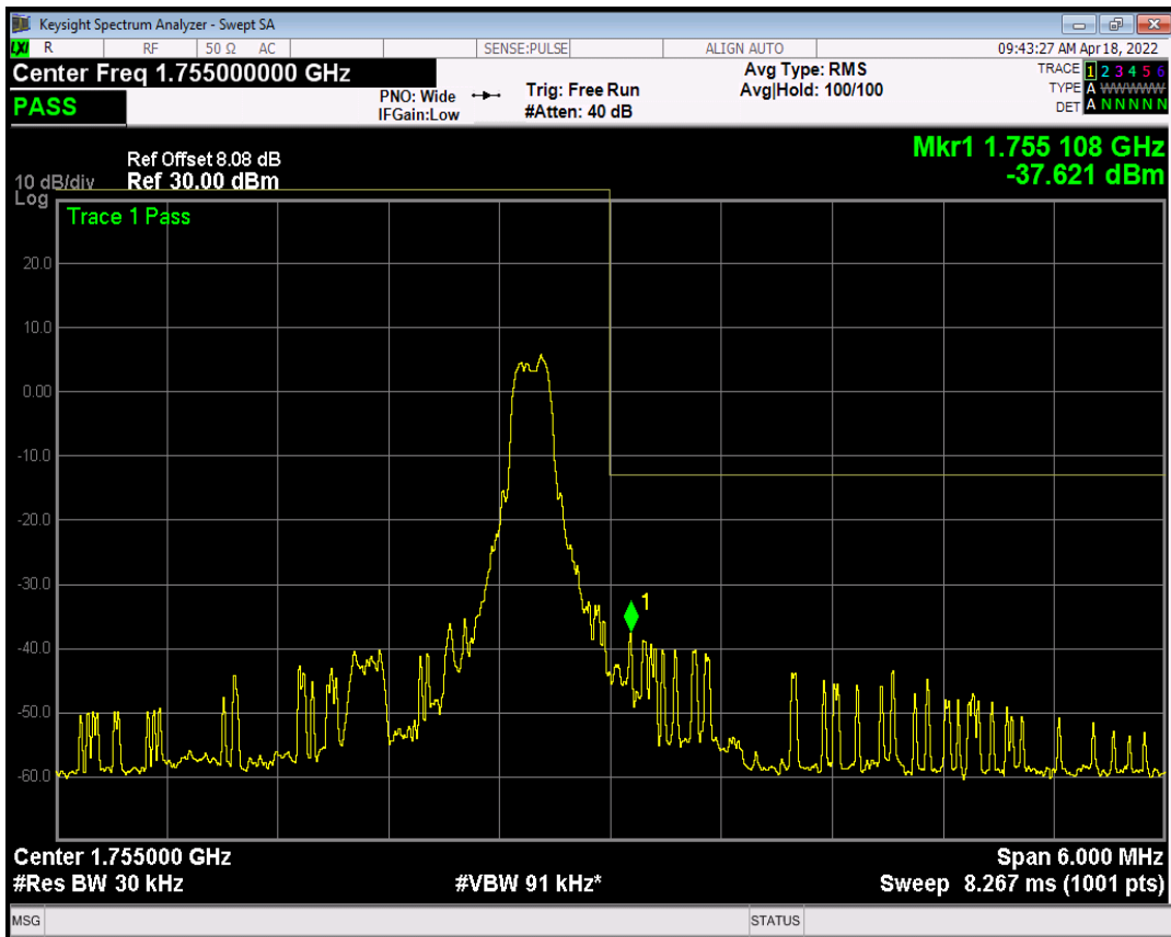
Band4 16QAM BW=3MHz Channel=20385 RB Size=6 Position=#Max NB Index=1
