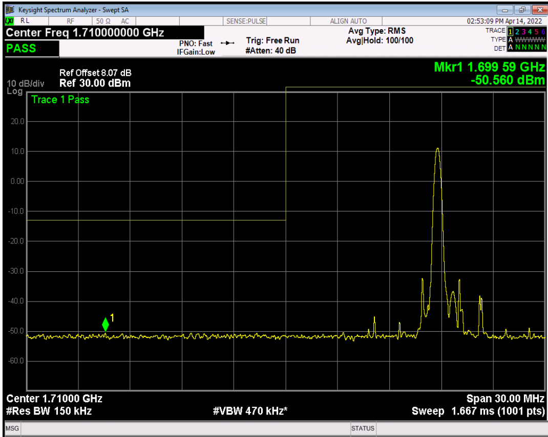
Band66 QPSK BW=15MHz Channel=132047 RB Size=6 Position=#0 NB Index=7
