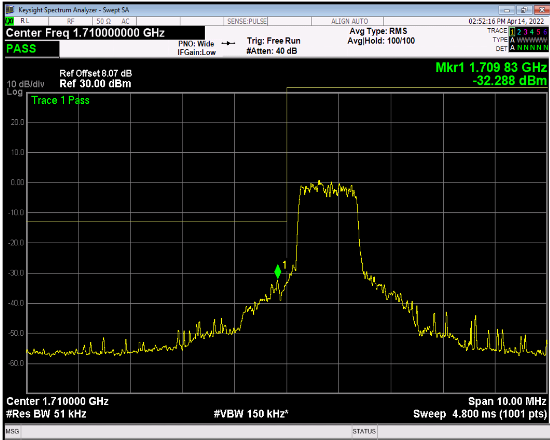
Band66 QPSK BW=5MHz Channel=132647 RB Size=1 Position=#Max NB Index=3
