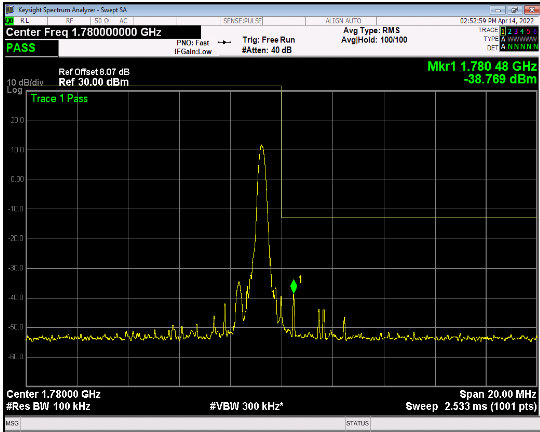
Band66 16QAM BW=10MHz Channel=132622 RB Size=4 Position=#Max NB Index=7
