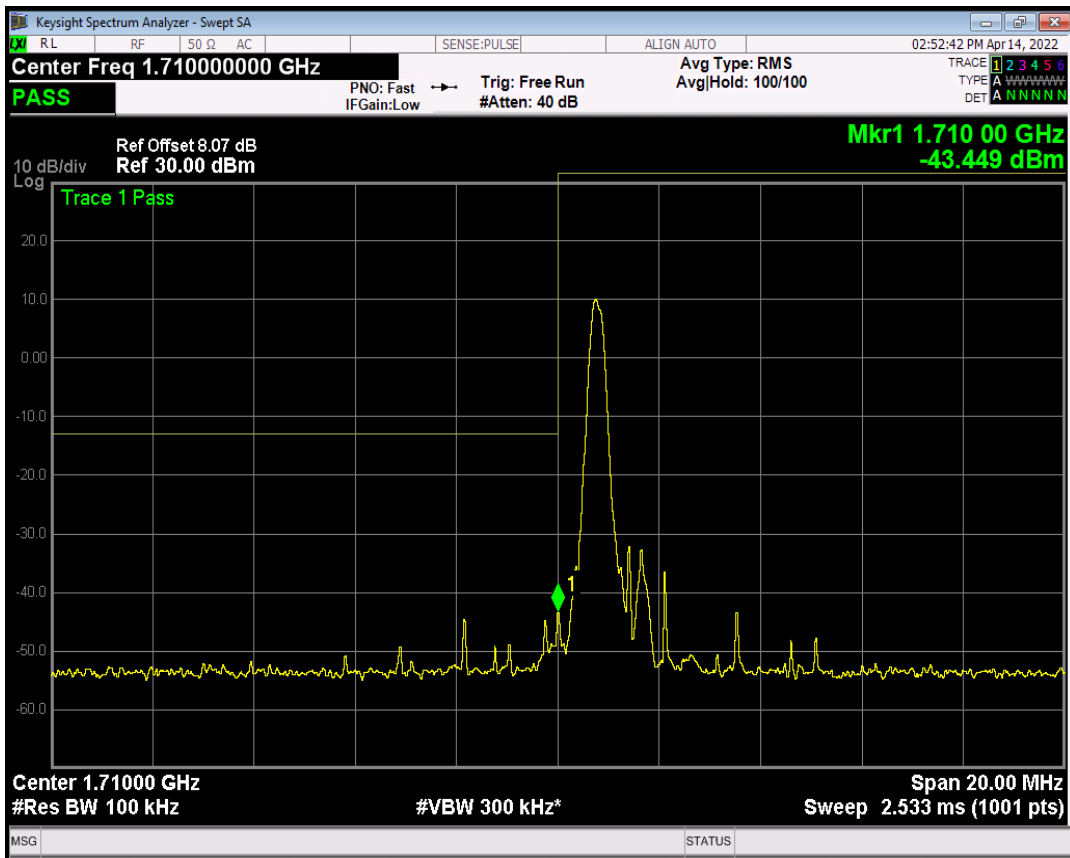
Band66 QPSK BW=10MHz Channel=132022 RB Size=4 Position=#0 NB Index=0
