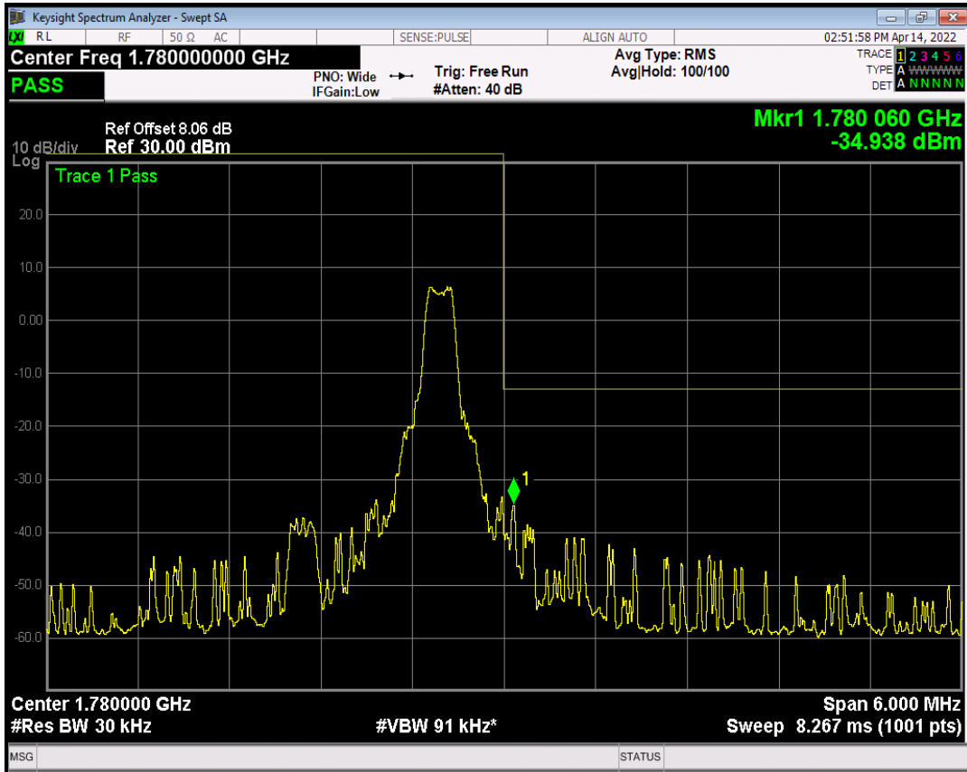
Band66 QPSK BW=3MHz Channel=132657 RB Size=6 Position=#Max NB Index=1
