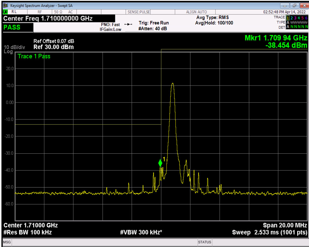
Band66 16QAM BW=10MHz Channel=132022 RB Size=4 Position=#0 NB Index=0
