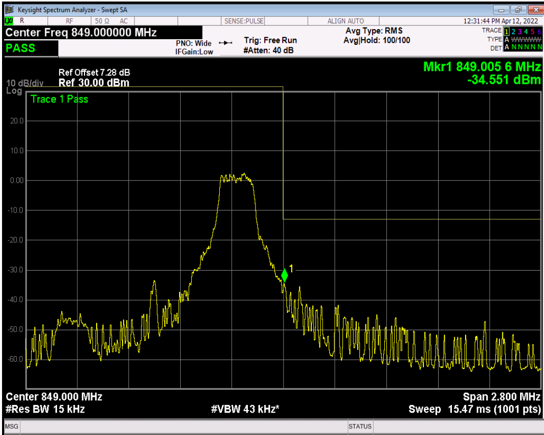
Band5 16QAM BW=1.4MHz Channel=20643 RB Size=6 Position=#Max NB Index=0
