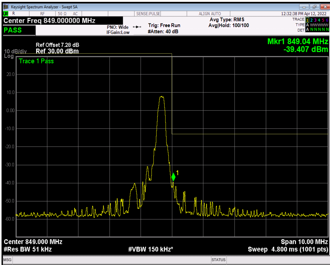
Band5 16QAM BW=5MHz Channel=20625 RB Size=6 Position=#Max NB Index=3
