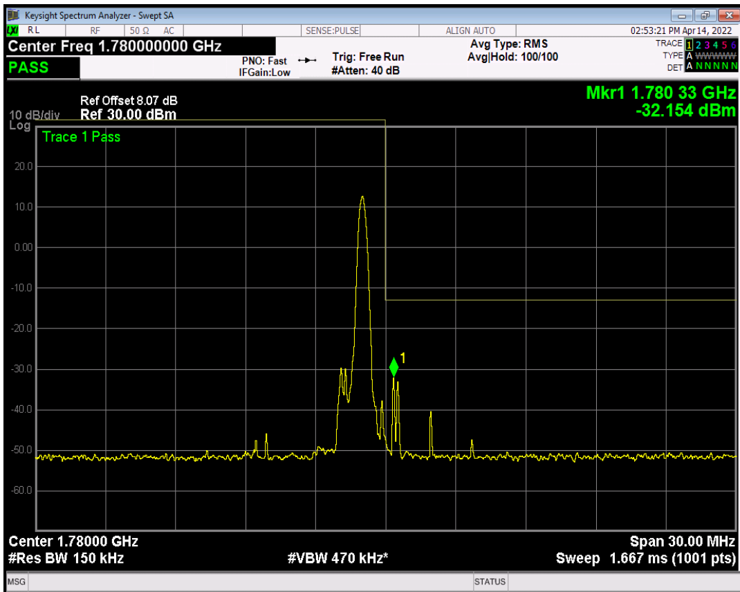
Band66 QPSK BW=15MHz Channel=132597 RB Size=6 Position=#Max NB Index=11
