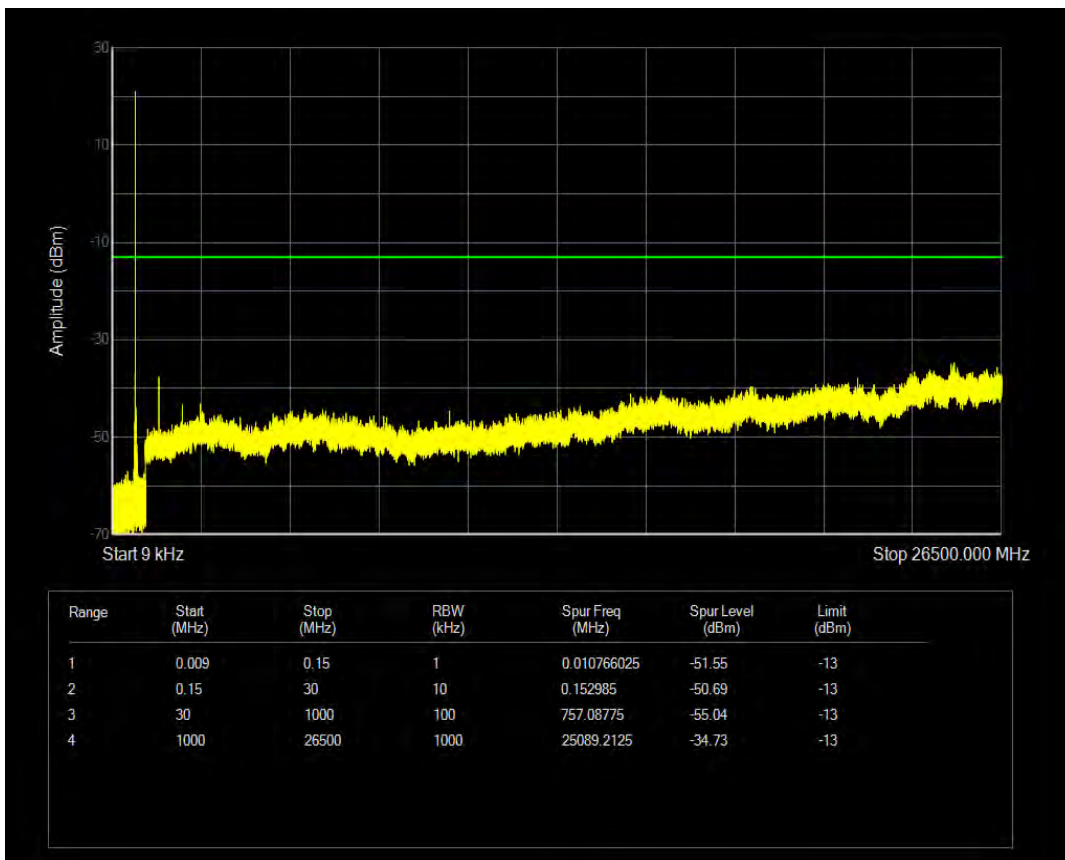
Band12 16QAM BW=10MHz Channel=23060 RB Size=6 Position=#0 NB Index=0
