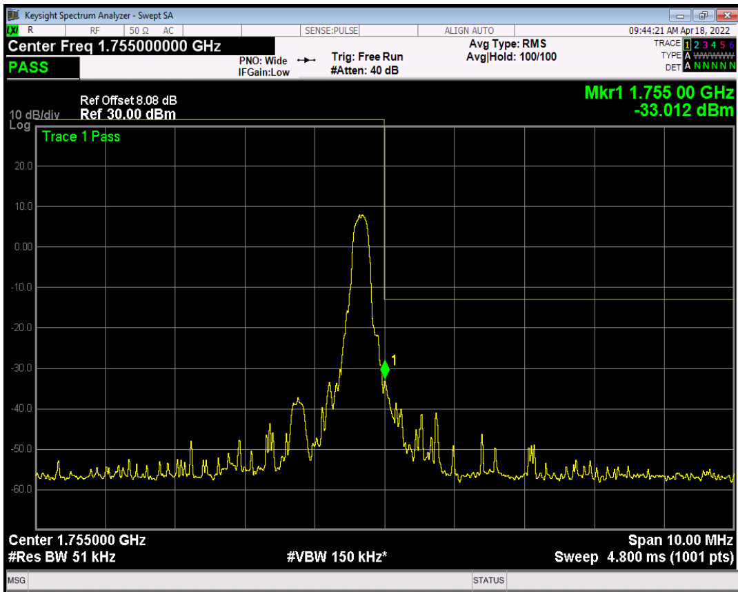
Band4 16QAM BW=5MHz Channel=20375 RB Size=6 Position=#Max NB Index=3
