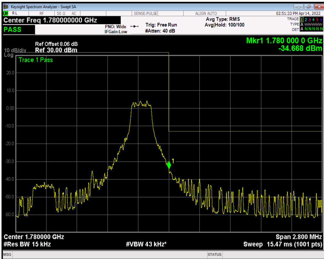
Band66 16QAM BW=1.4MHz Channel=132665 RB Size=6 Position=#Max NB Index=0
