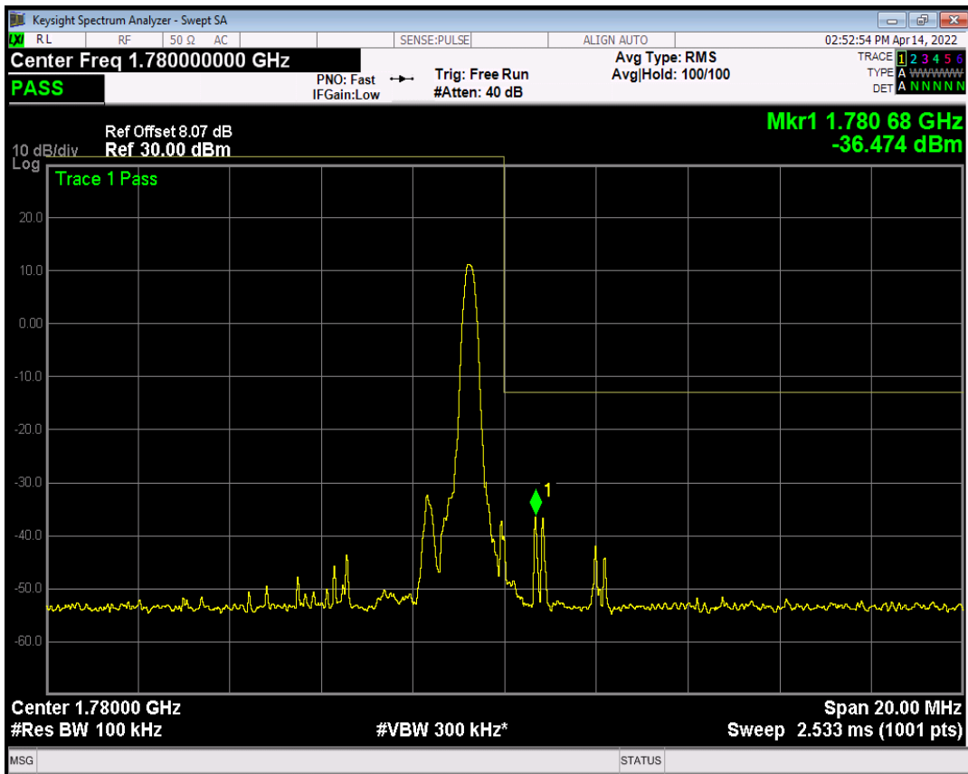
Band66 QPSK BW=10MHz Channel=132622 RB Size=4 Position=#Max NB Index=7
