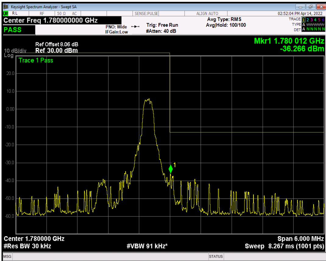
Band66 16QAM BW=3MHz Channel=132657 RB Size=6 Position=#Max NB Index=1
