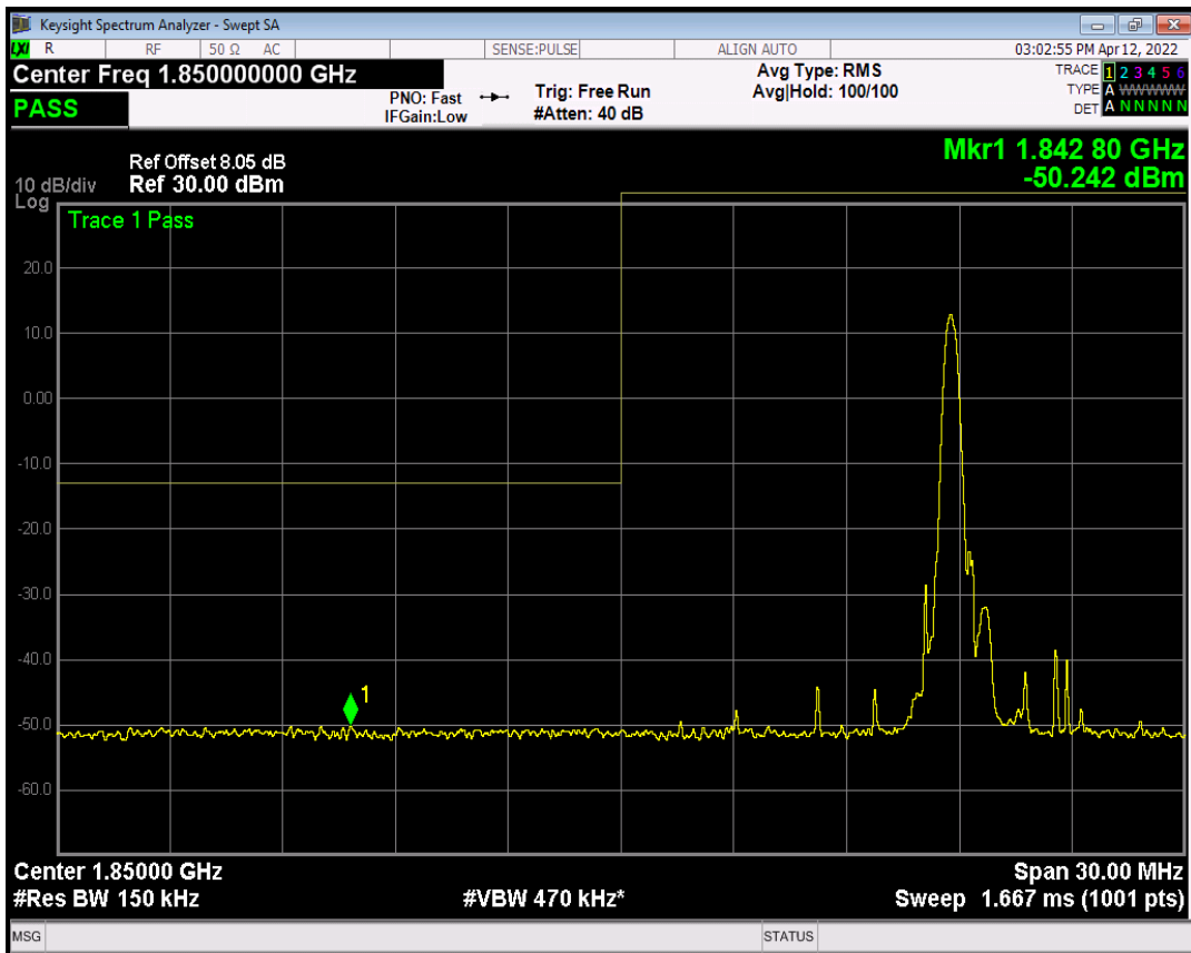
Band25 QPSK BW=15MHz Channel=26115 RB Size=6 Position=#0 NB Index=7
