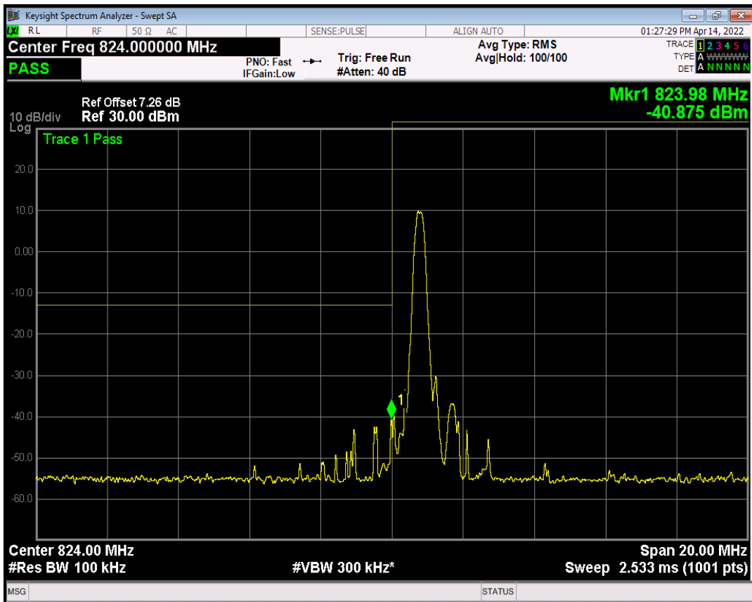
Band26(824-849) 16QAM BW=10MHz Channel=26840 RB Size=4 Position=#0 NB Index=0
