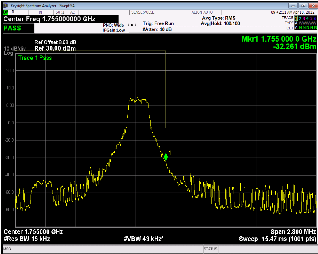
Band4 16QAM BW=1.4MHz Channel=20393 RB Size=6 Position=#Max NB Index=0
