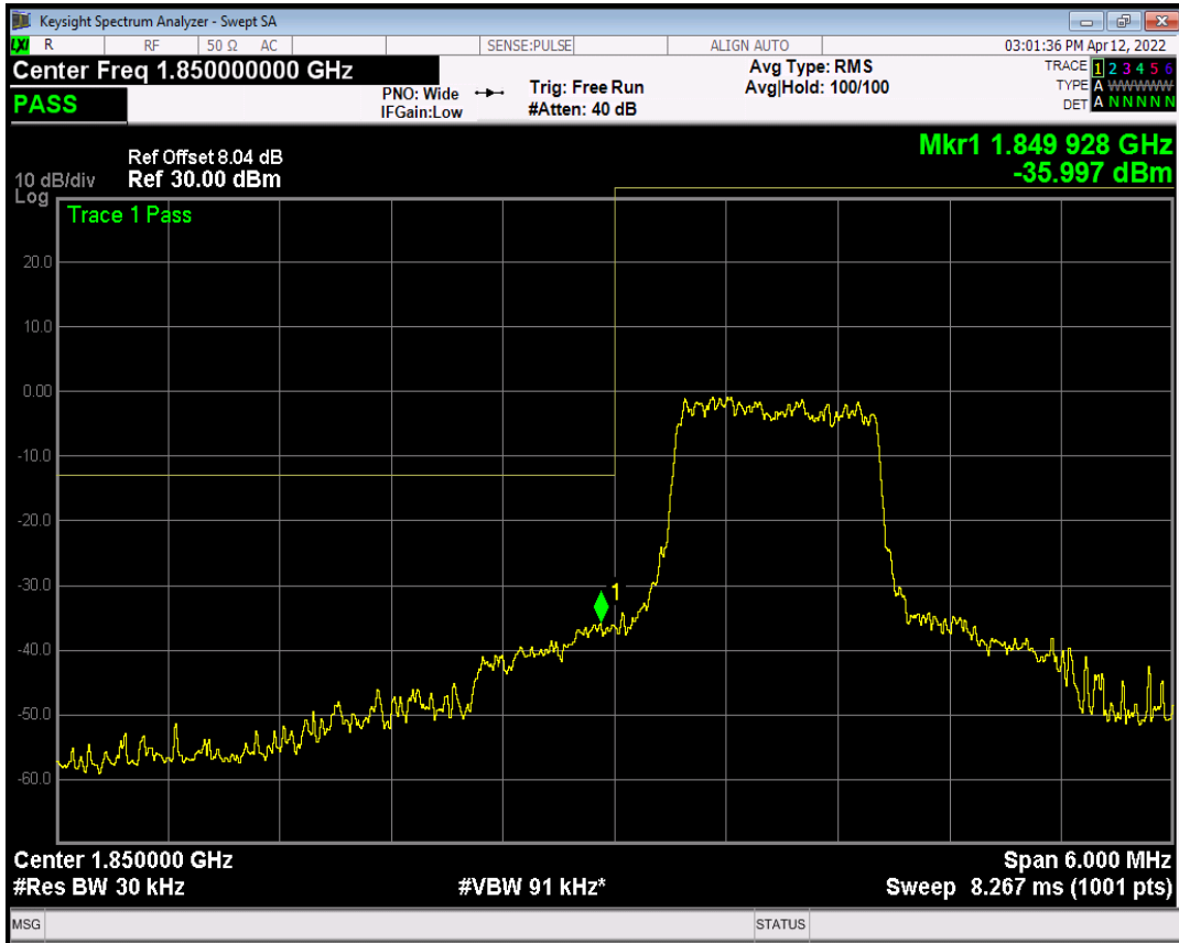
Band25 16QAM BW=3MHz Channel=26675 RB Size=1 Position=#Max NB Index=1
