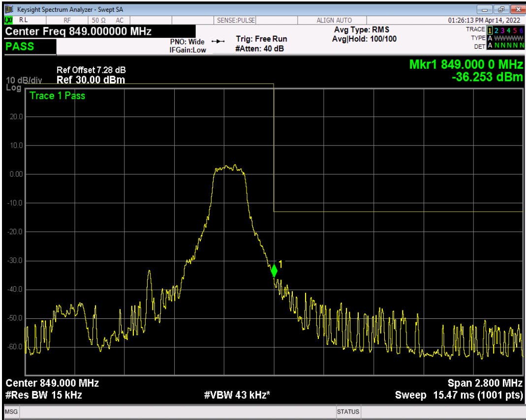
Band26(824-849) 16QAM BW=1.4MHz Channel=27033 RB Size=6 Position=#Max NB Index=0
