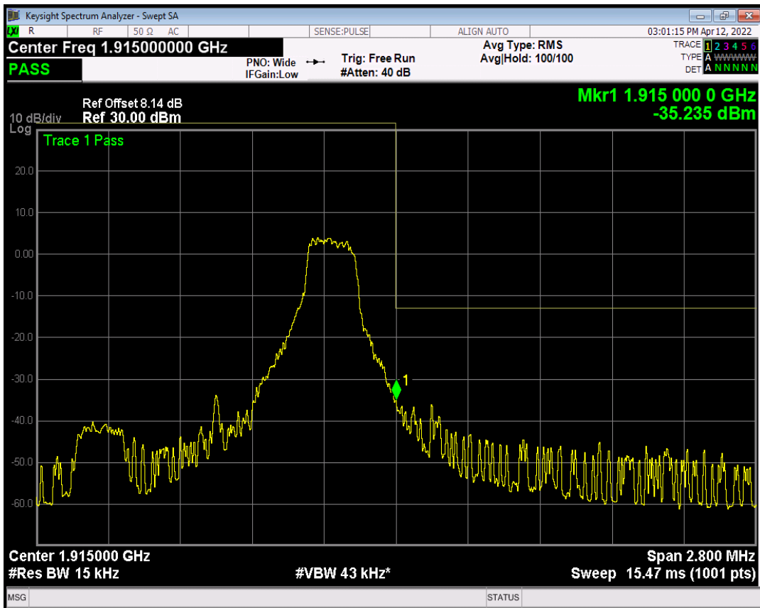
Band25 16QAM BW=1.4MHz Channel=26683 RB Size=6 Position=#Max NB Index=0
