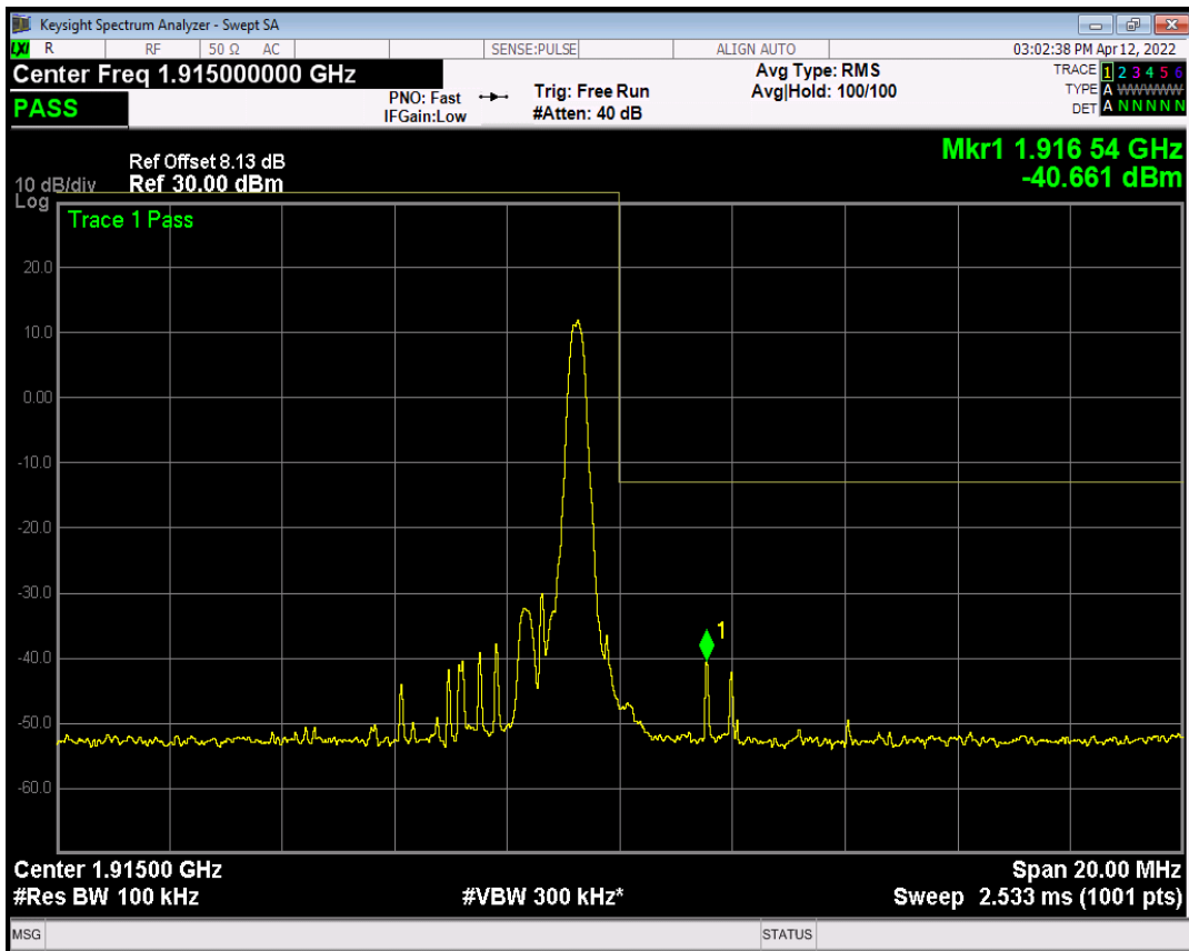
Band25 QPSK BW=10MHz Channel=26640 RB Size=4 Position=#Max NB Index=7
