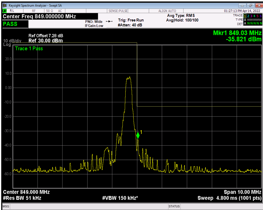
Band26(824-849) 16QAM BW=5MHz Channel=27015 RB Size=6 Position=#Max NB Index=3
