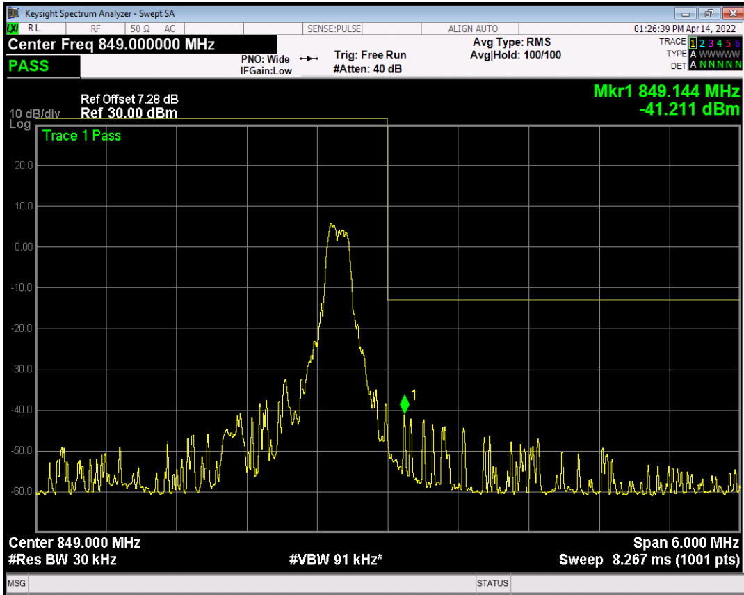
Band26(824-849) QPSK BW=3MHz Channel=27025 RB Size=6 Position=#Max NB Index=1
