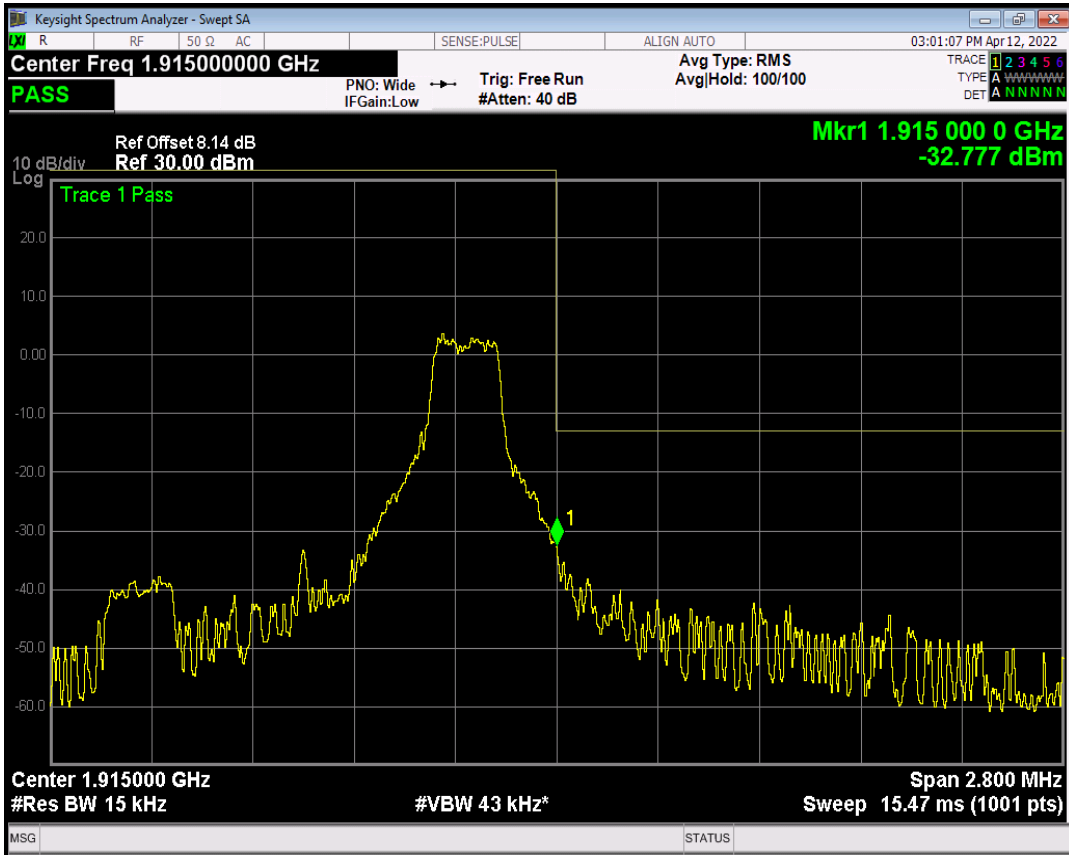
Band25 QPSK BW=1.4MHz Channel=26683 RB Size=6 Position=#Max NB Index=0
