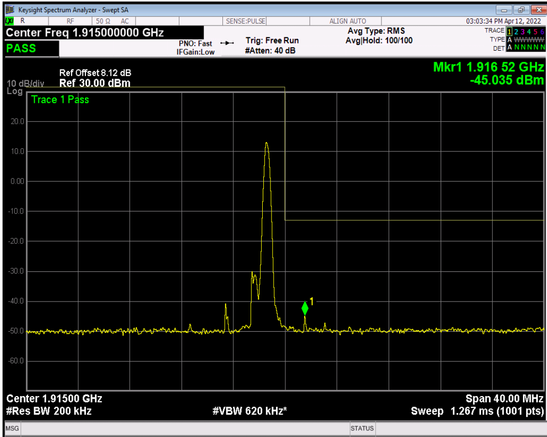
Band25 QPSK BW=20MHz Channel=26590 RB Size=6 Position=#Max NB Index=15
