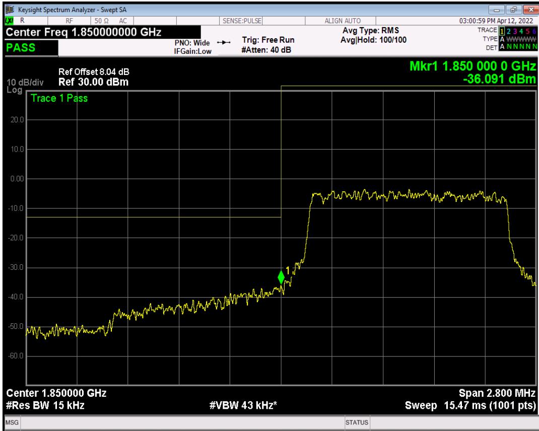
Band25 16QAM BW=1.4MHz Channel=26683 RB Size=1 Position=#Max NB Index=0
