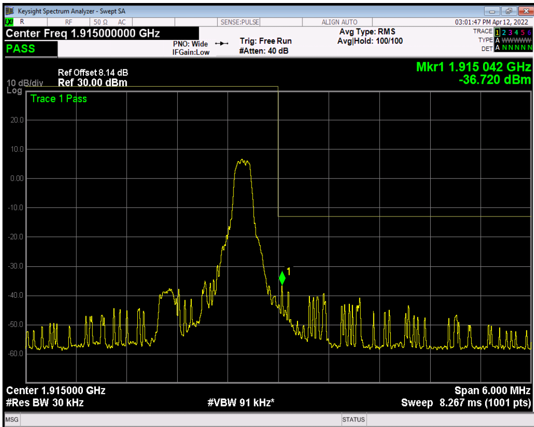
Band25 16QAM BW=3MHz Channel=26675 RB Size=6 Position=#Max NB Index=1
