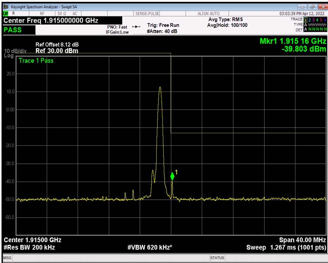
Band25 16QAM BW=20MHz Channel=26590 RB Size=6 Position=#Max NB Index=15
