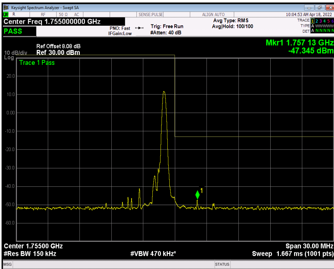
Band4 16QAM BW=15MHz Channel=20325 RB Size=6 Position=#Max NB Index=1
