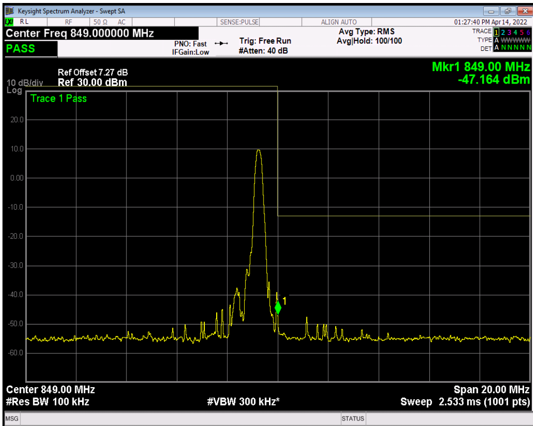
Band26(824-849) 16QAM BW=10MHz Channel=26990 RB Size=4 Position=#Max NB Index=7
