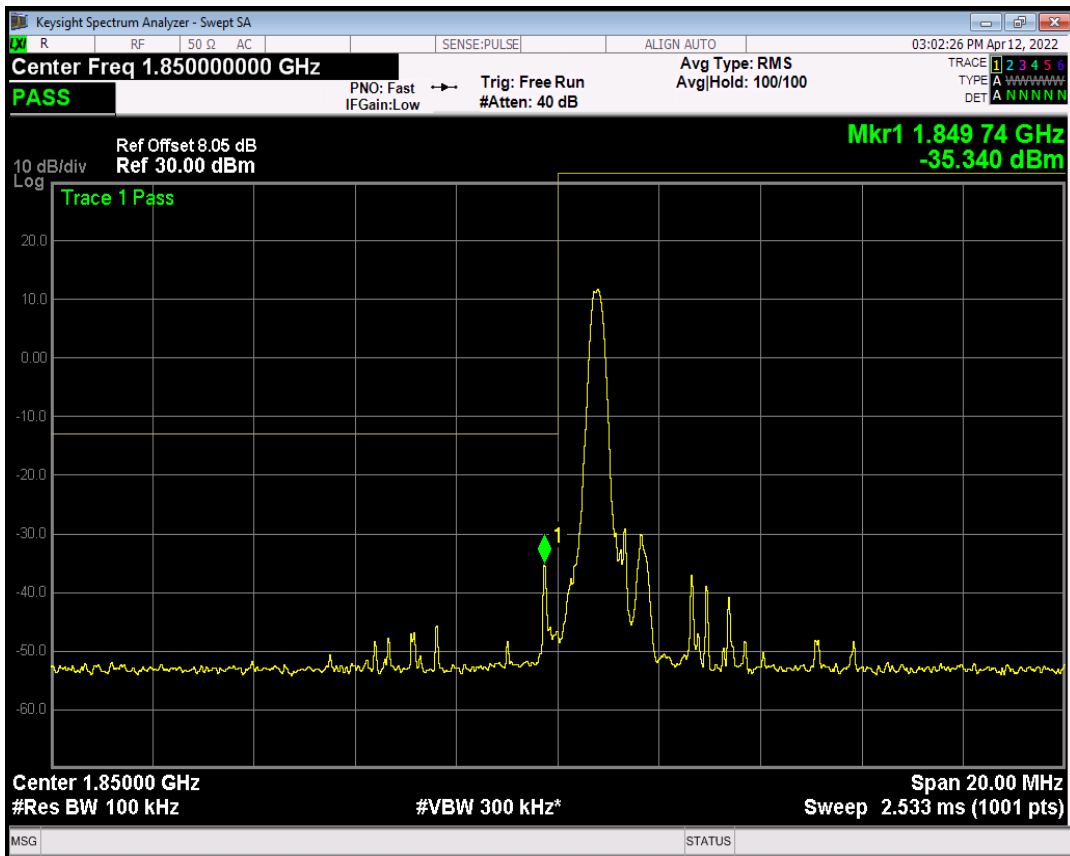
Band25 QPSK BW=10MHz Channel=26090 RB Size=4 Position=#0 NB Index=0
