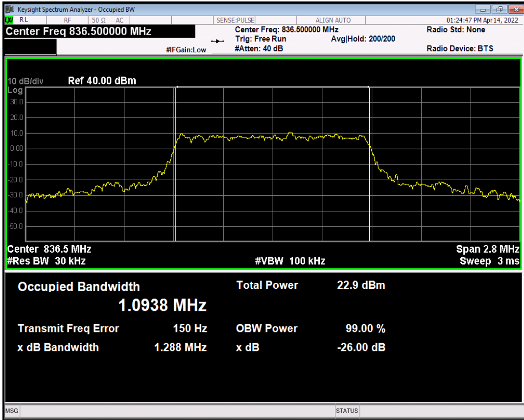
Band26(824-849) 16QAM BW=3MHz Channel=26915 RB Size=6 Position=#0 NB Index=0
