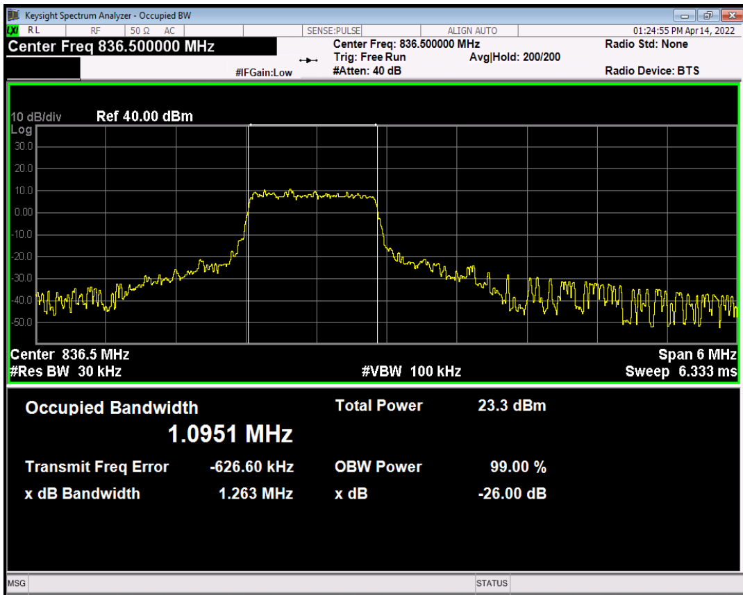
Band26(824-849) 16QAM BW=5MHz Channel=26915 RB Size=6 Position=#0 NB Index=0
