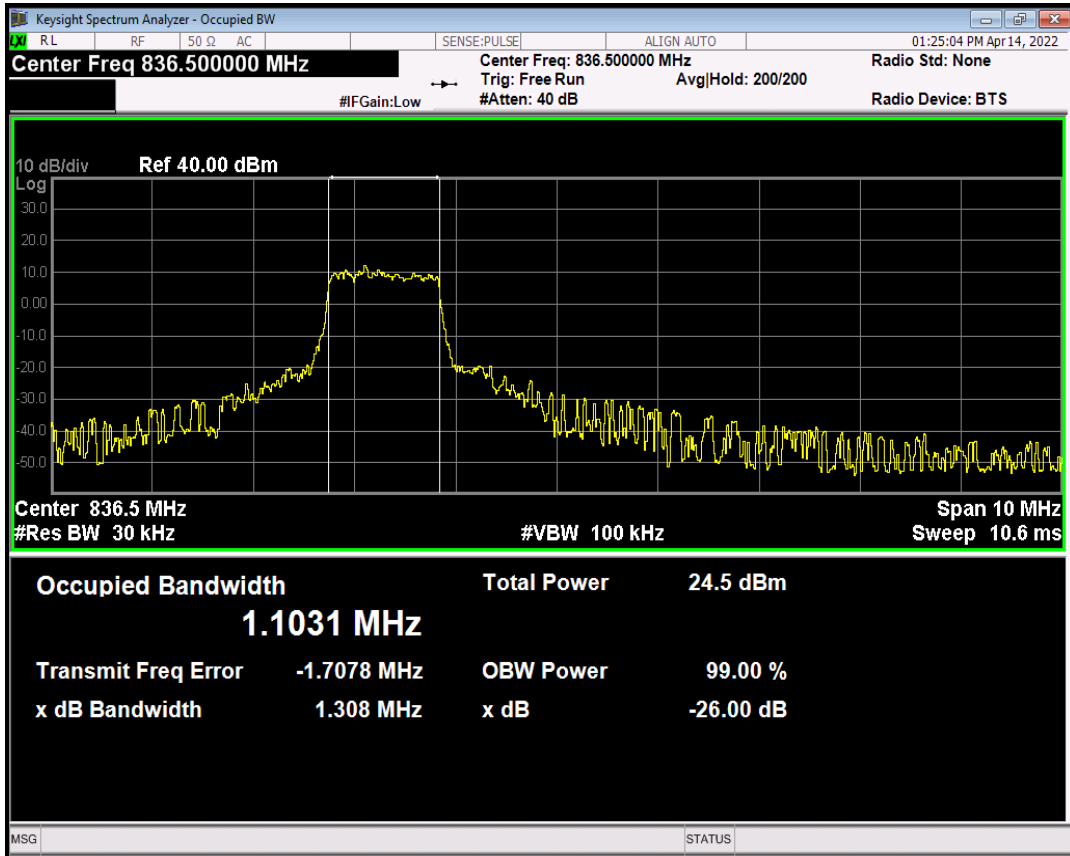
Band26(824-849) 16QAM BW=10MHz Channel=26915 RB Size=6 Position=#0 NB Index=0
