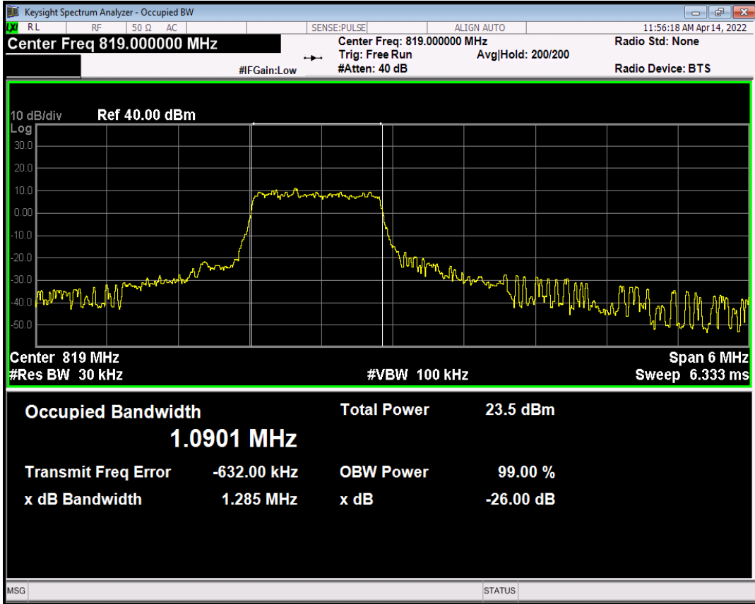
Band26(814-824) 16QAM BW=5MHz Channel=26740 RB Size=6 Position=#0 NB Index=0
