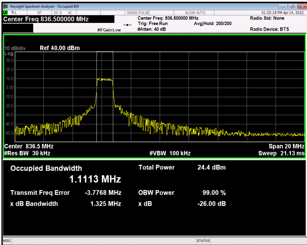
Band26(824-849) 16QAM BW=15MHz Channel=26915 RB Size=6 Position=#0 NB Index=0
