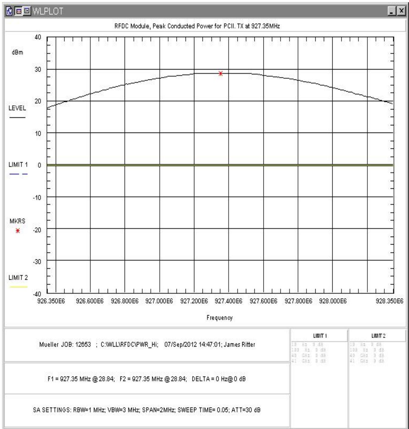
Figure 4: Conducted Peak Power, 927.35MHz
