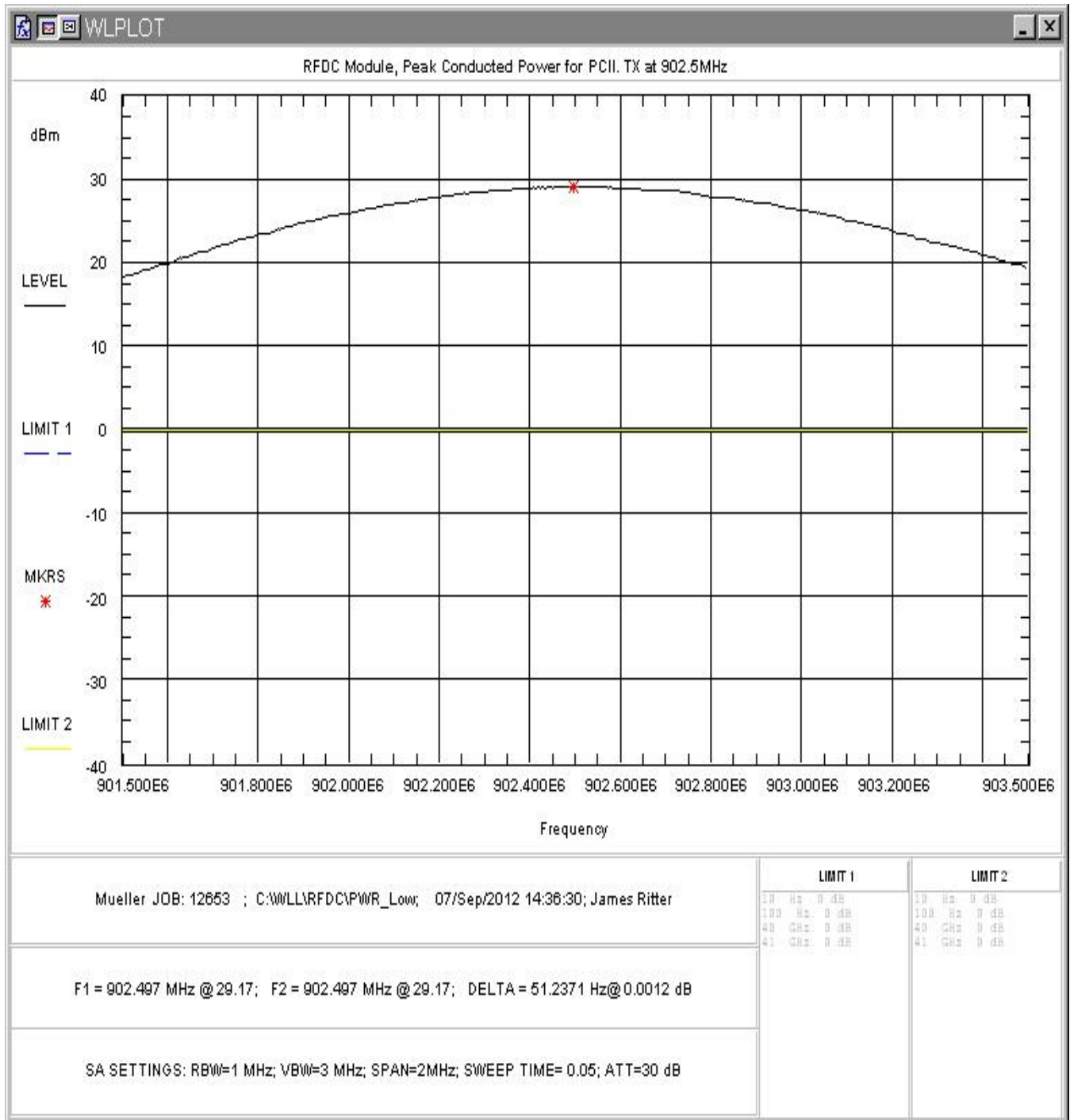
Figure 2: Conducted Peak Power, 902.5MHz
