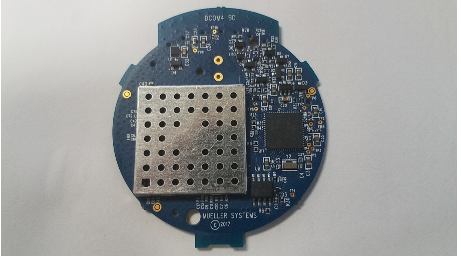
Figure 1: Top View with Shield
