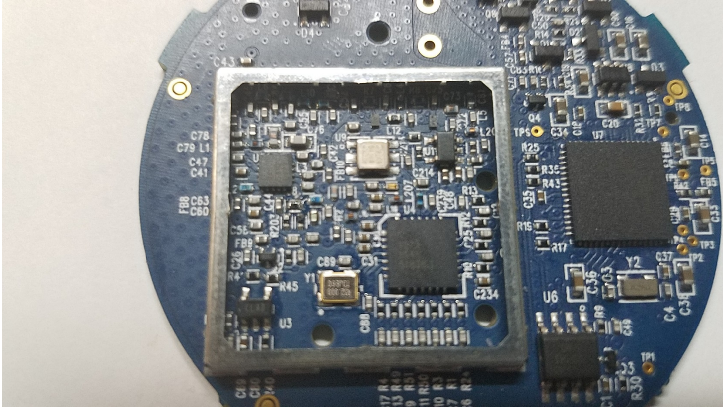
Figure 2: Top View with Shield Removed
