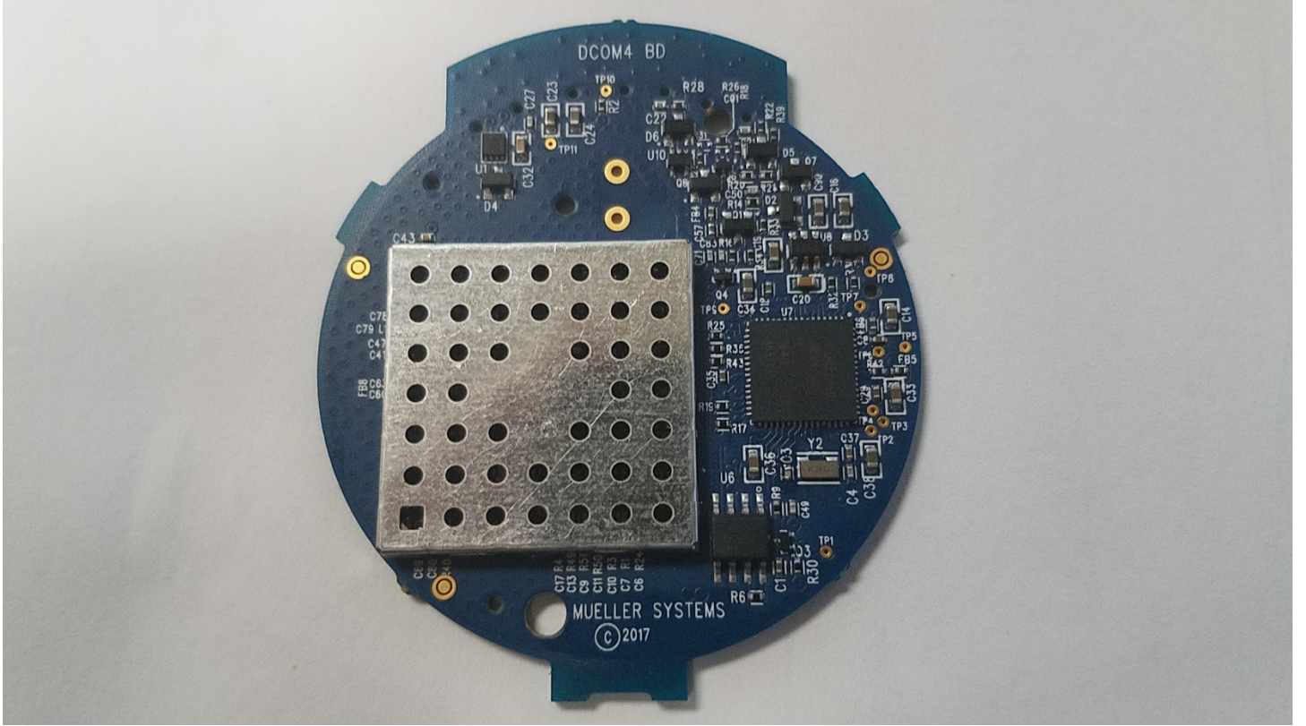
Figure 1: Top View
