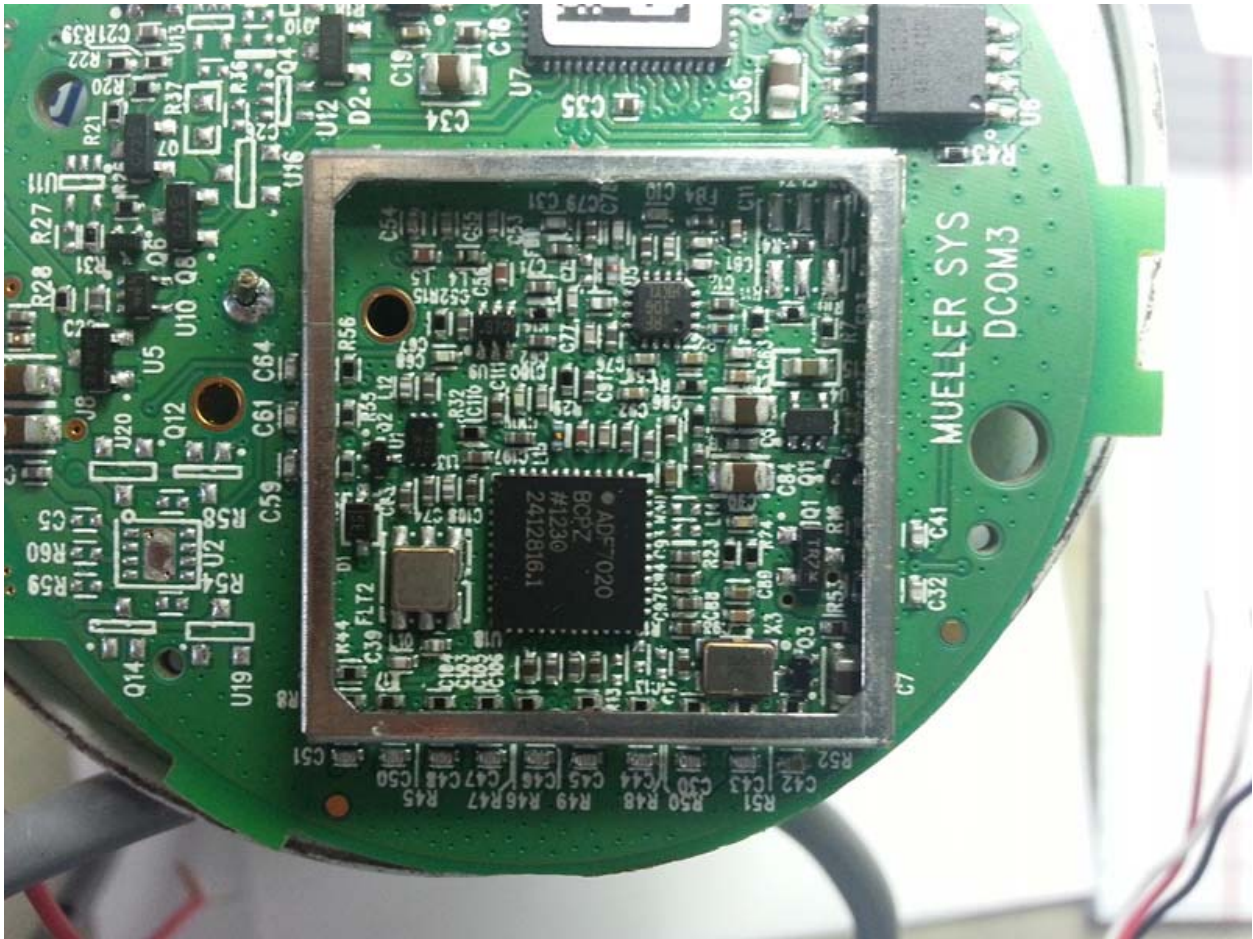
Figure 3 - DCOM3 under shield
