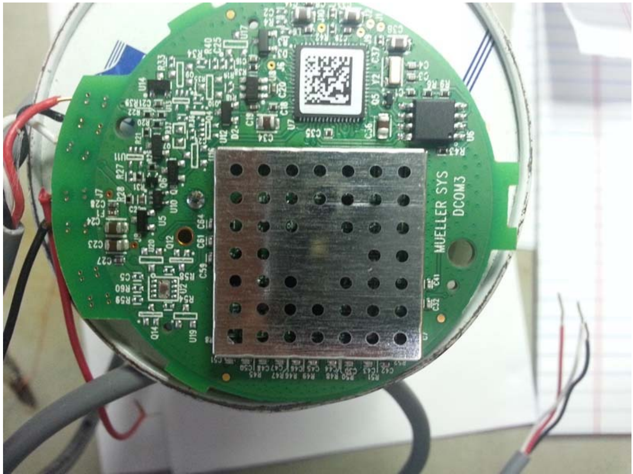
Figure 1- DCOM3 Top side
