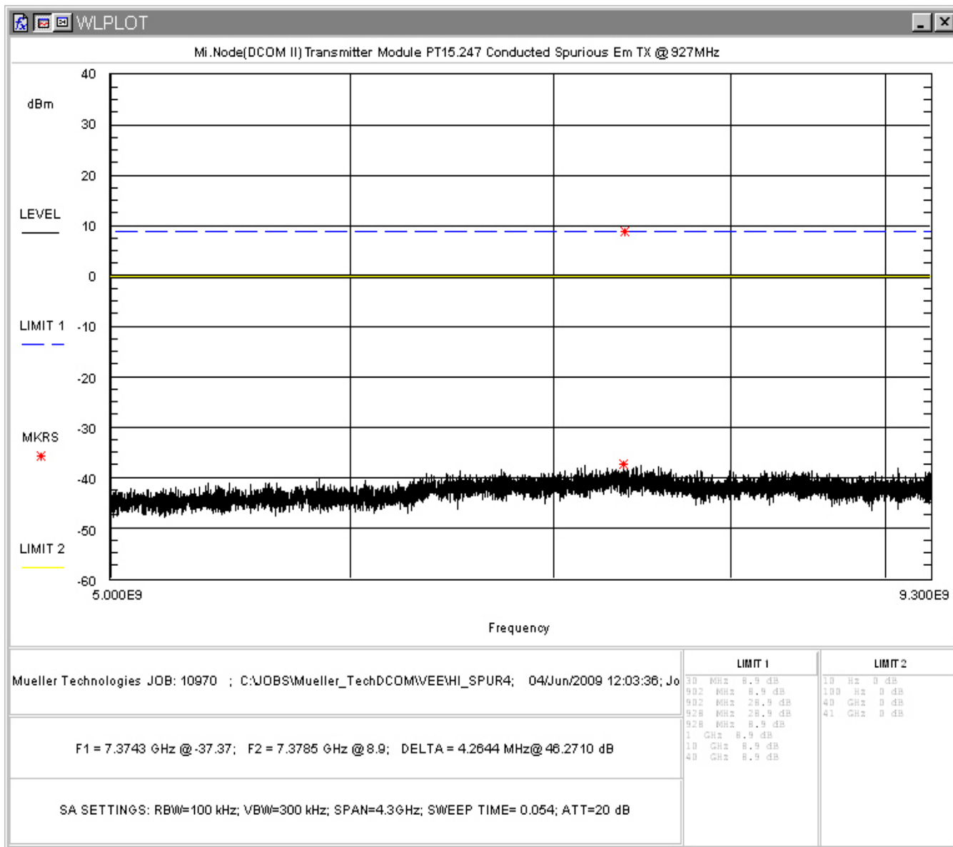
Figure 26: Conducted Spurious Emissions, High Channel 5-9.3GHz
