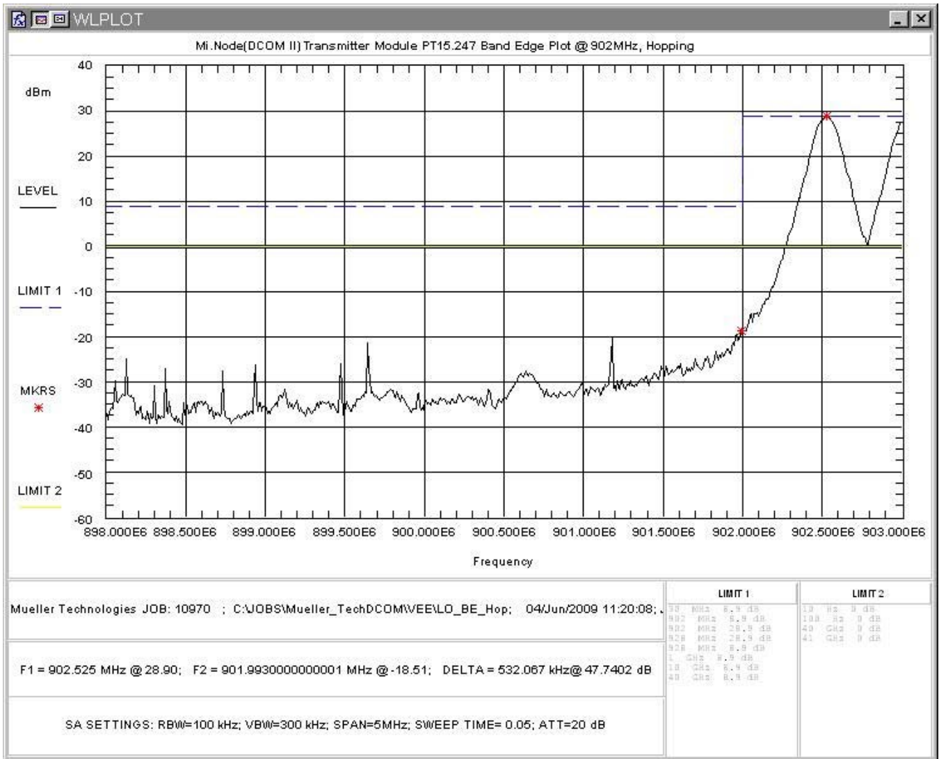
Figure 13: Lower Band Edge Plot, Hopping Mode
