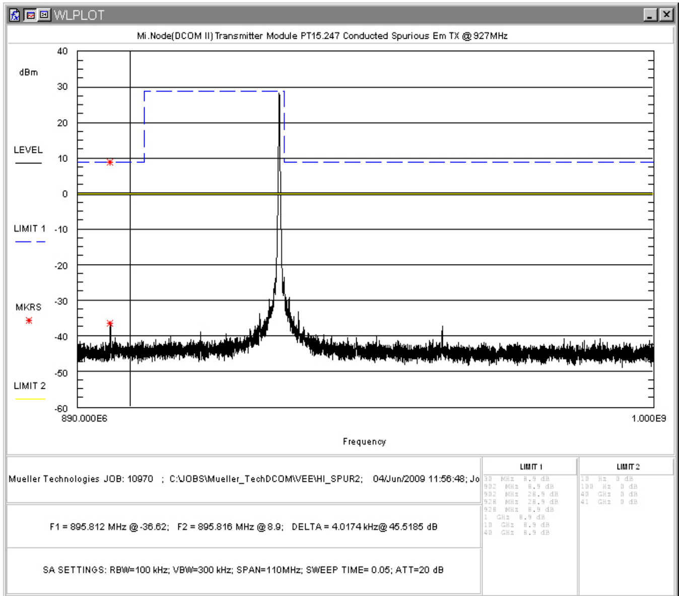
Figure 24: Conducted Spurious Emissions, High Channel 890-1000MHz
