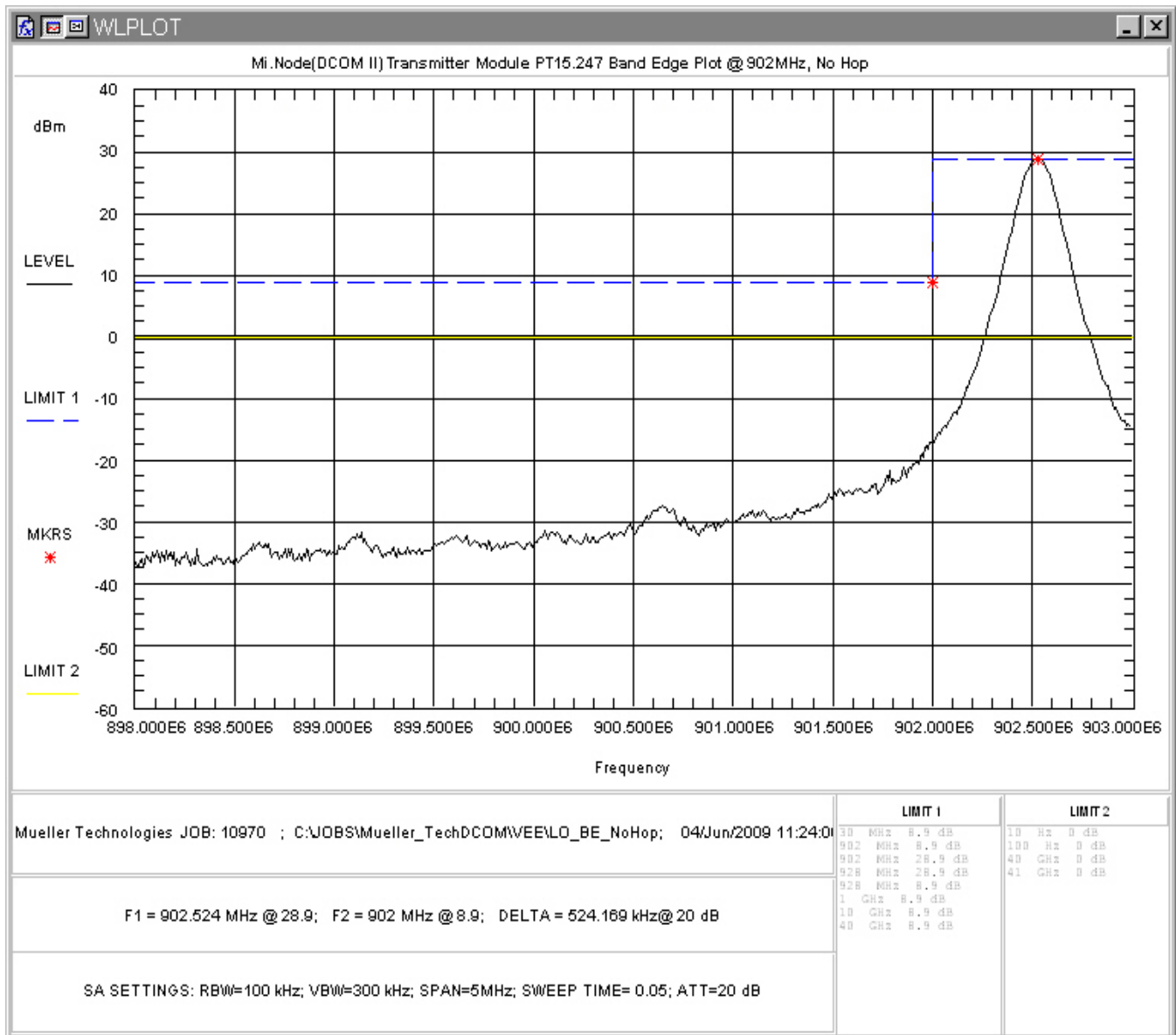
Figure 11: Lower Band Edge Plot, Low Channel, Non-Hopping
