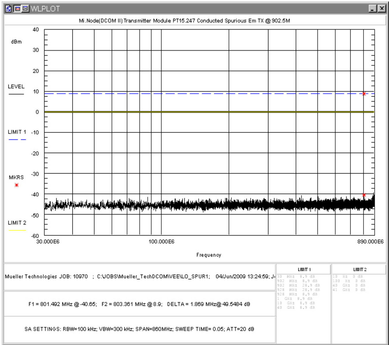
Figure 15: Conducted Spurious Emissions, Low Channel 30 - 890MHz
