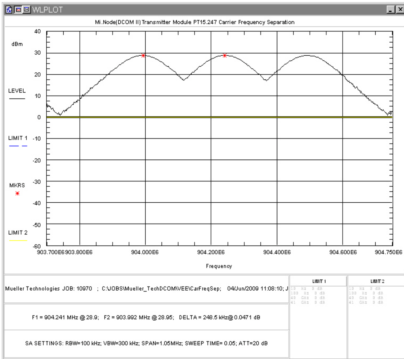
Figure 9: Channel Spacing
