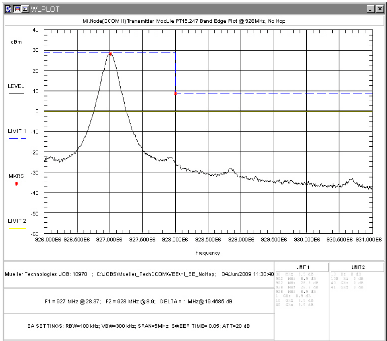
Figure 12: Upper Band Edge Plot, High Channel, Non-Hopping
