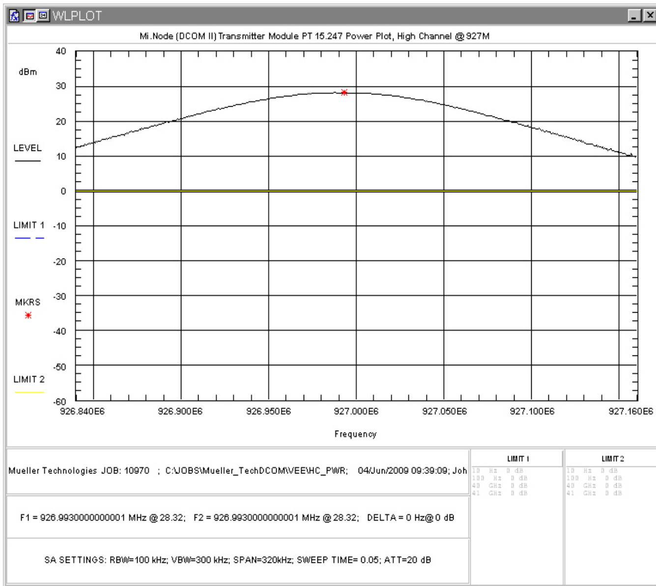
Figure 5: RF Peak Power, High Channel
