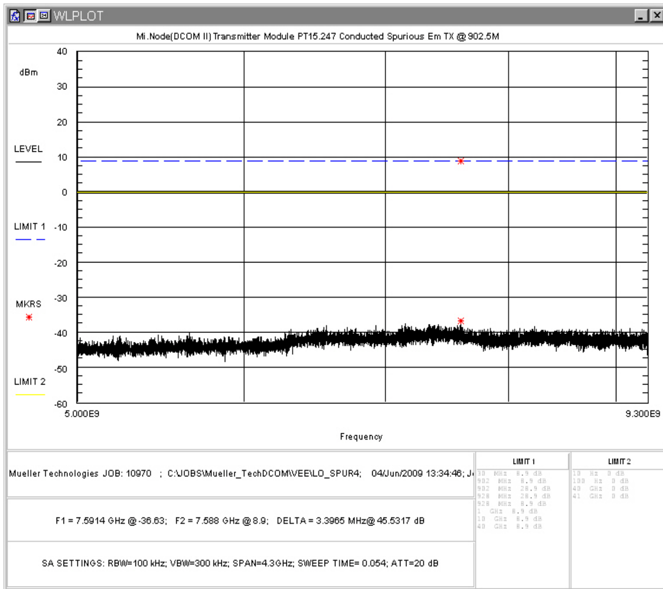
Figure 18: Conducted Spurious Emissions, Low Channel 5 -9.3GHz
