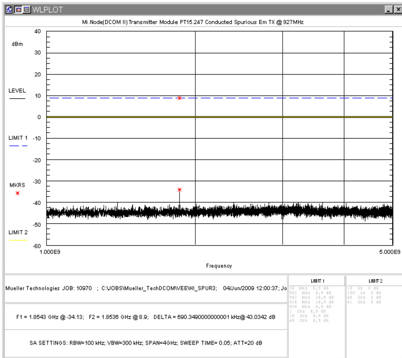
Figure 25: Conducted Spurious Emissions, High Channel 1-5GHz
