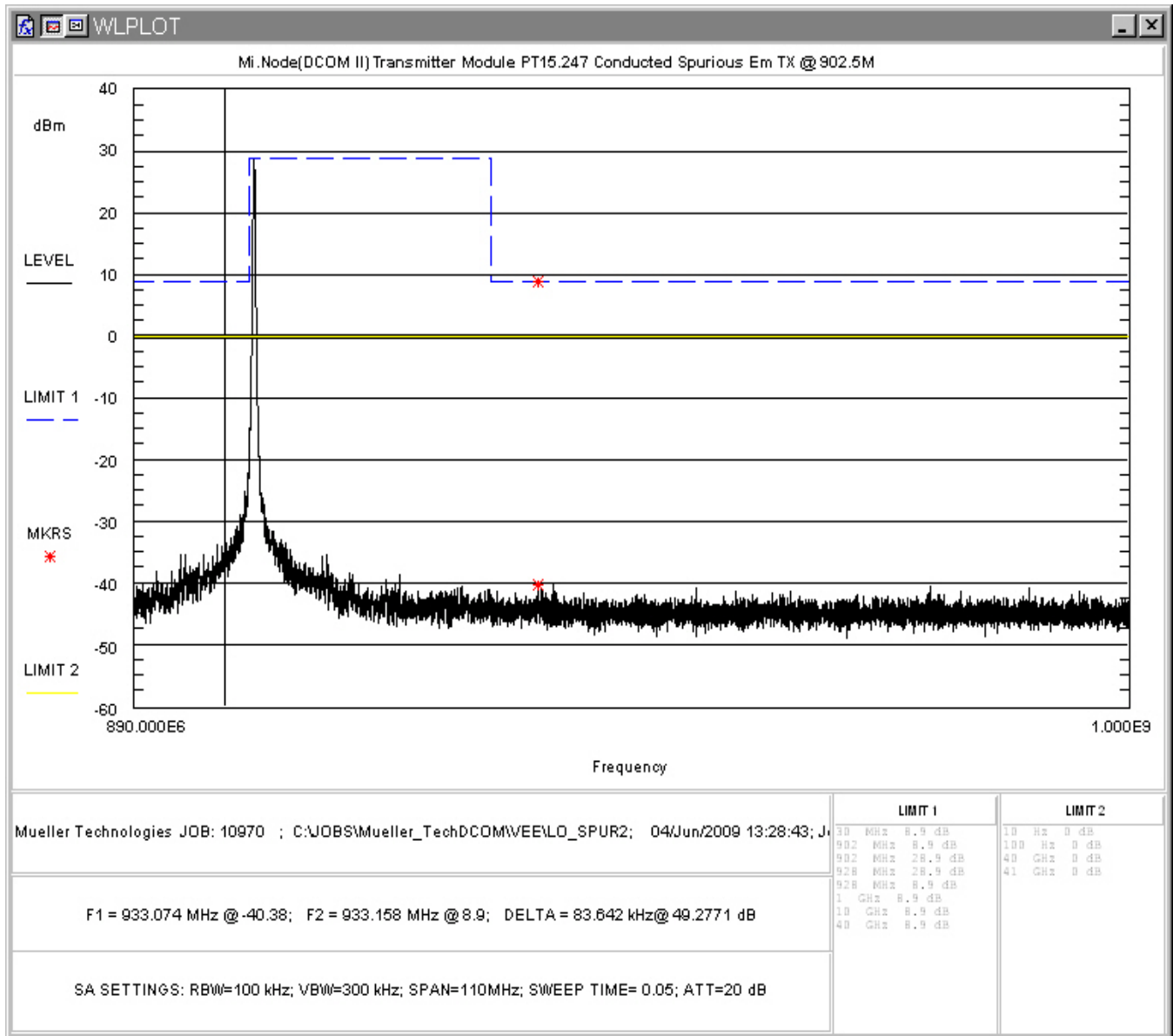
Figure 16: Conducted Spurious Emissions, Low Channel 890-1000MHz
