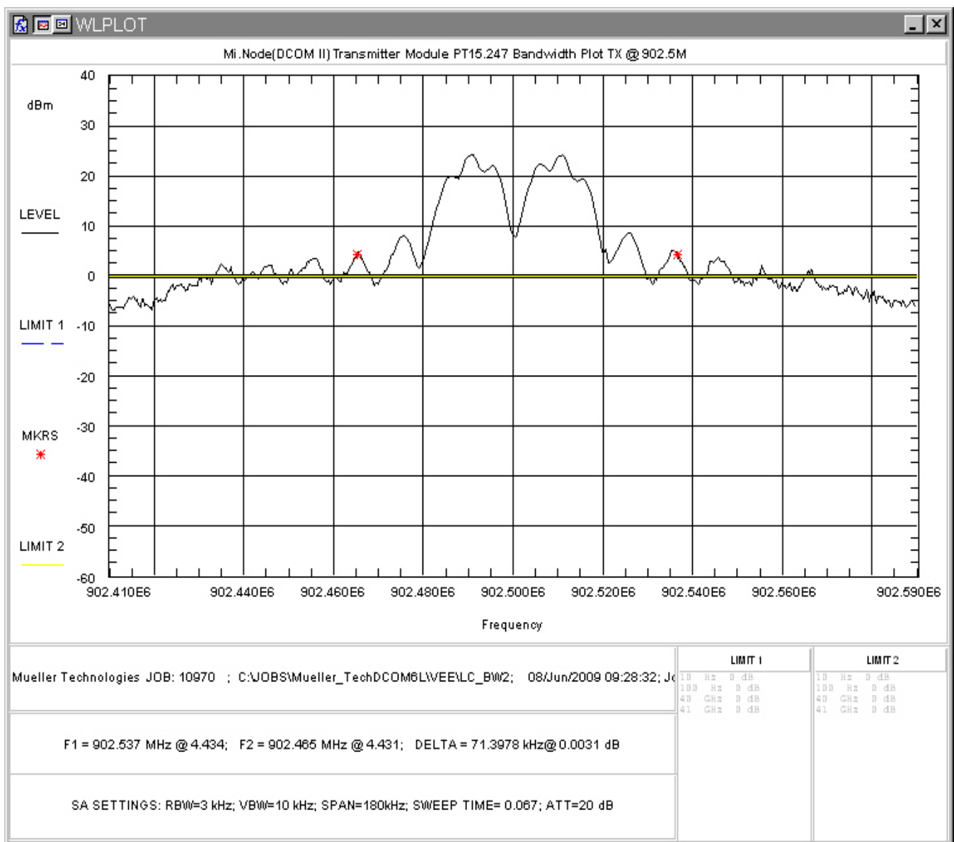
Figure 6: Occupied Bandwidth, Low Channel
