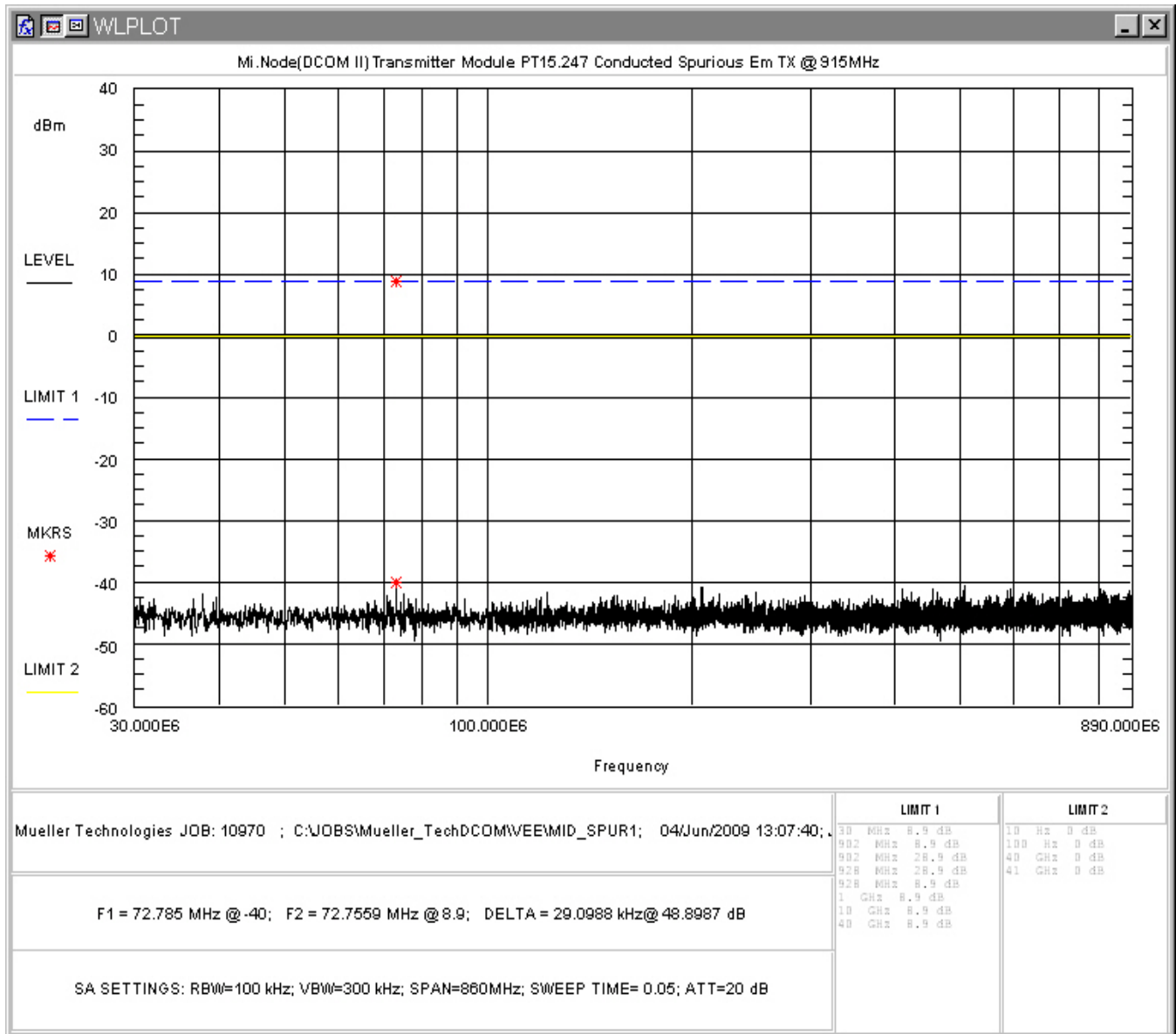
Figure 19: Conducted Spurious Emissions, Mid Channel 30 - 890MHz
