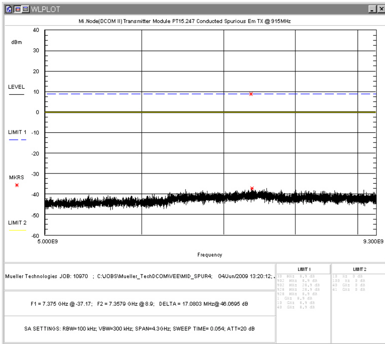
Figure 22: Conducted Spurious Emissions, Mid Channel 5 – 9.3GHz
