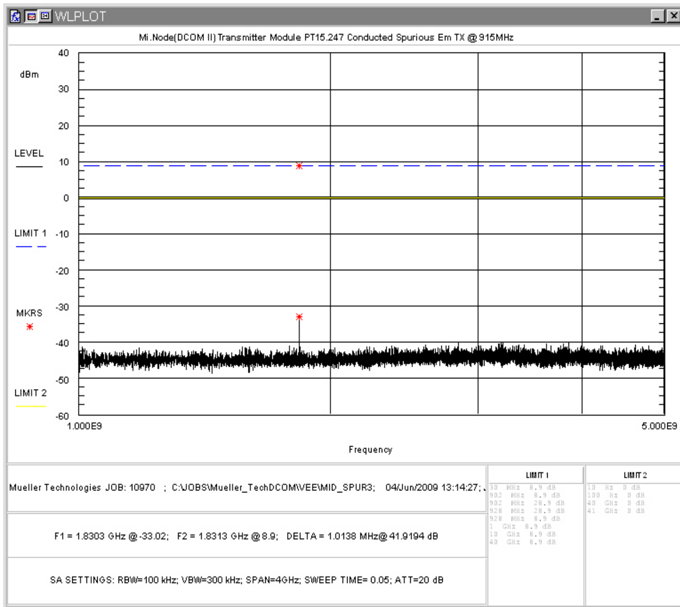
Figure 21: Conducted Spurious Emissions, Mid Channel 1-5GHz
