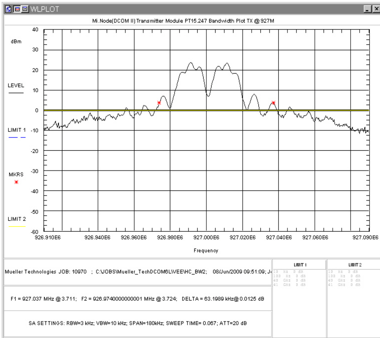
Figure 8: Occupied Bandwidth, High Channel
