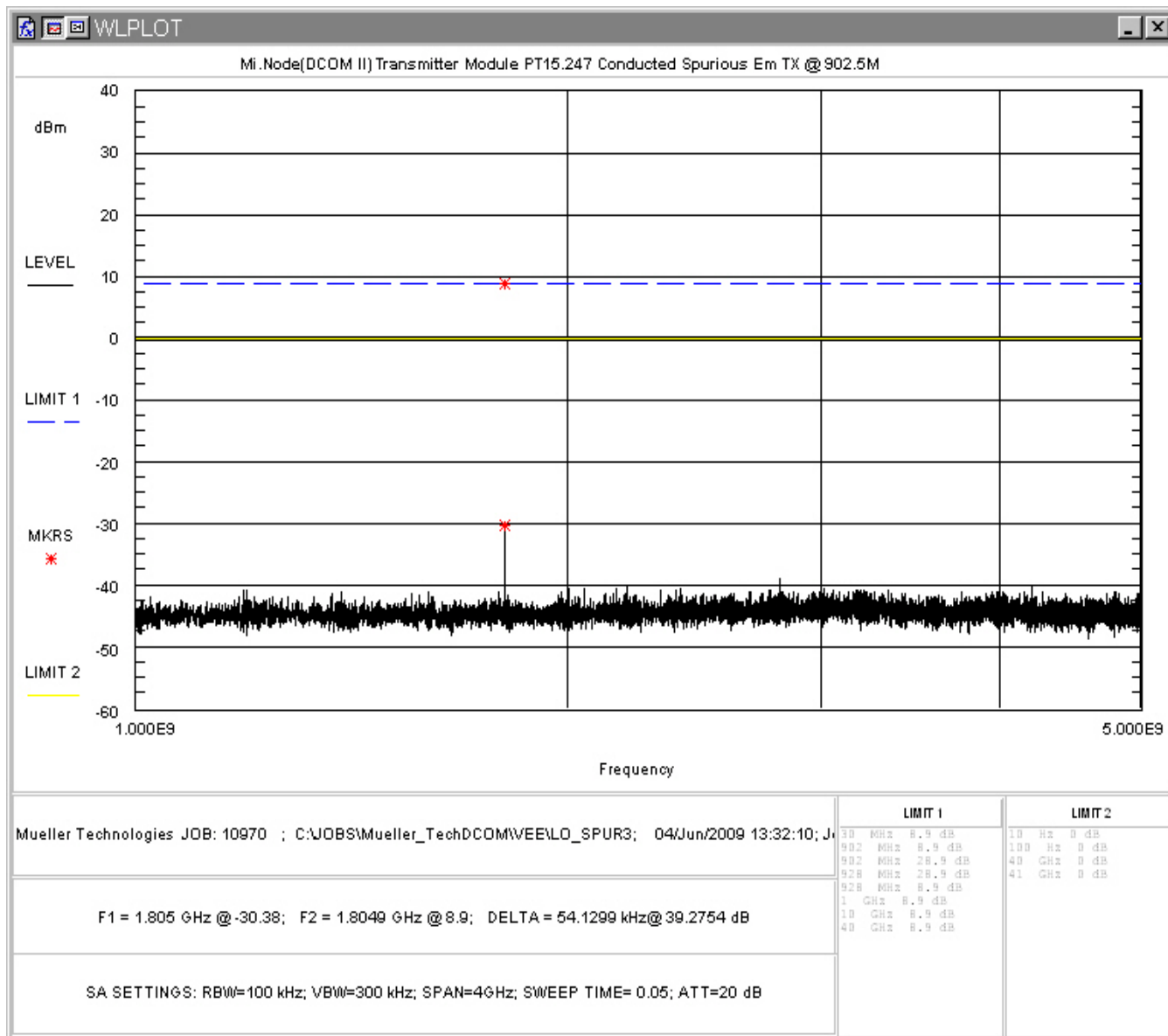
Figure 17: Conducted Spurious Emissions, Low Channel 1-5GHz
