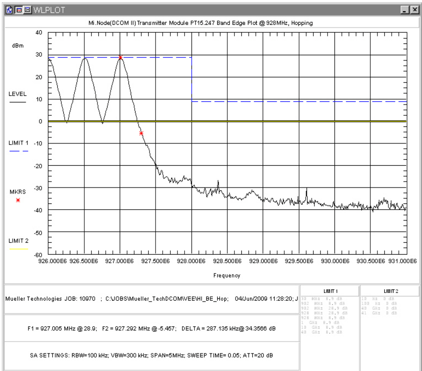
Figure 14: Upper Band Edge Plot, Hopping Mode
