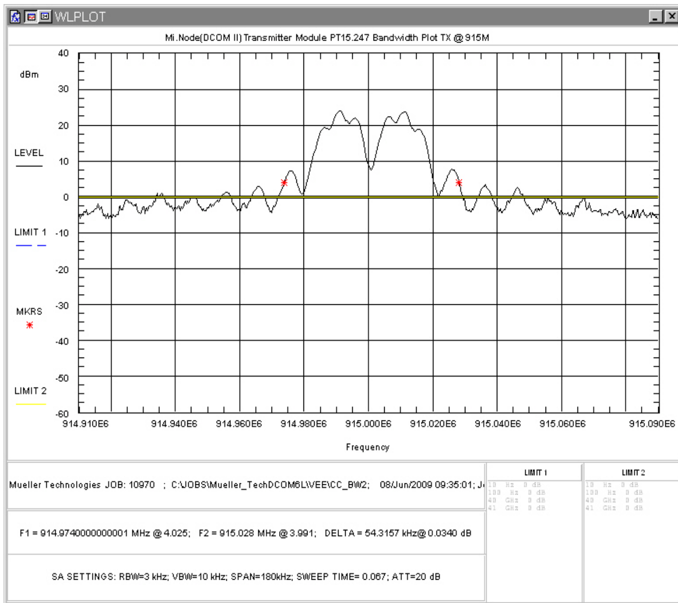
Figure 7: Occupied Bandwidth, Mid Channel
