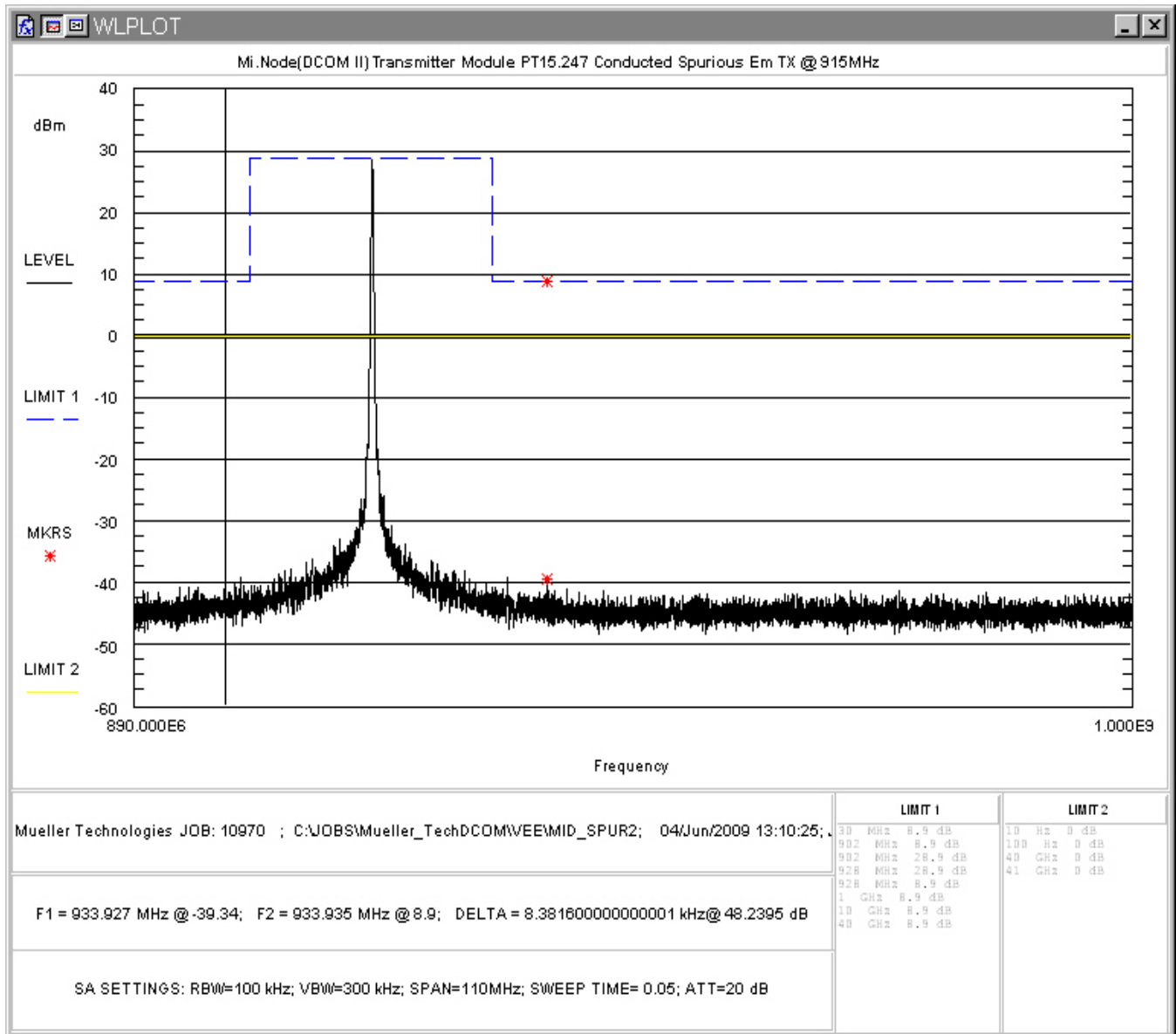
Figure 20: Conducted Spurious Emissions, Mid Channel 890-1000MHz
