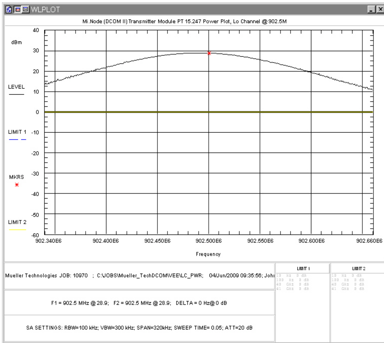
Figure 3: RF Peak Power, Low Channel
