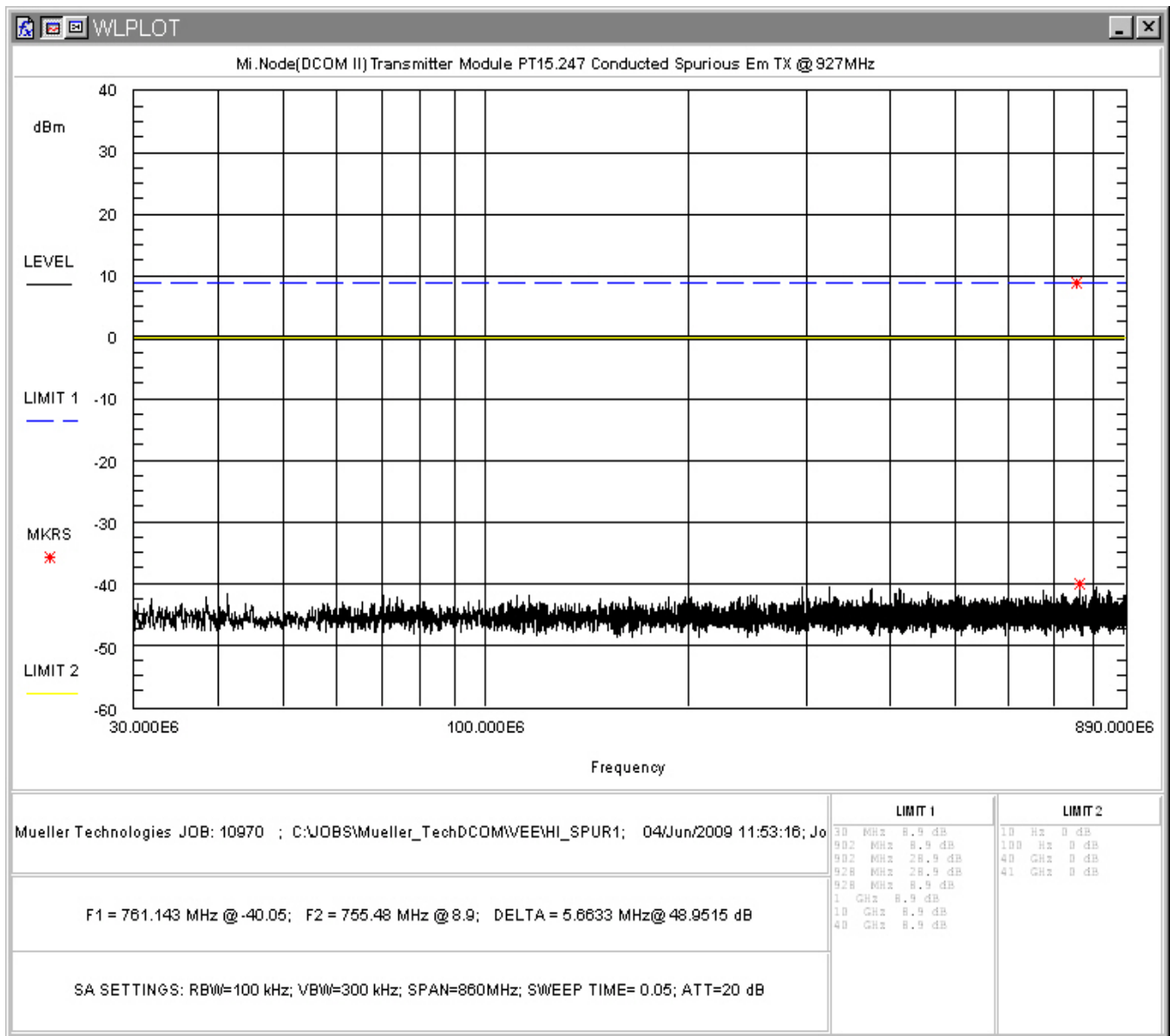
Figure 23: Conducted Spurious Emissions, High Channel 30 - 890MHz
