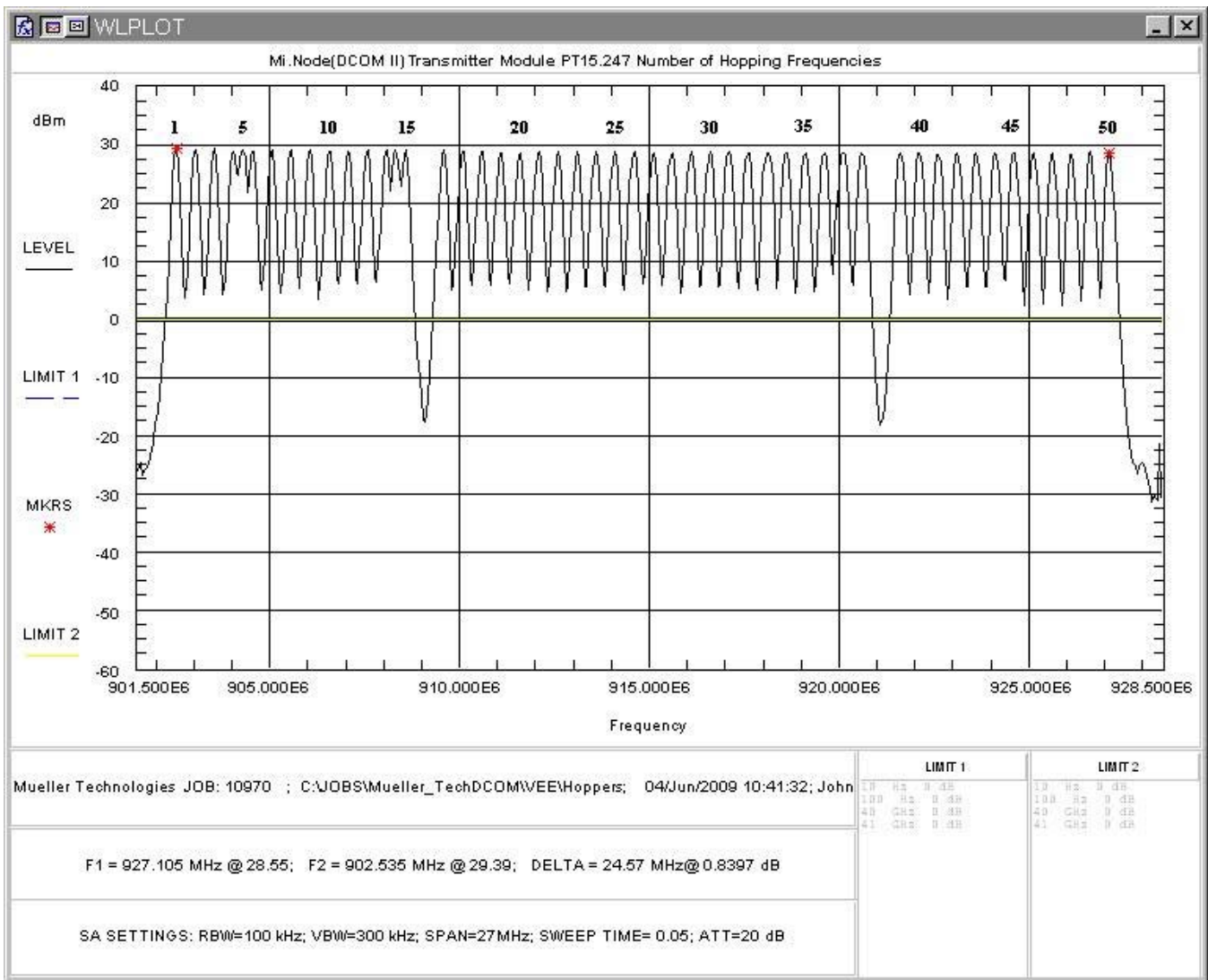
Figure 10: Number of Channels
