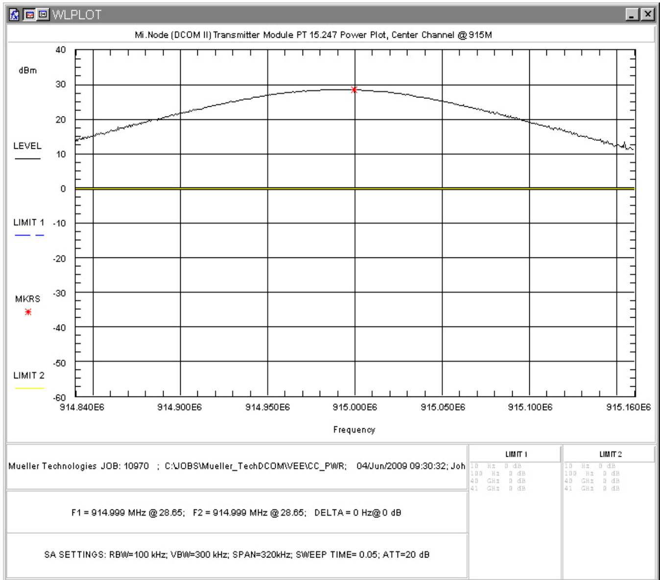
Figure 4: RF Peak Power, Mid Channel
