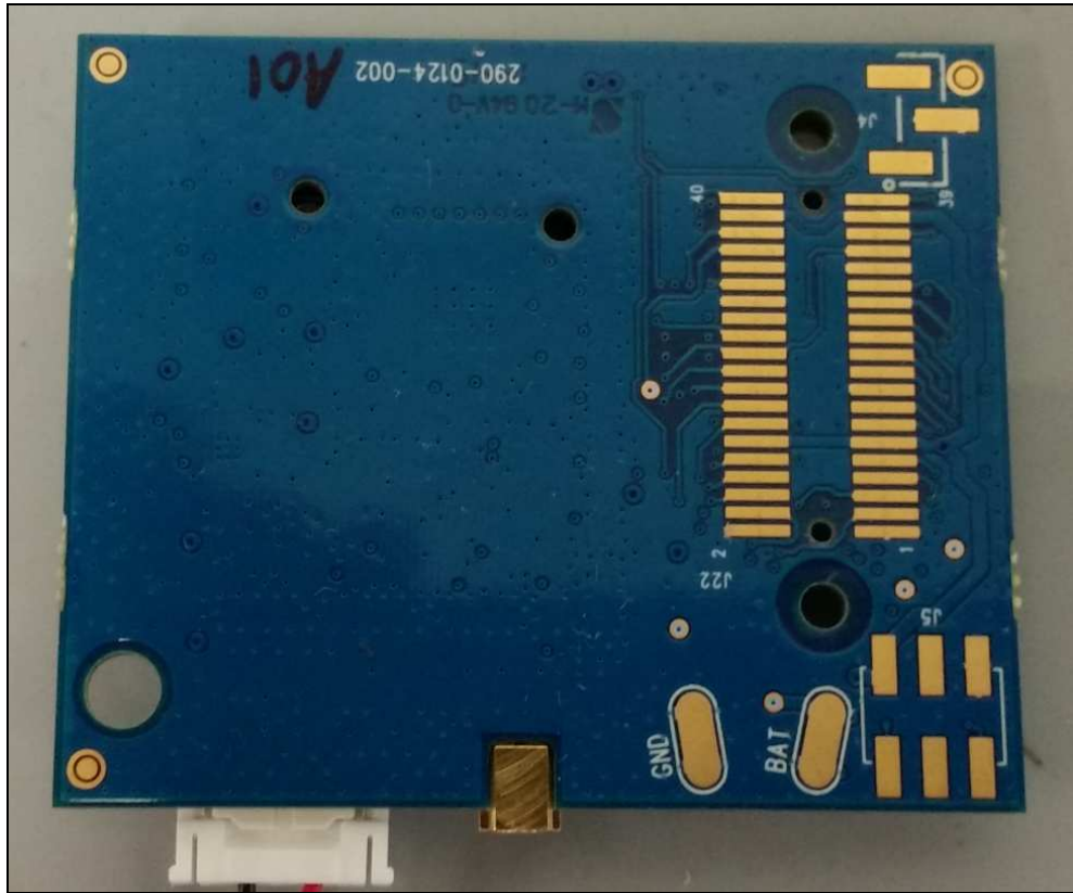
Figure 13: Internal Photo – LFM Bottom
