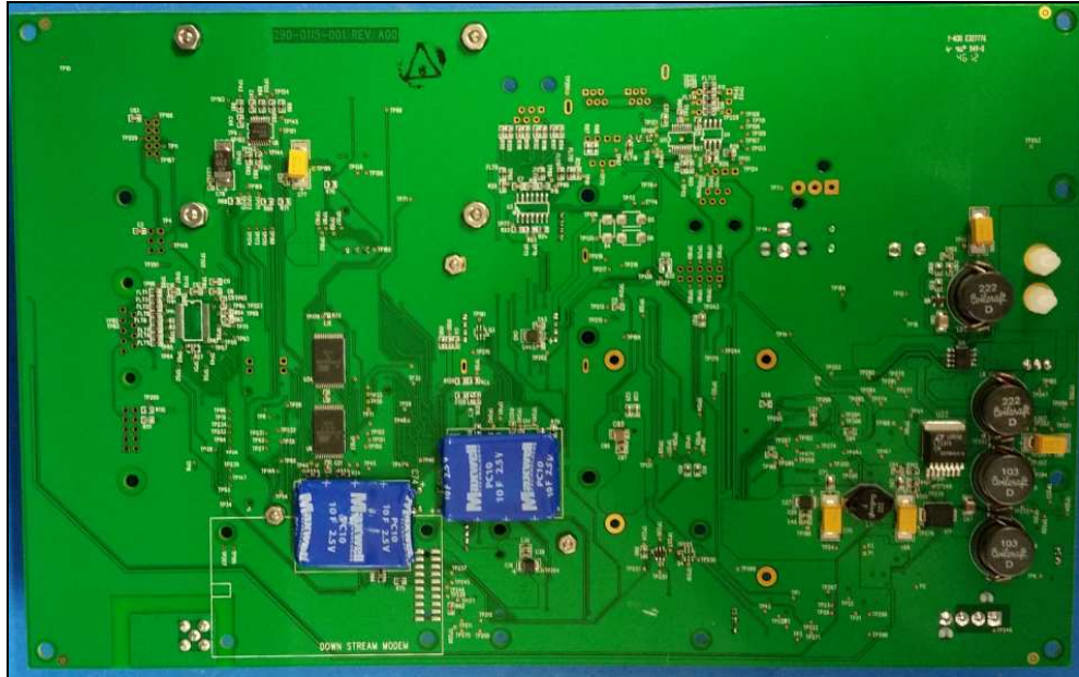
Figure 15: Internal Photo – Main Bottom
