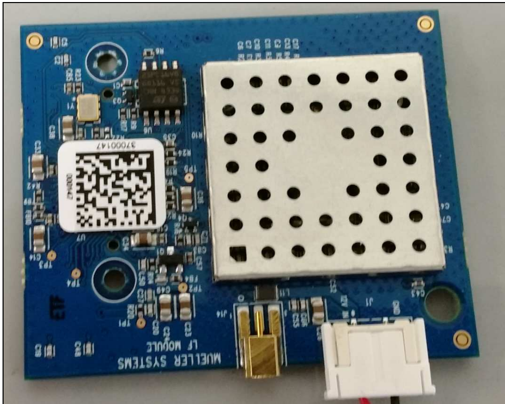
Figure 11: Internal Photo – LFM Top
