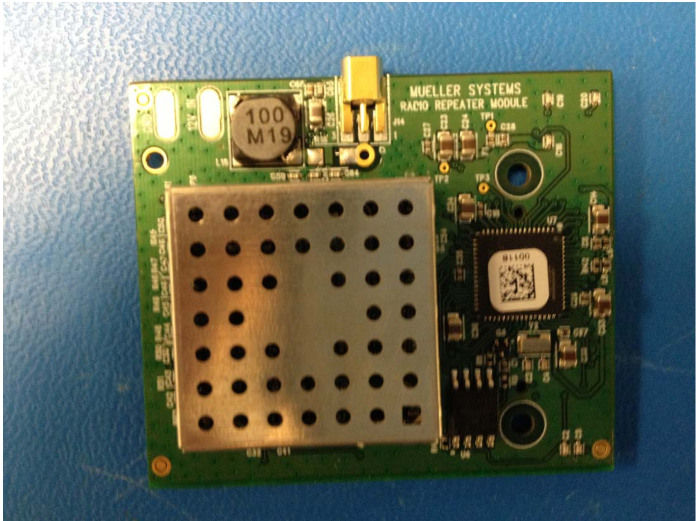
Figure 7 - Repeater Module top Side
