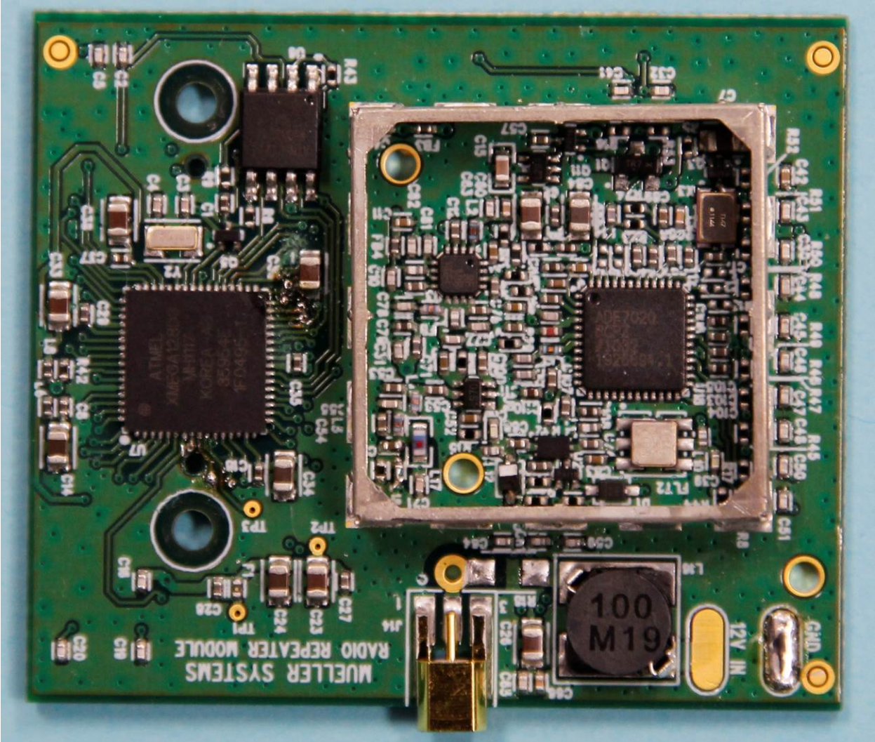
Figure 8- Repeater Module, No Shield
