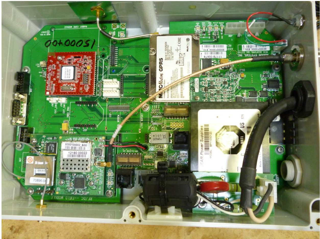
Figure 2 - MiHub 1.5 XR Main Board Top
