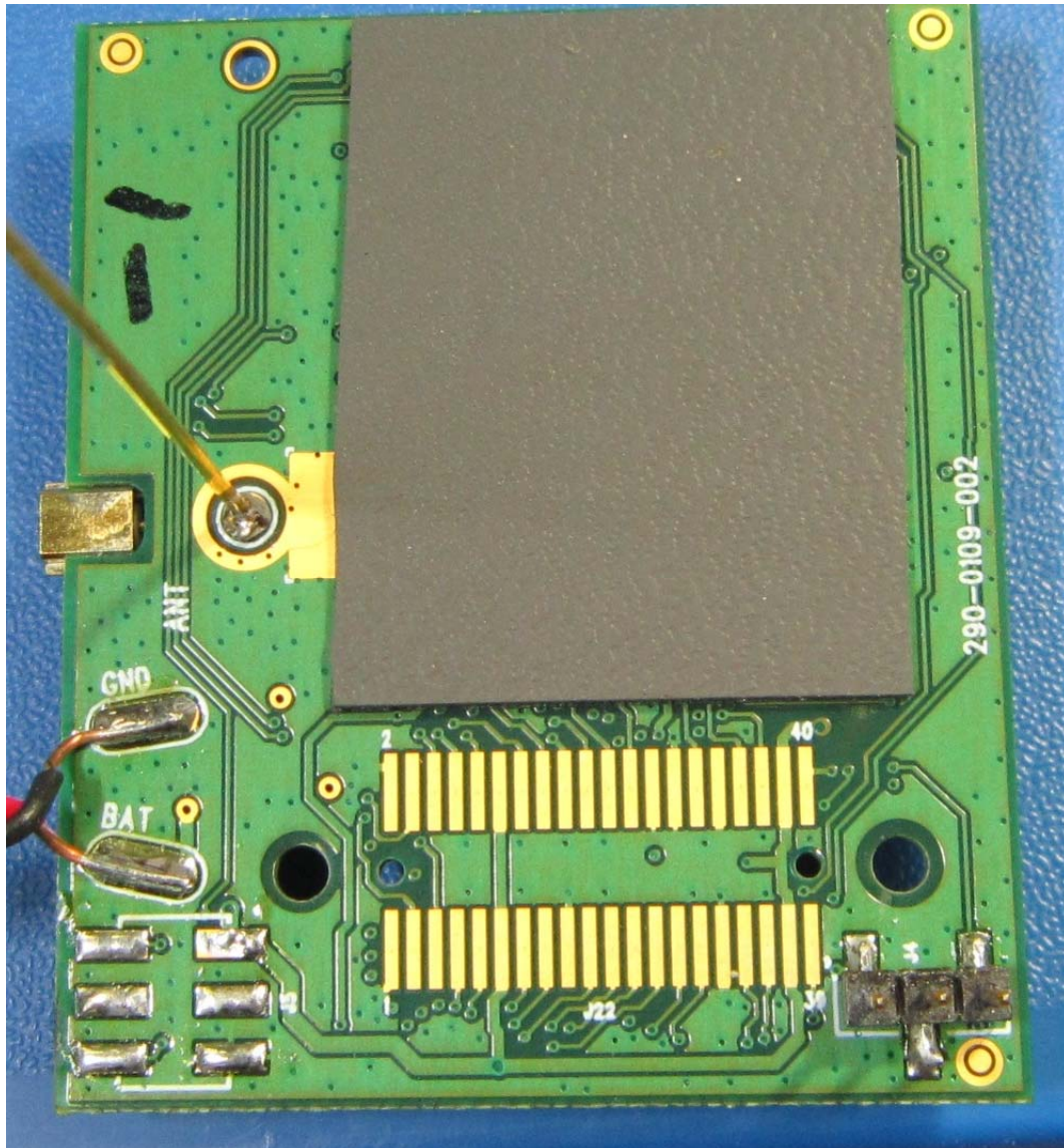
Figure 6 - Repeater module Bottom Side
