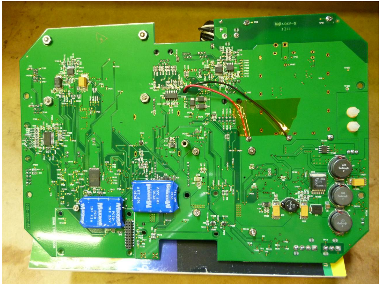
Figure 5- MiHub 1.5 XR Main Board Bottom Side
