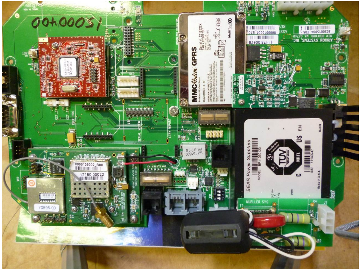
Figure 4 _ MiHub 1.5 XR Main board top side
