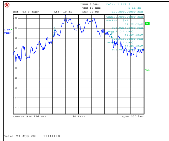
Figure 7.3.2-6: 99% Bandwidth Plot – 925MHz
