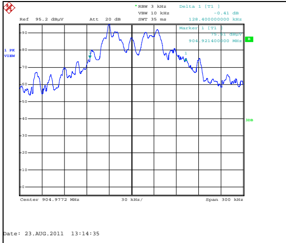
Figure 7.3.2-1: 20dB Bandwidth Plot – 905MHz
