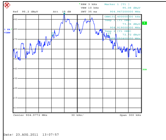
Figure 7.3.2-4: 99% Bandwidth Plot – 905MHz
