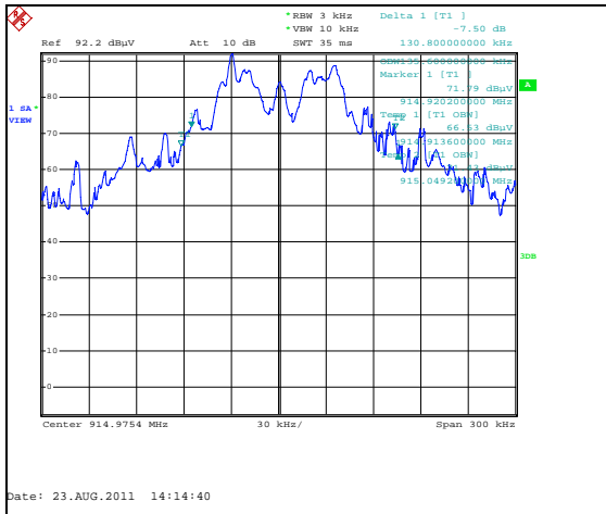
Figure 7.3.2-5: 99% Bandwidth Plot – 915MHz
