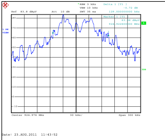
Figure 7.3.2-3: 20dB Bandwidth Plot – 925MHz
