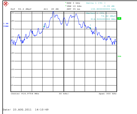
Figure 7.3.2-2: 20dB Bandwidth Plot – 915MHz
