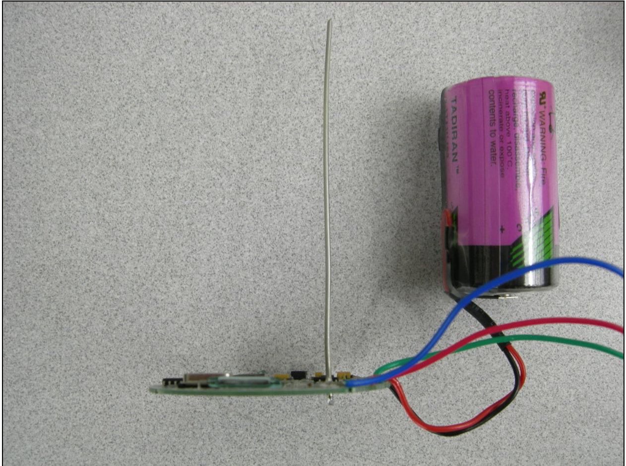
Figure 4: Internal Photo
