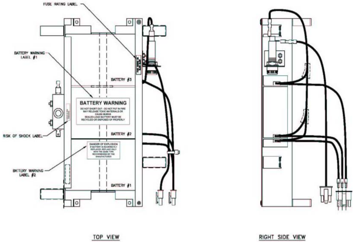
Battery Warning, ROS & Fuse Label locations on Battery Pack
