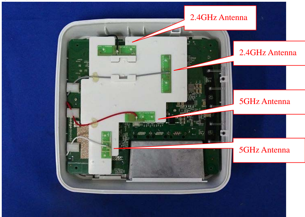
(7) EUT Photo
