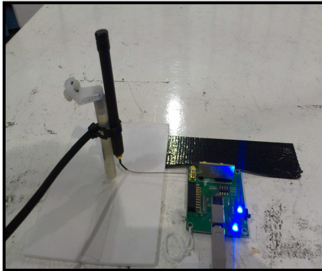
Photograph 2 - 3dBi Antenna
