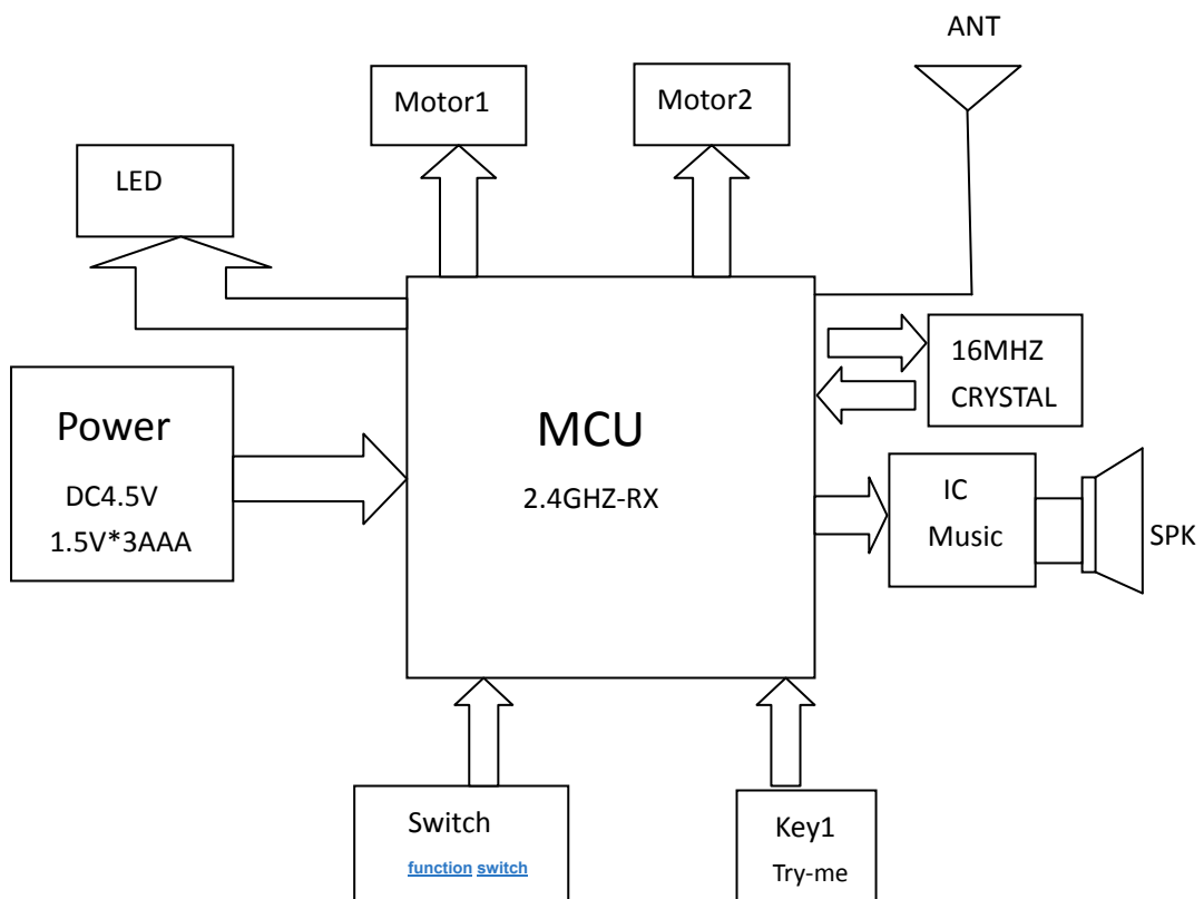
WH1330-WH1333RX ( block scheme )
