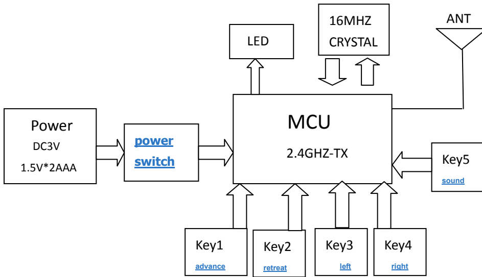
WH1132-WH1135TX ( block scheme )
