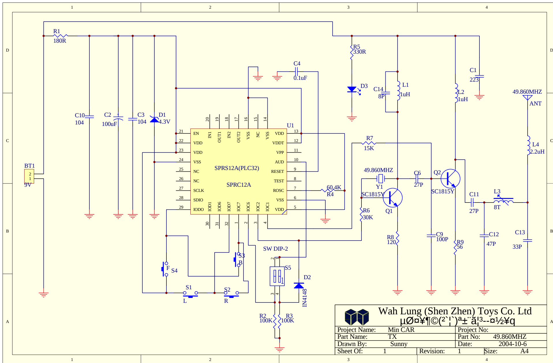
49.860MHz TX Schematic
