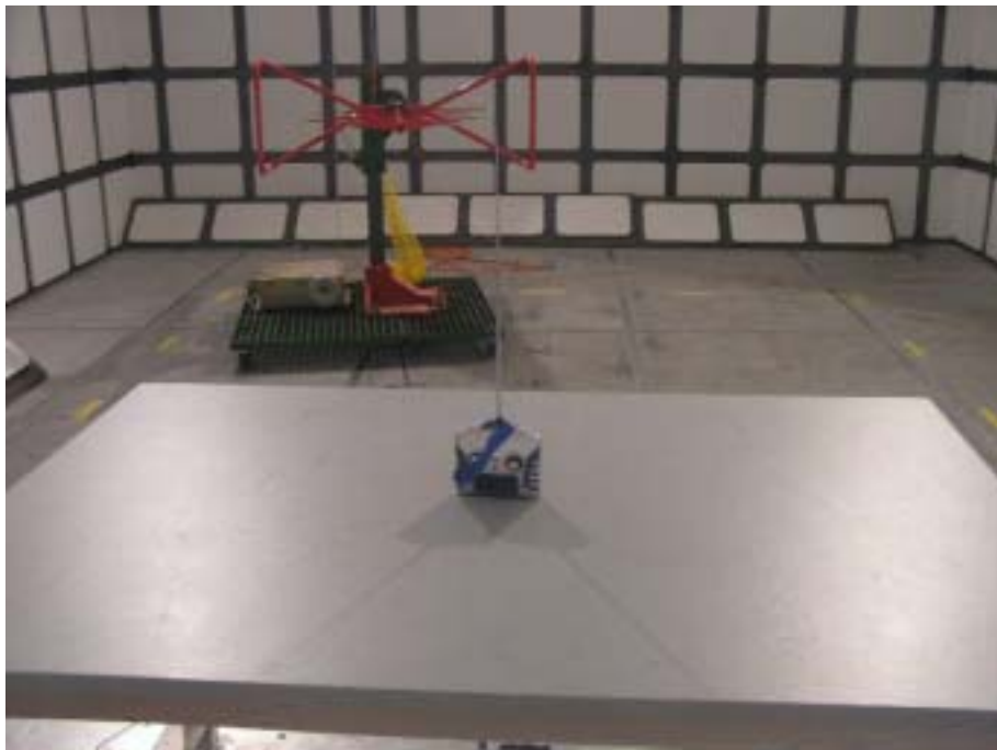
Radiated Emission-Stand View(30 MHz –1000 MHz)
