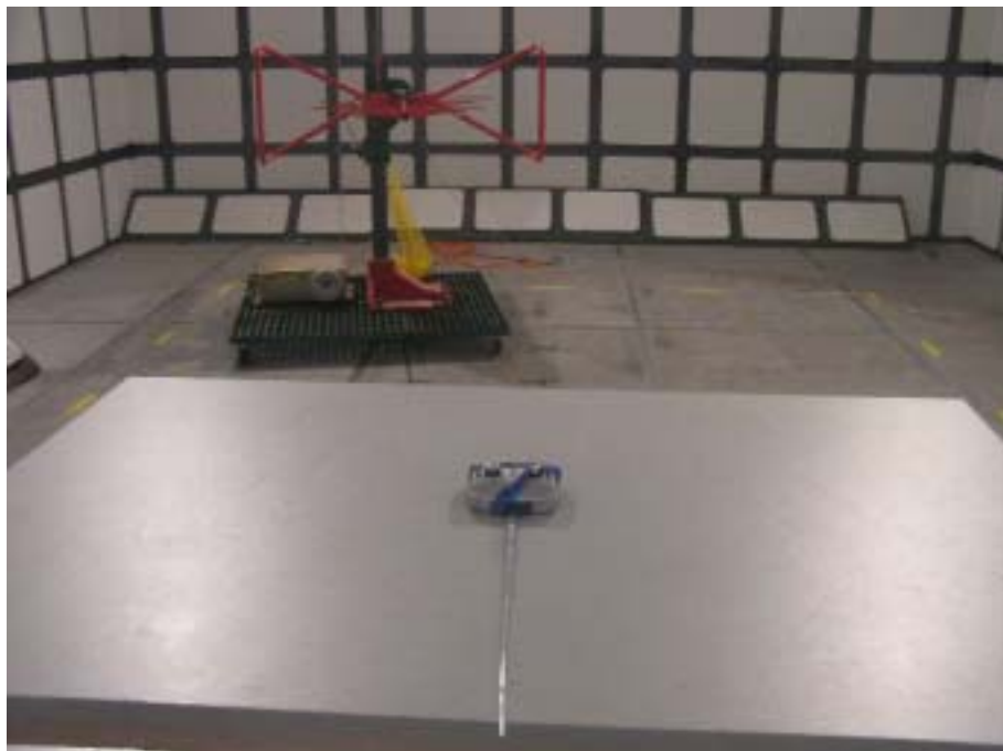
Radiated Emission-Lie View(30 MHz –1000 MHz)
