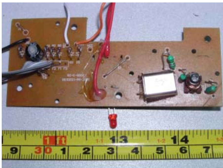
EUT – PCB2 Rear View
