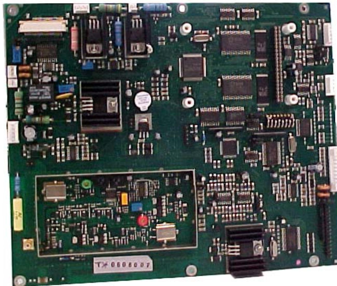
TX5000 CPU BOARD (Components side) All shields removed
