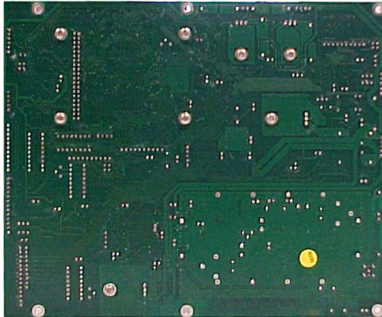
TX5000 CPU - Solder side
