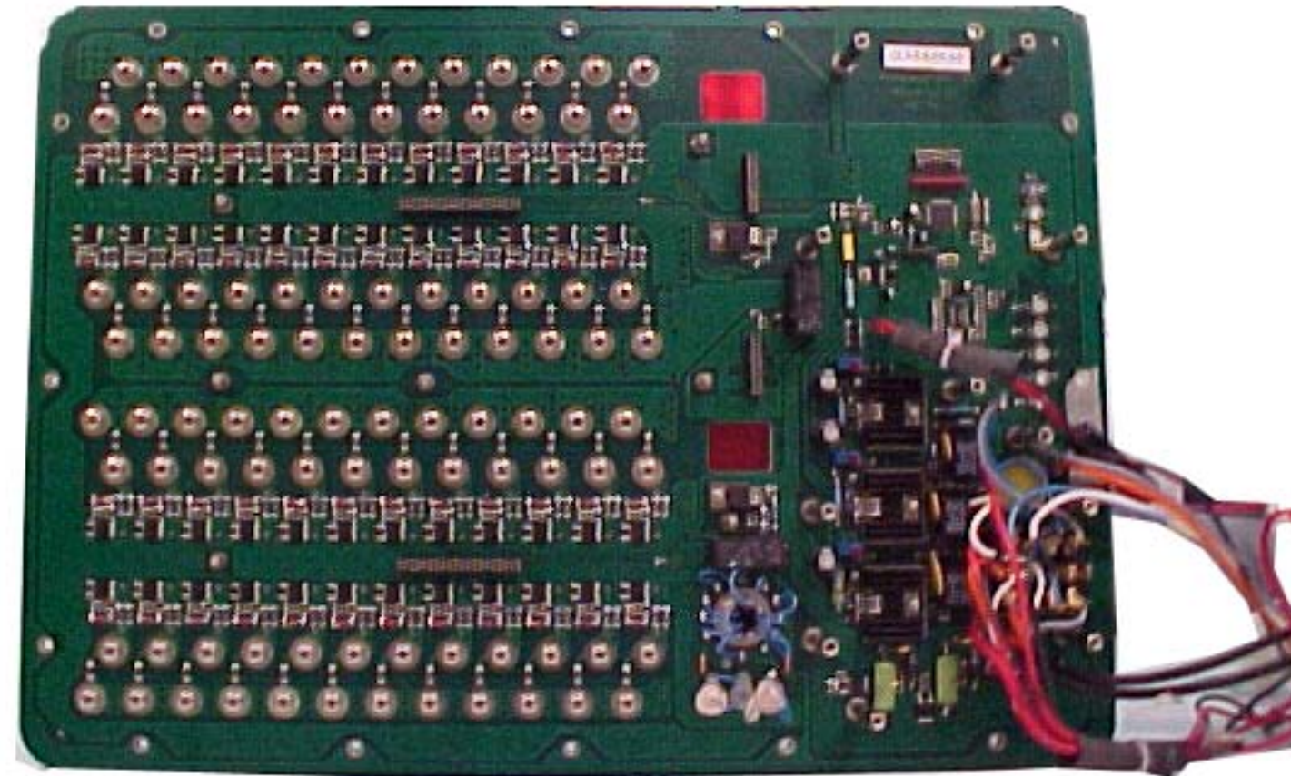
RX48-A MAIN BOARD (Components side) - All shields removed
