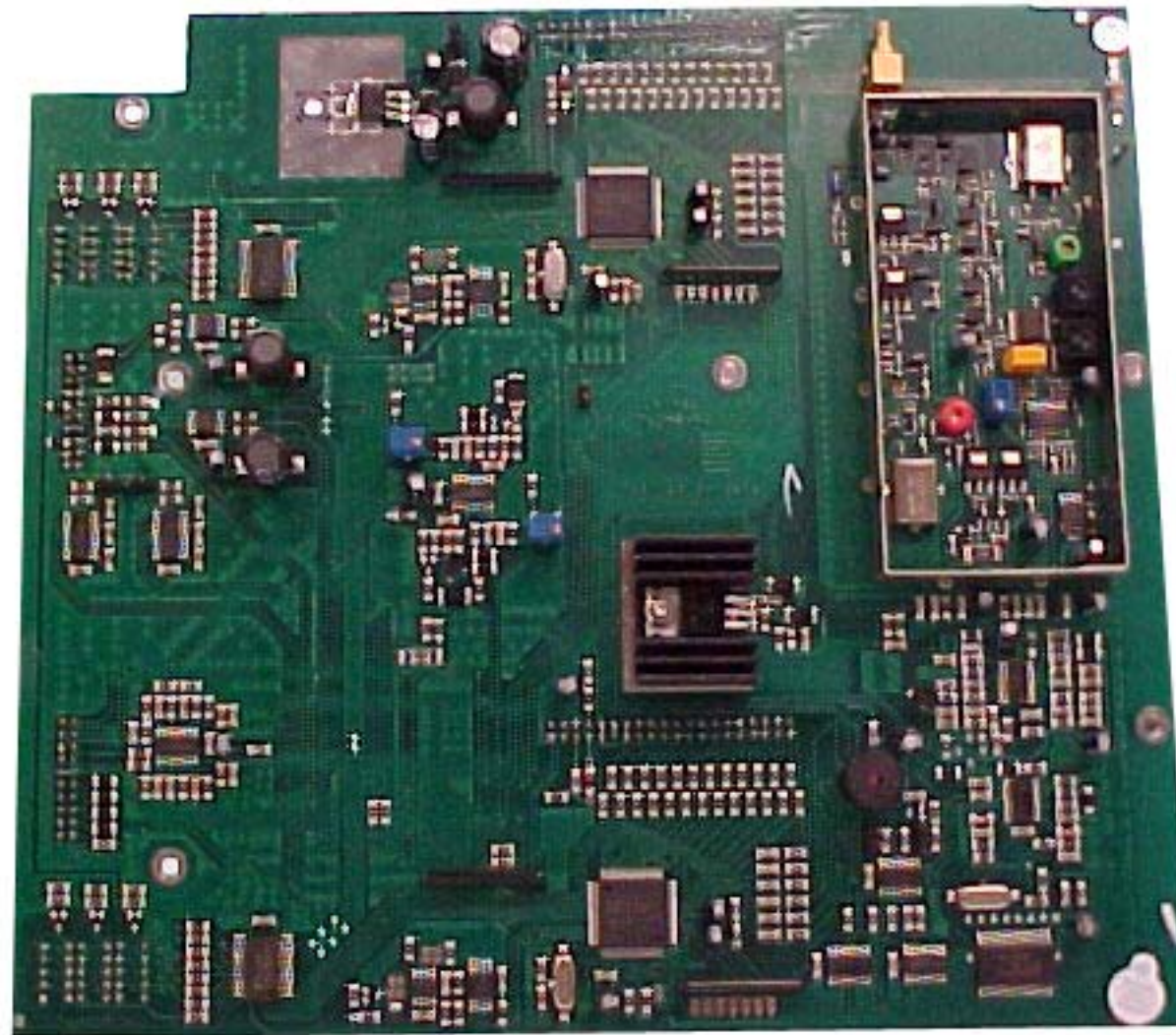
RX48-A CPU BOARD (Components side) All shields removed
