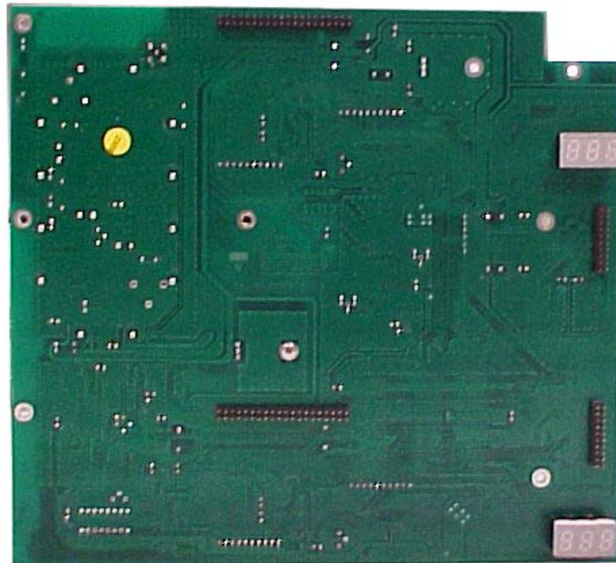
RX48-A CPU BOARD (solder side)
