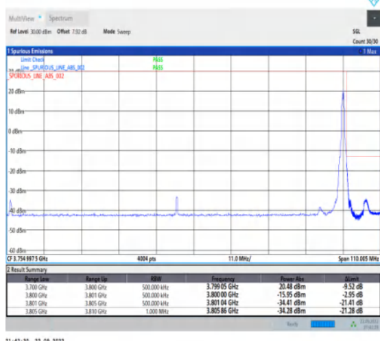
1-N78-3700-3800-30-100-H-5-CP-QPSK-Edge_1RB_Right-1@272-Ant1-1--PASS-see graph
