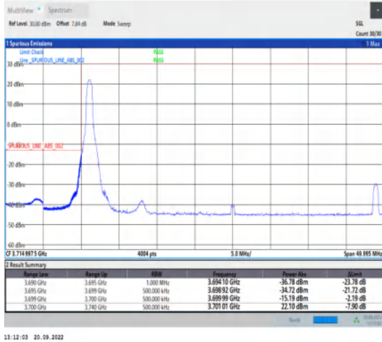
1-N78-3700-3800-30-40-L-1-DFT-PI2BPSK-Edge_1RB _Left-1@0-Ant1-1--PASS-see graph
