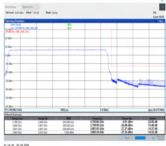
1-N78-3700-3800-30-20-H-6-CP-QPSK-Outer_Full-51@0-Ant1-1--PASS-see graph
