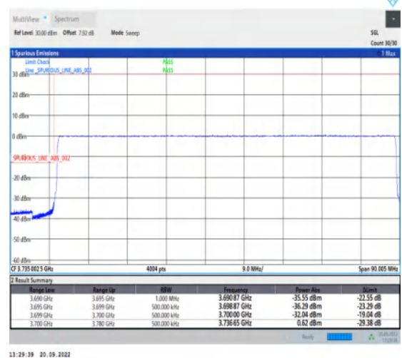
1-N78-3700-3800-30-80-L-6-CP-QPSK-Outer_Full -217@0-Ant1-1--PASS-see graph
