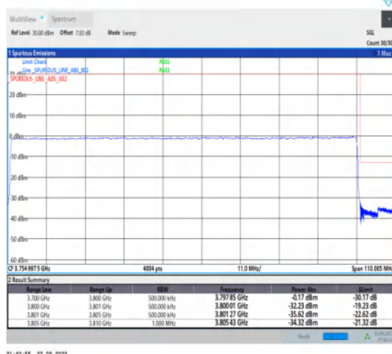
1-N78-3700-3800-30-100-H-6-CP-QPSK-Outer_Full-273@0-Ant1-1--PASS-see graph
