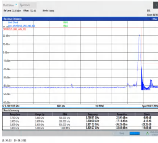
1-N78-3700-3800-30-80-H-2-DFT-PI2BPSK-Edge_1R B_Right-1@216-Ant1-1--PASS-see graph
