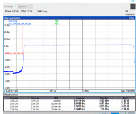
1-N78-3700-3800-30-60-L-6-CP-QPSK-Outer_Full_-162@0-Ant1-1--PASS-see graph
