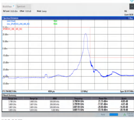
1-N78-3700-3800-PC2-30-20-H-5-CP-QPSK-Edge_1R B_Right-1@50-Ant1-1--PASS-see graph
