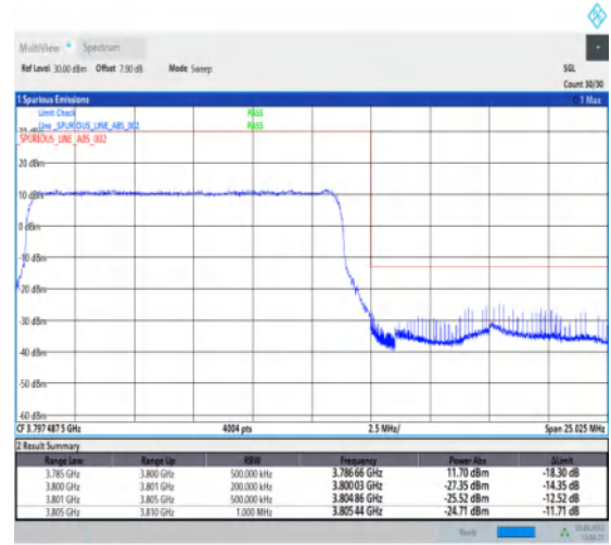
1-N78-3700-3800-30-15-H-3-DFT-PI2BPSK-Outer_Full-36@0-Ant1-1--PASS-see graph
