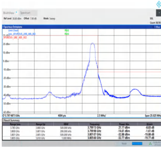
1-N78-3700-3800-30-15-H-2-DFT-PI2BPSK-Edge_1R_B_Right-1@37-Ant1-1--PASS-see graph
