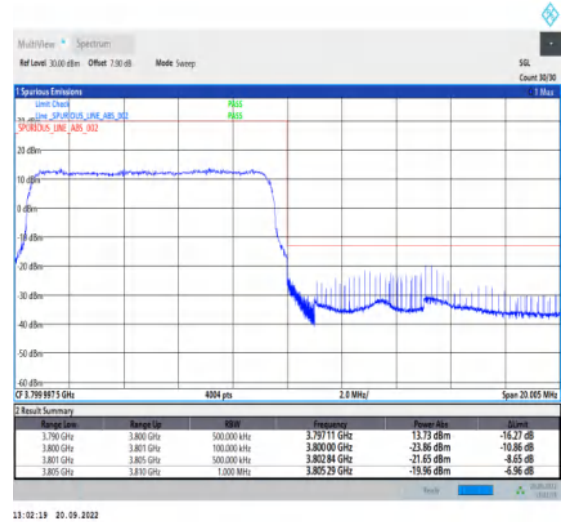
1-N78-3700-3800-30-10-H-3-DFT-PI2BPSK-Outer_Full-24@0-Ant1-1--PASS-see graph
