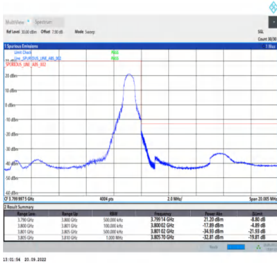
1-N78-3700-3800-30-10-H-2-DFT-PI2BPSK-Edge_1R_B_Right-1@23-Ant1-1--PASS-see graph
