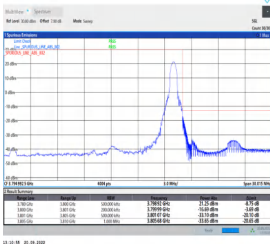
1-N78-3700-3800-30-20-H-5-CP-QPSK-Edge_1RB_Right-1@50-Ant1-1--PASS-see graph
