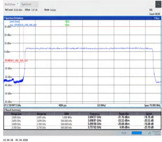
1-N78-3700-3800-30-70-L-3-DFT-PI2BPSK-Outer _Full-180@0-Ant1-1--PASS-see graph
