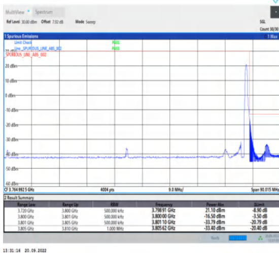
1-N78-3700-3800-30-80-H-5-CP-QPSK-Edge_1RB_Ri ght-1@216-Ant1-1--PASS-see graph
