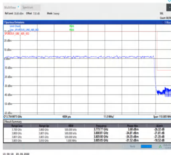
1-N78-3700-3800-30-100-H-3-DFT-PI2BPSK-Outer_Full-270@0-Ant1-1--PASS-see graph
