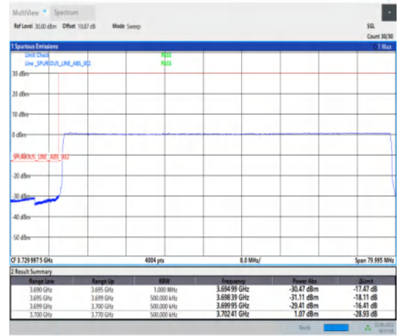
1-N78-3700-3800-PC2-30-70-L-6-CP-QPSK-Outer _Full-189@0-Ant1-1--PASS-see graph
