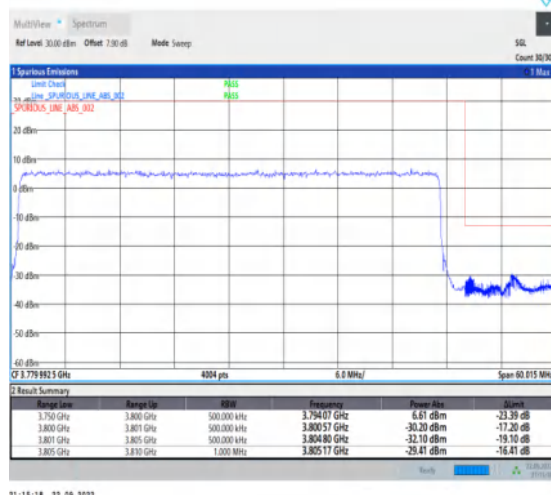
1-N78-3700-3800-30-50-H-3-DFT-PI2BPSK-Outer _Full-128@0-Ant1-1--PASS-see graph
