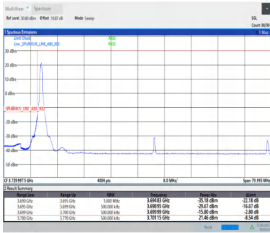
1-N78-3700-3800-PC2-30-70-L-4-CP-QPSK-Edge_1R B_Left-1@0-Ant1-1--PASS-see graph
