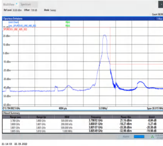
1-N78-3700-3800-30-20-H-2-DFT-PI2BPSK-Edge_1R_B_Right-1@50-Ant1-1--PASS-see graph
