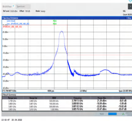
1-N78-3700-3800-30-10-H-5-CP-QPSK-Edge_1RB_Right-1@23-Ant1-1--PASS-see graph
