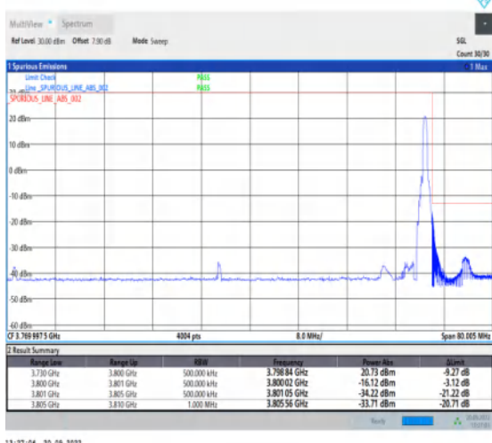
1-N78-3700-3800-30-70-H-5-CP-QPSK-Edge_1RB_Ri ght-1@188-Ant1-1--PASS-see graph
