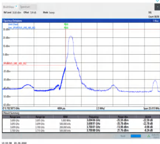
1-N78-3700-3800-30-15-L-1-DFT-PI2BPSK-Edge_1RB_Left-1@0-Ant1-1--PASS-see graph
