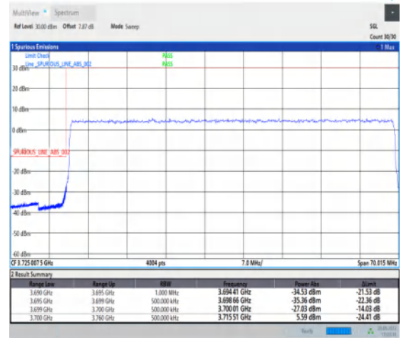
1-N78-3700-3800-30-60-L-3-DFT-PI2BPSK-Outer_Full-162@0-Ant1-1--PASS-see graph
