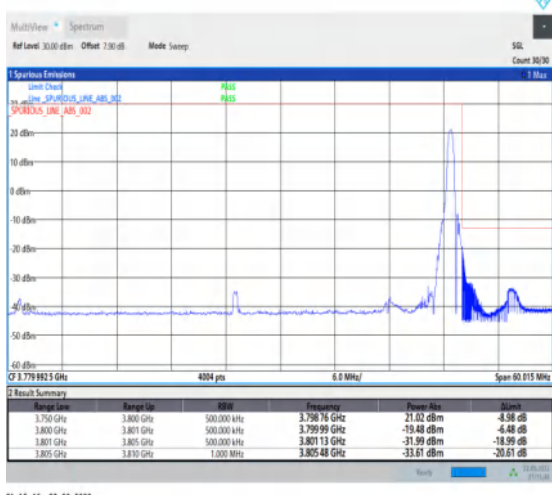
1-N78-3700-3800-30-50-H-5-CP-QPSK-Edge_1RB_Ri ght-1@132-Ant1-1--PASS-see graph
