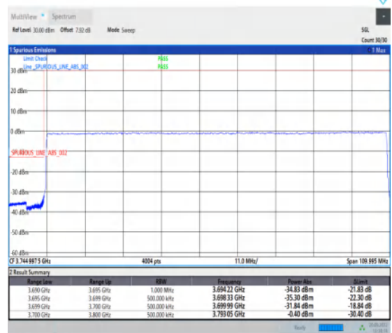
1-N78-3700-3800-30-100-L-6-CP-QPSK-Outer_Full-273@0-Ant1-1--PASS-see graph
