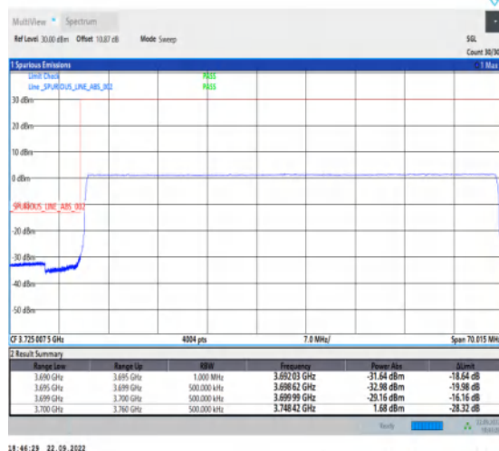
1-N78-3700-3800-PC2-30-60-L-6-CP-QPSK-Outer _Full-162@0-Ant1-1--PASS-see graph
