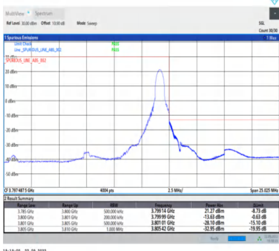
1-N78-3700-3800-PC2-30-15-H-5-CP-QPSK-Edge_1R B_Right-1@37-Ant1-1--PASS-see graph
