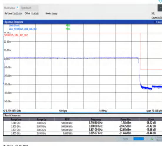
1-N78-3700-3800-PC2-30-60-H-6-CP-QPSK-Outer _Full-162@0-Ant1-1--PASS-see graph
