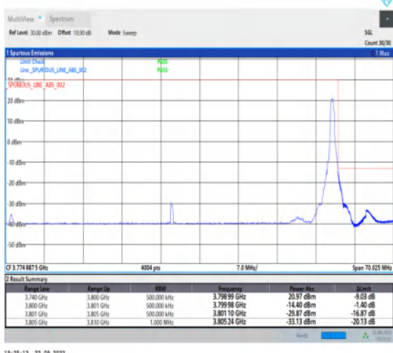
1-N78-3700-3800-PC2-30-60-H-5-CP-QPSK-Edge_1R B_Right-1@161-Ant1-1--PASS-see graph
