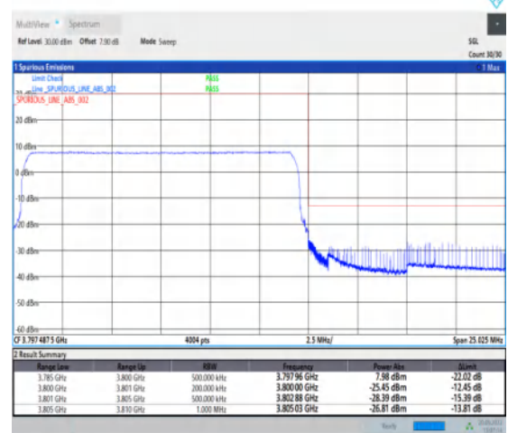
1-N78-3700-3800-30-15-H-6-CP-QPSK-Outer_Full-38@0-Ant1-1--PASS-see graph
