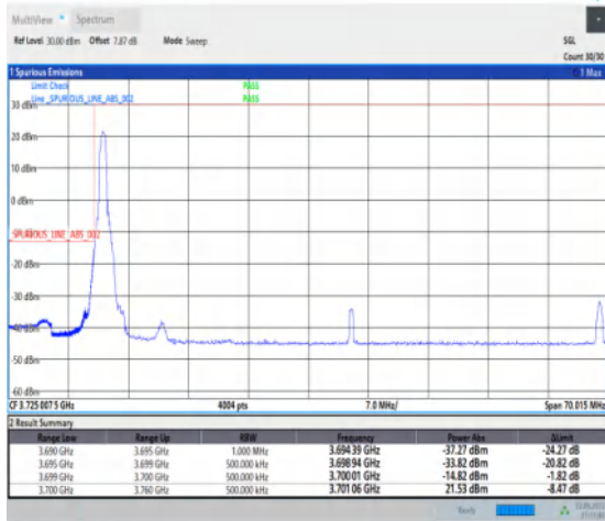
1-N78-3700-3800-30-60-L-1-DFT-PI2BPSK-Edge_1RB_Left-1@0-Ant1-1--PASS-see graph
