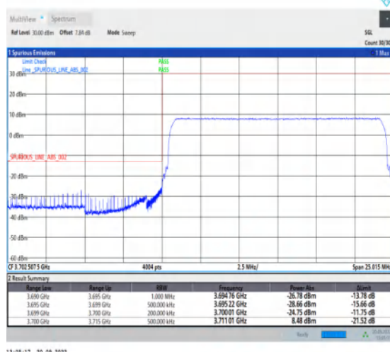
1-N78-3700-3800-30-15-L-6-CP-QPSK-Outer_Full -38@0-Ant1-1--PASS-see graph
