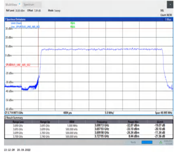
1-N78-3700-3800-30-40-L-3-DFT-PI2BPSK-Outer _Full-100@0-Ant1-1--PASS-see graph
