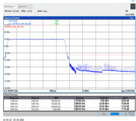
1-N78-3700-3800-30-10-H-6-CP-QPSK-Outer_Full-24@0-Ant1-1--PASS-see graph
