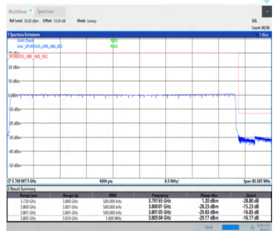
1-N78-3700-3800-PC2-30-70-H-6-CP-QPSK-Outer _Full-189@0-Ant1-1--PASS-see graph
