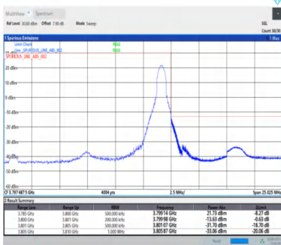
1-N78-3700-3800-30-15-H-5-CP-QPSK-Edge_1RB_Right-1@37-Ant1-1--PASS-see graph
