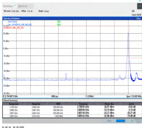
1-N78-3700-3800-30-100-H-2-DFT-PI2BPSK-Edge_1R_B_Right-1@272-Ant1-1--PASS-see graph
