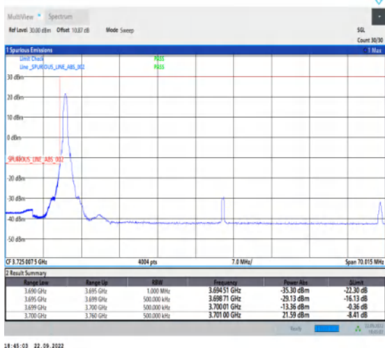
1-N78-3700-3800-PC2-30-60-L-4-CP-QPSK-Edge_1R B_Left-1@0-Ant1-1--PASS-see graph
