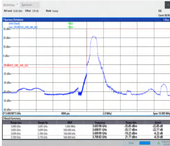
1-N78-3700-3800-30-10-L-1-DFT-PI2BPSK-Edge_1RB _Left-1@0-Ant1-1--PASS-see graph
