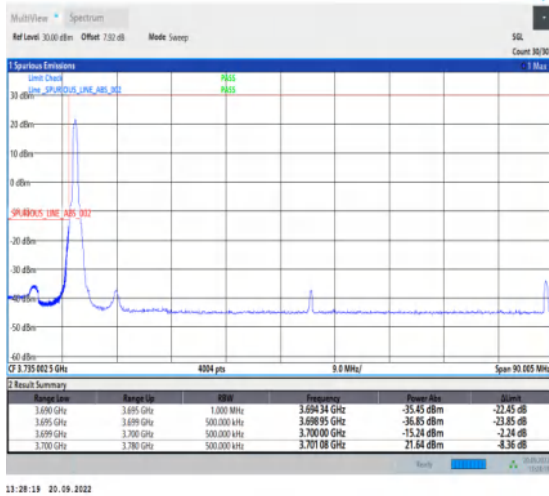
1-N78-3700-3800-30-80-L-1-DFT-PI2BPSK-Edge_1RB_Left-1@0-Ant1-1--PASS-see graph
