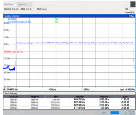
1-N78-3700-3800-30-100-L-3-DFT-PI2BPSK-Outer_Full-270@0-Ant1-1--PASS-see graph
