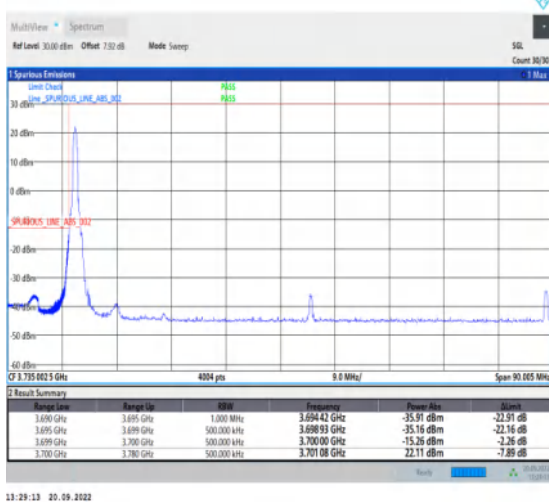
1-N78-3700-3800-30-80-L-4-CP-QPSK-Edge_1RB_Lef t-1@0-Ant1-1--PASS-see graph
