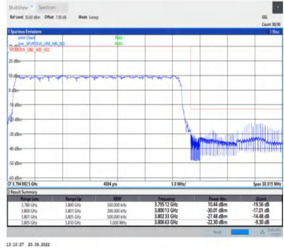
1-N78-3700-3800-30-20-H-3-DFT-PI2BPSK-Outer_Full-50@0-Ant1-1--PASS-see graph
