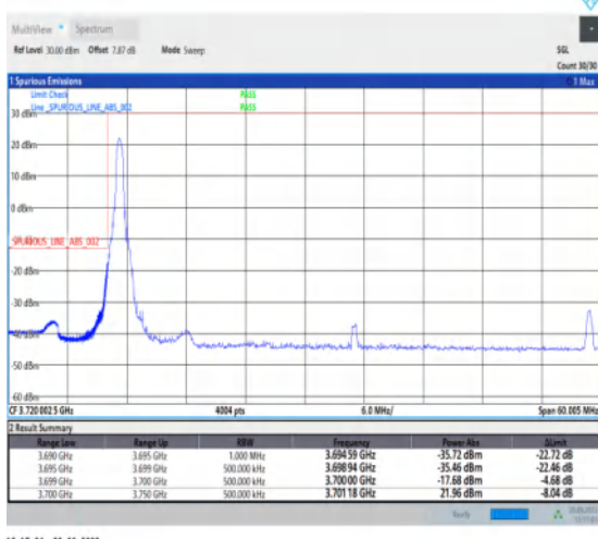
1-N78-3700-3800-30-50-L-4-CP-QPSK-Edge_1RB_Lef t-1@0-Ant1-1--PASS-see graph
